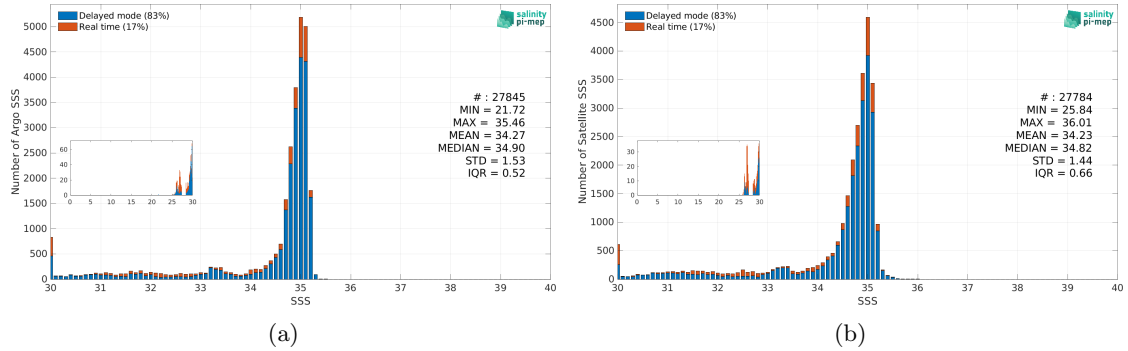
Figure 3: Histograms of SSS from Argo (a) and SMOS SSS L4 v1 - Daily (CMEMS-CNR) (b) considering all match-up pairs per bins of 0.1 over the Arctic Ocean Pi-MEP region and for the full satellite product period.
