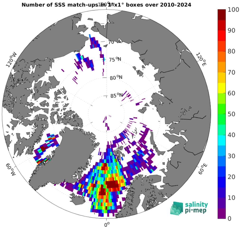
Figure 5: Number of SSS match-ups between Argo SSS and the SMOS SSS L4 v1 - Daily (CMEMS-CNR) SSS product for the Arctic Ocean Pi-MEP region over 1^\circ \times 1^\circ boxes and for the full satellite product period.
