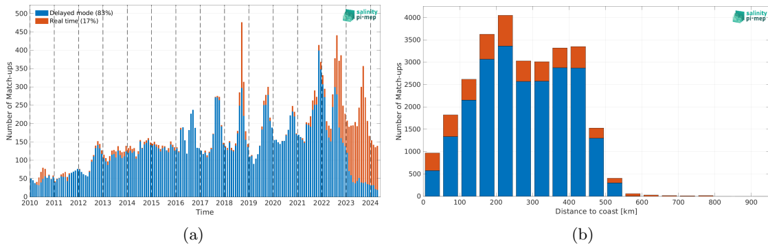
Figure 2: Number of match-ups between Argo and SMOS SSS L4 v1 - Daily (CMEMS-CNR) SSS as a function of time (a) and as function of the distance to coast (b) over the Arctic Ocean Pi-MEP region and for the full satellite product period.
