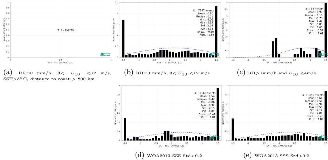
Figure 15: Normalized histogram of \Delta\text{SSS} (SMOS SSS L4 OI v346 - Weekly (CMEMS-CATDS-LOPS) - TSG (SAMOS)) for 5 different subdatasets corresponding to: RR=0 mm/h, 3 < U_{10} < 12 m/s, SST>5°C, distance to coast > 800 km (a), RR=0 mm/h, 3 < U_{10} < 12 m/s (b), RR>1mm/h and U_{10} < 4 m/s (c), WOA2013 SSS Std<0.2 (d), WOA2013 SSS Std>0.2 (e).
