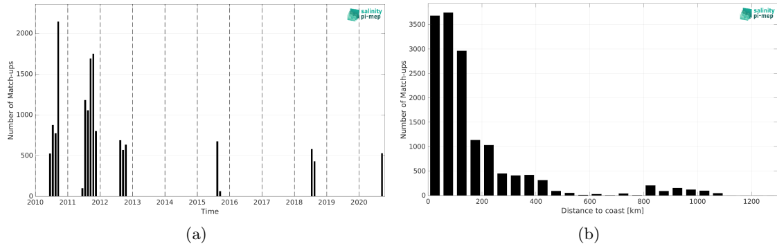
Figure 2: Number of match-ups between TSG (SAMOS) and SMOS SSS L4 OI v346 - Weekly (CMEMS-CATDS-LOPS) SSS as a function of time (a) and as function of the distance to coast (b) over the Arctic Ocean Pi-MEP region and for the full satellite product period.
