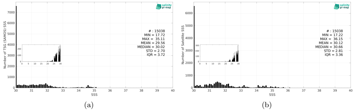
Figure 3: Histograms of SSS from TSG (SAMOS) (a) and SMOS SSS L4 OI v346 - Weekly (CMEMS-CATDS-LOPS) (b) considering all match-up pairs per bins of 0.1 over the Arctic Ocean Pi-MEP region and for the full satellite product period.
