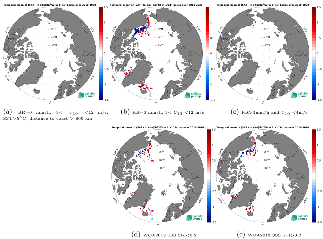
Figure 14: Temporal mean gridded over spatial boxes of size 1^\circ \times 1^\circ of \Delta\text{SSS} (SMOS SSS L4 OI v346 - Weekly (CMEMS-CATDS-LOPS) - TSG (SAMOS)) for 5 different subdatasets corresponding to:RR=0 mm/h, 3 < U_{10} < 12 m/s, SST > 5°C, distance to coast > 800 km (a), RR=0 mm/h, 3 < U_{10} < 12 m/s (b), RR > 1mm/h and U_{10} < 4 m/s (c), WOA2013 SSS Std < 0.2 (d), WOA2013 SSS Std > 0.2 (e).
