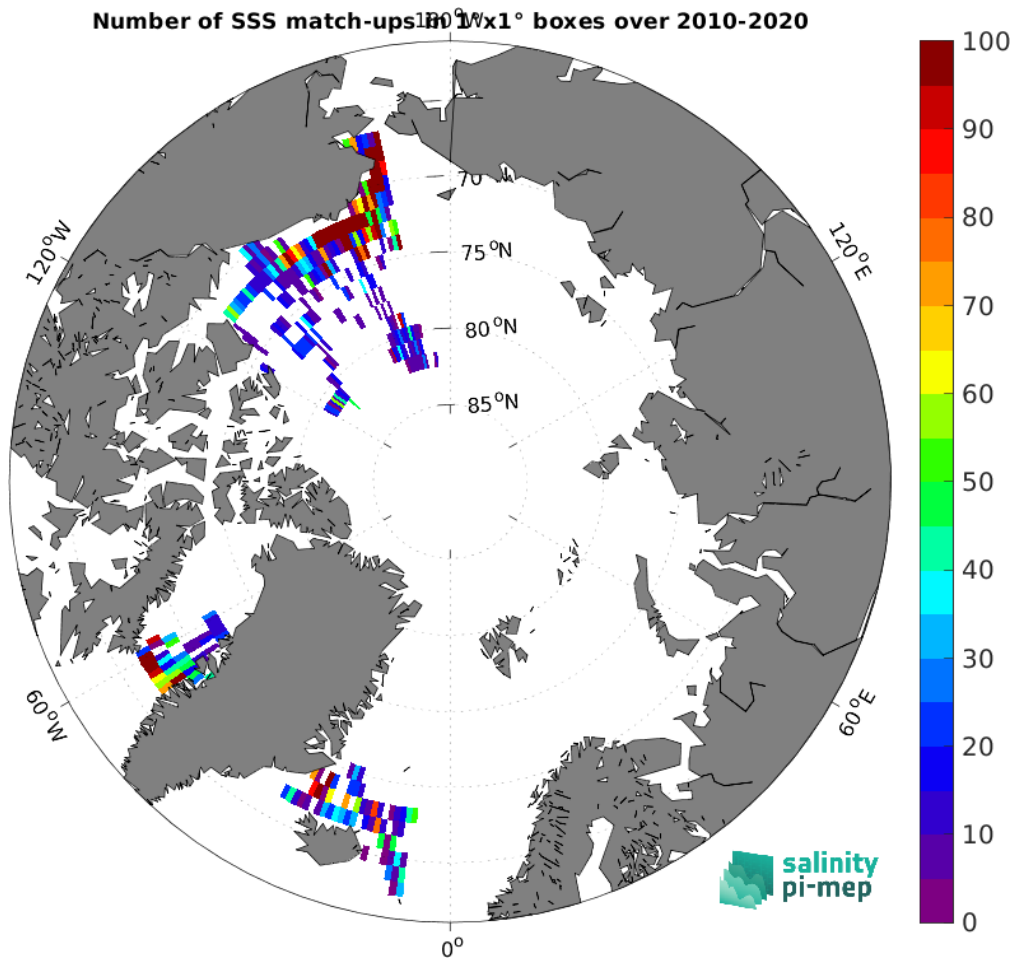
Figure 5: Number of SSS match-ups between TSG (SAMOS) SSS and the SMOS SSS L4 OI v346 - Weekly (CMEMS-CATDS-LOPS) SSS product for the Arctic Ocean Pi-MEP region over 1^\circ \times 1^\circ boxes and for the full satellite product period.
