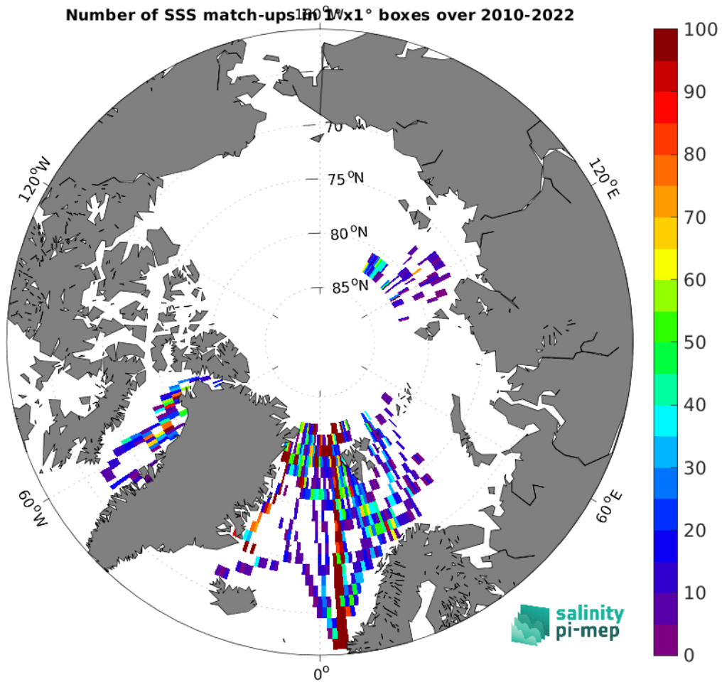
Figure 5: Number of SSS match-ups between TSG (Polarstern) SSS and the SMOS SSS L4 OI v346 - Weekly (CMEMS-CATDS-LOPS) SSS product for the Arctic Ocean Pi-MEP region over 1^\circ \times 1^\circ boxes and for the full satellite product period.
