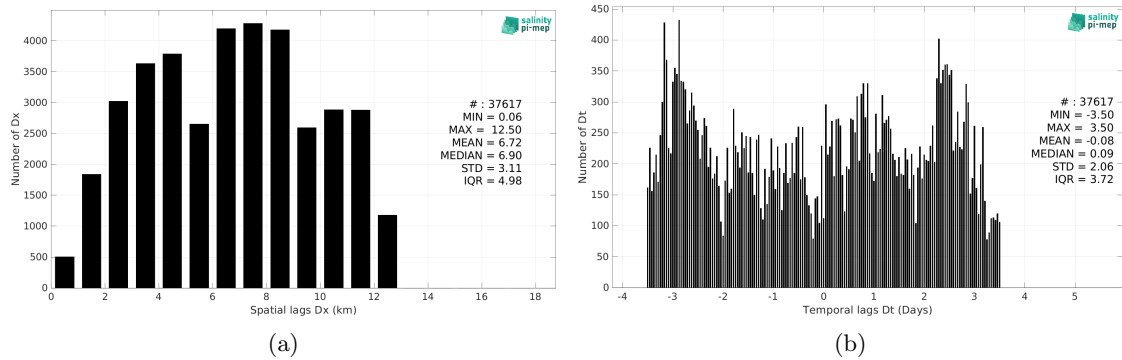
Figure 6: Histograms of the spatial (a) and temporal (b) lags between the location/time of the TSG (Polarstern) measurement and the date of the corresponding SMOS SSS L4 OI v346 - Weekly (CMEMS-CATDS-LOPS) SSS pixel.
