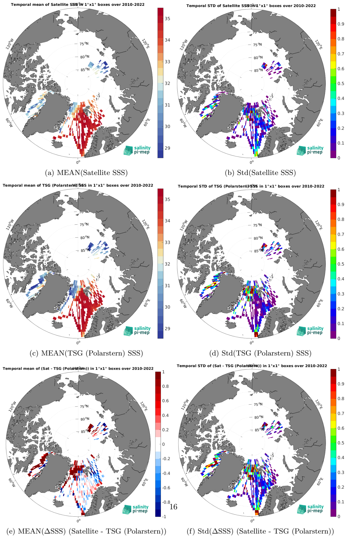
Figure 7: Temporal mean (left) and Std (right) of SSS from SMOS SSS L4 OI v346 - Weekly (CMEMS-CATDS-LOPS) (top), TSG (Polarstern) (middle), and of \Delta SSS (Satellite - TSG (Polarstern)). Only match-up pairs are used to generate these maps.
