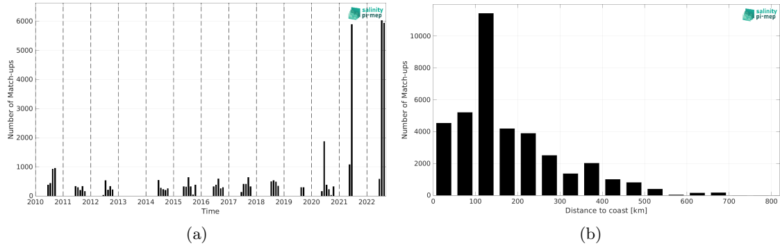
Figure 2: Number of match-ups between TSG (Polarstern) and SMOS SSS L4 OI v346 - Weekly (CMEMS-CATDS-LOPS) SSS as a function of time (a) and as function of the distance to coast (b) over the Arctic Ocean Pi-MEP region and for the full satellite product period.
