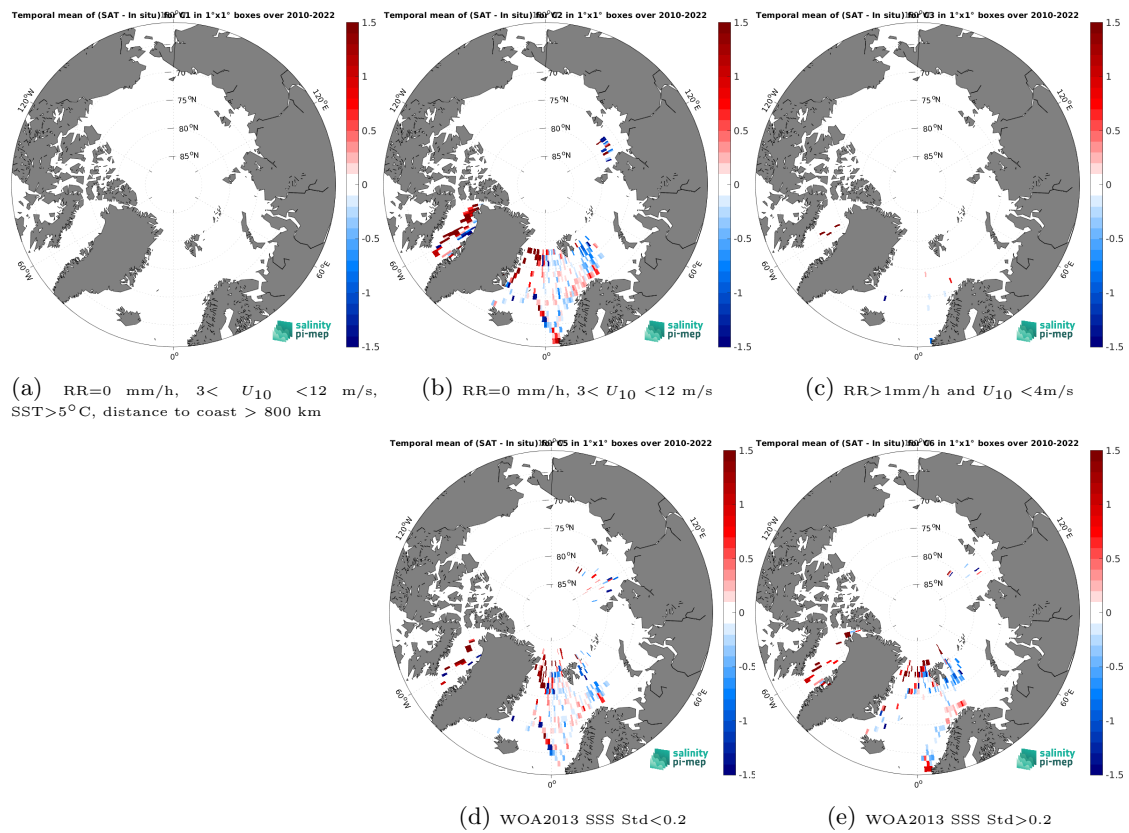
Figure 14: Temporal mean gridded over spatial boxes of size 1^\circ \times 1^\circ of \Delta SSS (SMOS SSS L4 OI v346 - Weekly (CMEMS-CATDS-LOPS) - TSG (Polarstern)) for 5 different subdatasets corresponding to:RR=0 mm/h, 3 < U_{10} < 12 m/s, SST >5^\circ\text{C} , distance to coast > 800 km (a), RR=0 mm/h, 3 < U_{10} < 12 m/s (b), RR >1 mm/h and U_{10} < 4 m/s (c), WOA2013 SSS Std <0.2 (d), WOA2013 SSS Std >0.2 (e).
