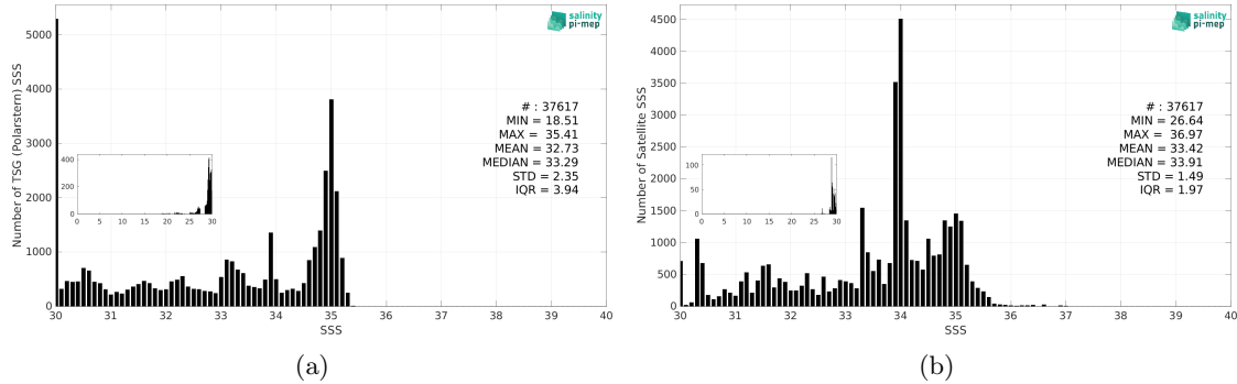
Figure 3: Histograms of SSS from TSG (Polarstern) (a) and SMOS SSS L4 OI v346 - Weekly (CMEMS-CATDS-LOPS) (b) considering all match-up pairs per bins of 0.1 over the Arctic Ocean Pi-MEP region and for the full satellite product period.
