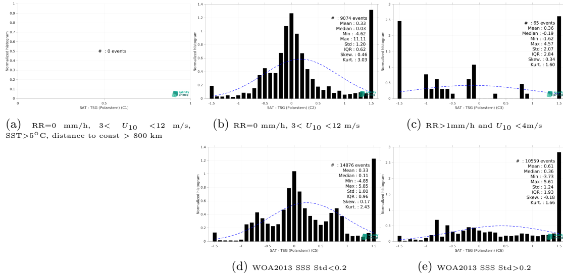
Figure 15: Normalized histogram of \Delta SSS (SMOS SSS L4 OI v346 - Weekly (CMEMS-CATDS-LOPS) - TSG (Polarstern)) for 5 different subdatasets corresponding to: RR=0 mm/h, 3 < U_{10} < 12 m/s, SST > 5°C, distance to coast > 800 km (a), RR=0 mm/h, 3 < U_{10} < 12 m/s (b), RR > 1mm/h and U_{10} < 4 m/s (c), WOA2013 SSS Std < 0.2 (d), WOA2013 SSS Std > 0.2 (e).
