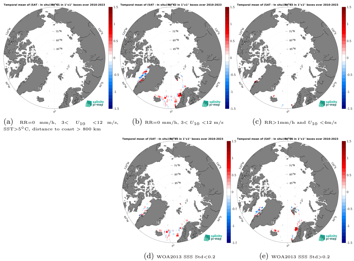
Figure 14: Temporal mean gridded over spatial boxes of size 1^\circ \times 1^\circ of \Delta\text{SSS} (SMOS SSS L4 OI v346 - Weekly (CMEMS-CATDS-LOPS) - TSG (LEGOS-DM)) for 5 different subdatasets corresponding to:RR=0 mm/h, 3 < U_{10} < 12 m/s, SST>5°C, distance to coast > 800 km (a), RR=0 mm/h, 3 < U_{10} < 12 m/s (b), RR>1mm/h and U_{10} < 4 m/s (c), WOA2013 SSS Std<0.2 (d), WOA2013 SSS Std>0.2 (e).
