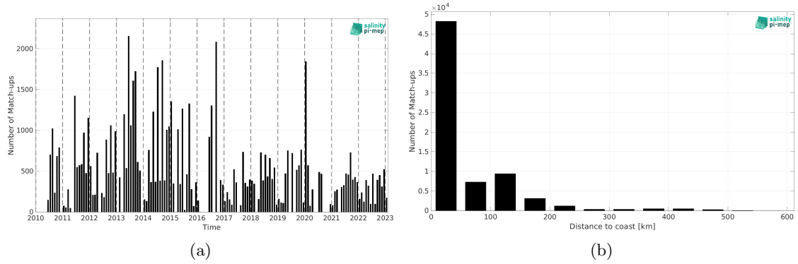
Figure 2: Number of match-ups between TSG (LEGOS-DM) and SMOS SSS L4 OI v346 - Weekly (CMEMS-CATDS-LOPS) SSS as a function of time (a) and as function of the distance to coast (b) over the Arctic Ocean Pi-MEP region and for the full satellite product period.
