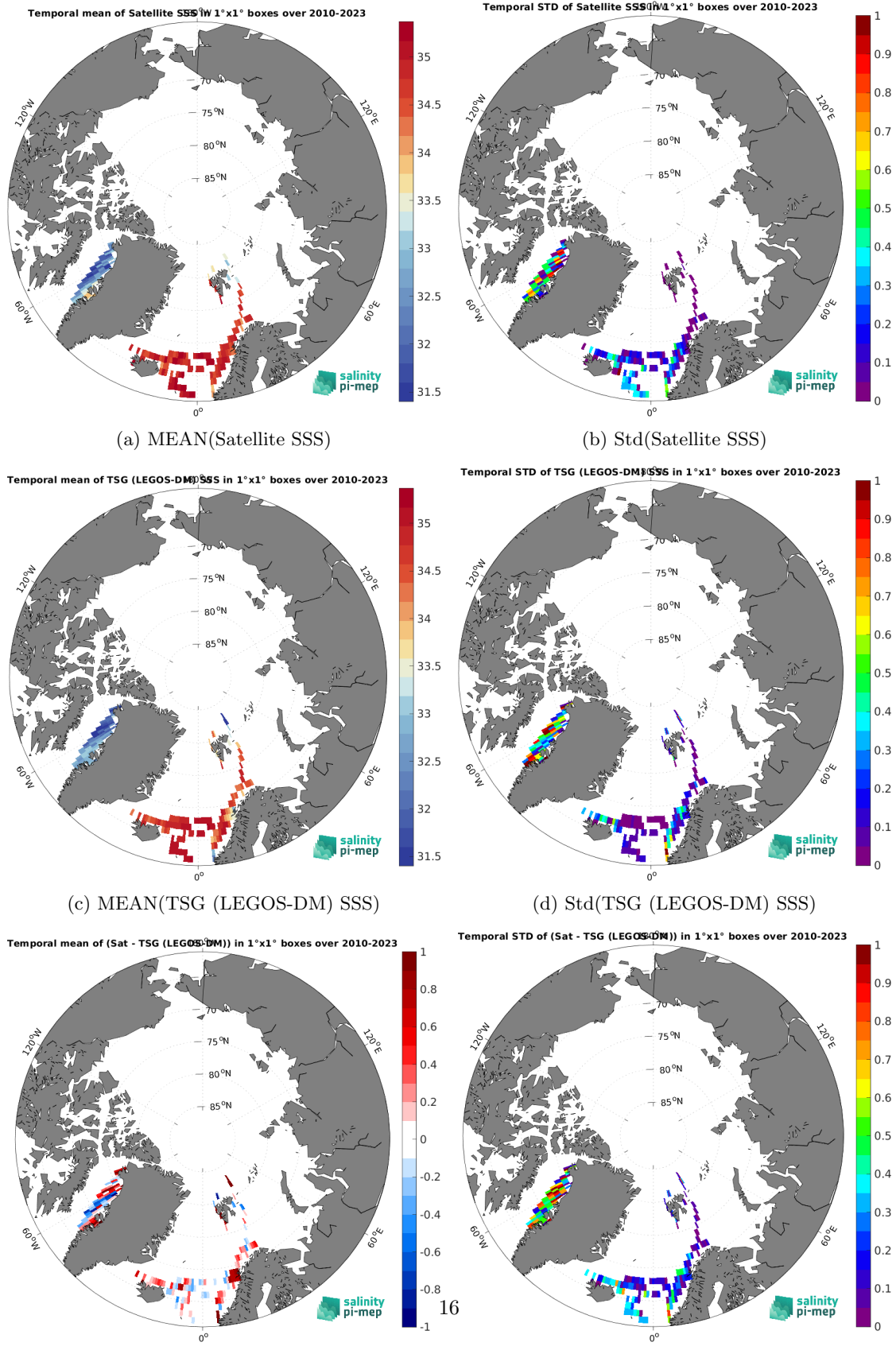
(e) MEAN( \Delta SSS) (Satellite - TSG (LEGOS-DM)) (f) Std( \Delta SSS) (Satellite - TSG (LEGOS-DM)) Figure 7: Temporal mean (left) and Std (right) of SSS from SMOS SSS L4 OI v346 - Weekly (CMEMS-CATDS-LOPS) (top), TSG (LEGOS-DM) (middle), and of \Delta SSS (Satellite - TSG (LEGOS-DM)). Only match-up pairs are used to generate these maps.
