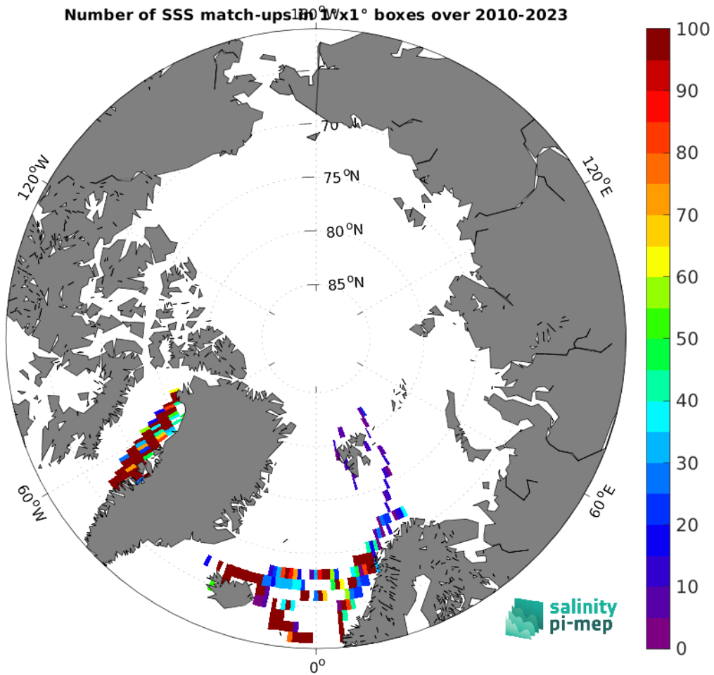
Figure 5: Number of SSS match-ups between TSG (LEGOS-DM) SSS and the SMOS SSS L4 OI v346 - Weekly (CMEMS-CATDS-LOPS) SSS product for the Arctic Ocean Pi-MEP region over 1^\circ \times 1^\circ boxes and for the full satellite product period.
