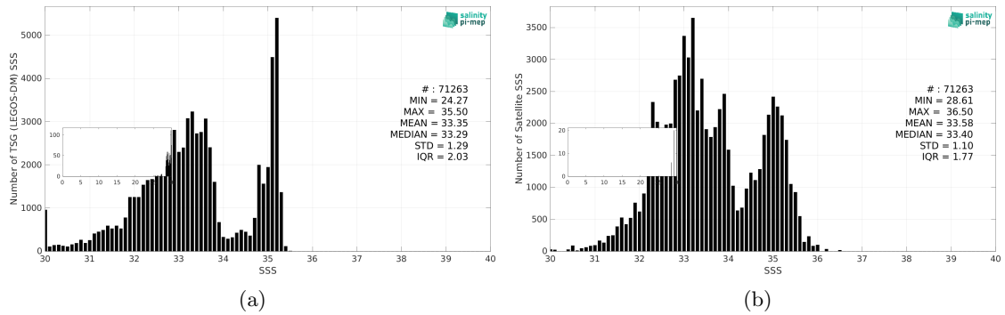
Figure 3: Histograms of SSS from TSG (LEGOS-DM) (a) and SMOS SSS L4 OI v346 - Weekly (CMEMS-CATDS-LOPS) (b) considering all match-up pairs per bins of 0.1 over the Arctic Ocean Pi-MEP region and for the full satellite product period.
