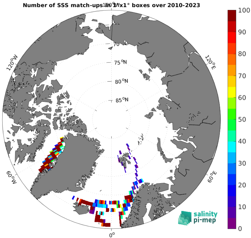
Figure 5: Number of SSS match-ups between TSG (LEGOS-DM) SSS and the SMOS SSS L4 OI v346 - Weekly (CMEMS-CATDS-LOPS) SSS product for the Arctic Ocean Pi-MEP region over 1^{\circ} \times 1^{\circ} boxes and for the full satellite product period.
