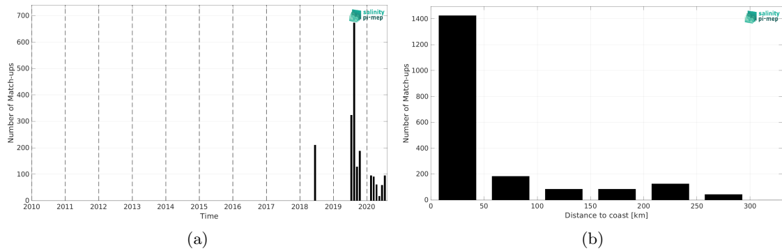
Figure 2: Number of match-ups between TSG (Lauge-Koch) and SMOS SSS L4 OI v346 - Weekly (CMEMS-CATDS-LOPS) SSS as a function of time (a) and as function of the distance to coast (b) over the Arctic Ocean Pi-MEP region and for the full satellite product period.
