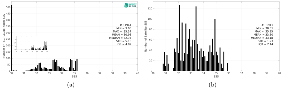
Figure 3: Histograms of SSS from TSG (Lauge-Koch) (a) and SMOS SSS L4 OI v346 - Weekly (CMEMS-CATDS-LOPS) (b) considering all match-up pairs per bins of 0.1 over the Arctic Ocean Pi-MEP region and for the full satellite product period.
