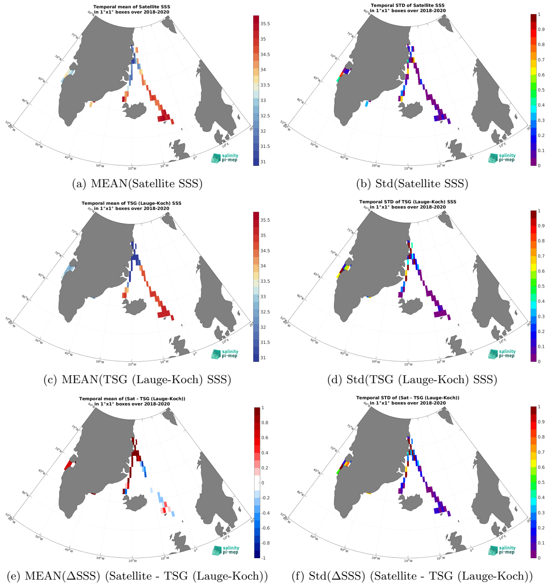
Figure 7: Temporal mean (left) and Std (right) of SSS from SMOS SSS L4 OI v346 - Weekly (CMEMS-CATDS-LOPS) (top), TSG (Lauge-Koch) (middle), and of \Delta SSS (Satellite - TSG (Lauge-Koch)). Only match-up pairs are used to generate these maps.
