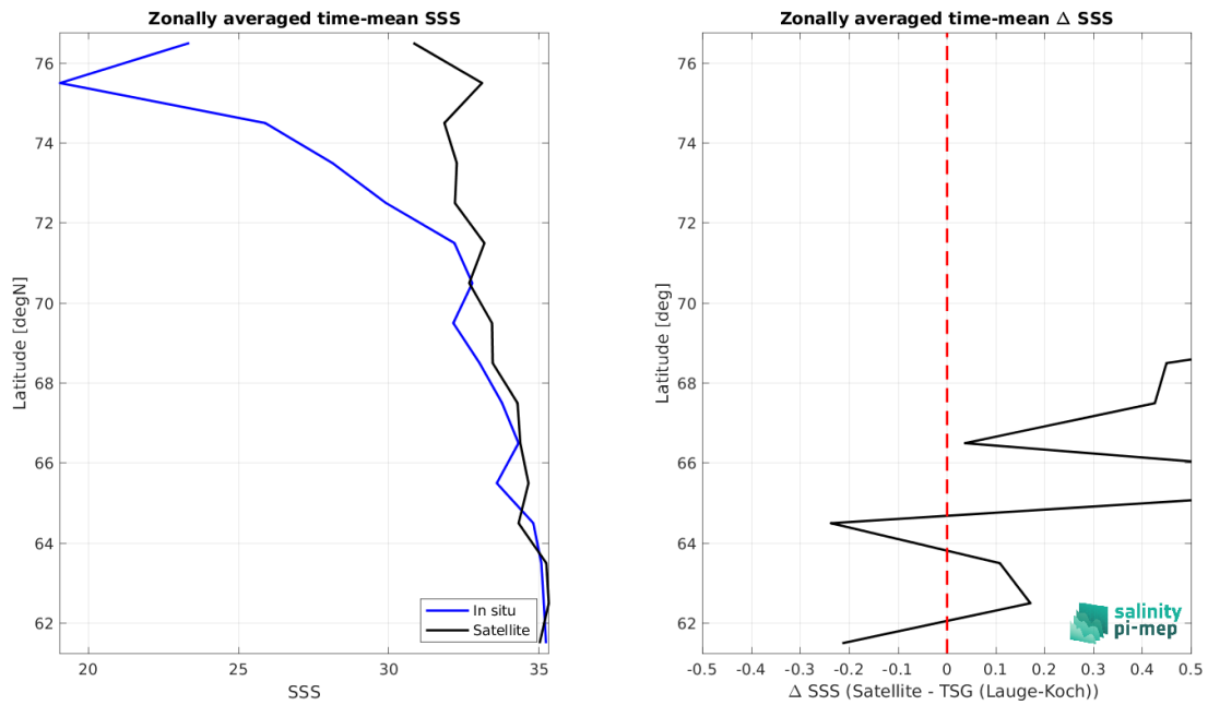
Figure 9: Left panel: Zonal mean SSS from SMOS SSS L4 OI v346 - Weekly (CMEMS-CATDS-LOPS) satellite product (black) and from TSG (Lauge-Koch) (blue). Right panel: Zonal mean of \Delta SSS (Satellite - TSG (Lauge-Koch)) for all the collected Pi-MEP match-up pairs estimated over the full satellite product period.
