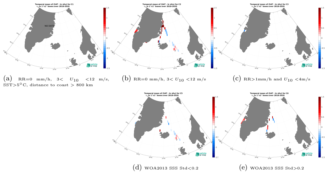
Figure 14: Temporal mean gridded over spatial boxes of size 1^\circ \times 1^\circ of \Delta SSS (SMOS SSS L4 OI v346 - Weekly (CMEMS-CATDS-LOPS) - TSG (Lauge-Koch)) for 5 different subdatasets corresponding to: RR=0 mm/h, 3 < U_{10} < 12 m/s, SST > 5^\circ\text{C} , distance to coast > 800 km (a), RR=0 mm/h, 3 < U_{10} < 12 m/s (b), RR > 1 mm/h and U_{10} < 4 m/s (c), WOA2013 SSS Std < 0.2 (d), WOA2013 SSS Std > 0.2 (e).
