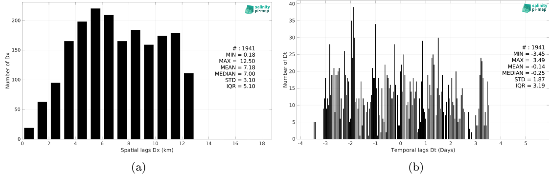
Figure 6: Histograms of the spatial (a) and temporal (b) lags between the location/time of the TSG (Lauge-Koch) measurement and the date of the corresponding SMOS SSS L4 OI v346 - Weekly (CMEMS-CATDS-LOPS) SSS pixel.
