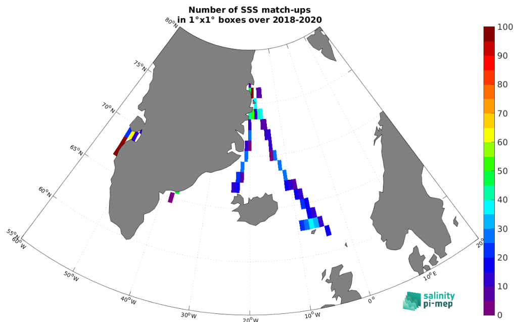
Figure 5: Number of SSS match-ups between TSG (Lauge-Koch) SSS and the SMOS SSS L4 OI v346 - Weekly (CMEMS-CATDS-LOPS) SSS product for the Arctic Ocean Pi-MEP region over 1^\circ \times 1^\circ boxes and for the full satellite product period.
