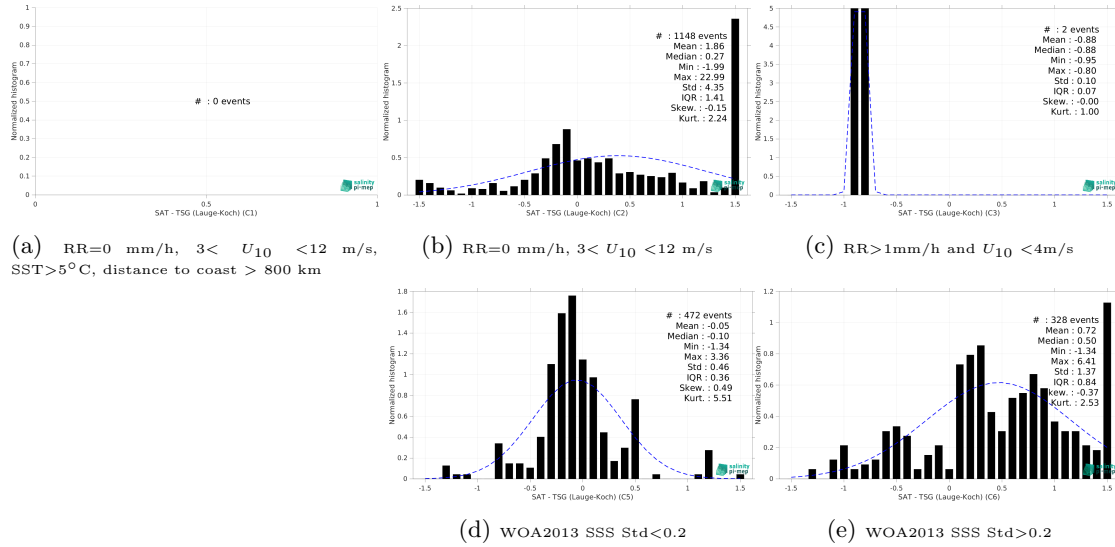
Figure 15: Normalized histogram of \Delta SSS (SMOS SSS L4 OI v346 - Weekly (CMEMS-CATDS-LOPS) - TSG (Lauge-Koch)) for 5 different subdatasets corresponding to: RR=0 mm/h, 3 < U_{10} < 12 m/s, SST > 5°C, distance to coast > 800 km (a), RR=0 mm/h, 3 < U_{10} < 12 m/s (b), RR > 1mm/h and U_{10} < 4 m/s (c), WOA2013 SSS Std < 0.2 (d), WOA2013 SSS Std > 0.2 (e).
