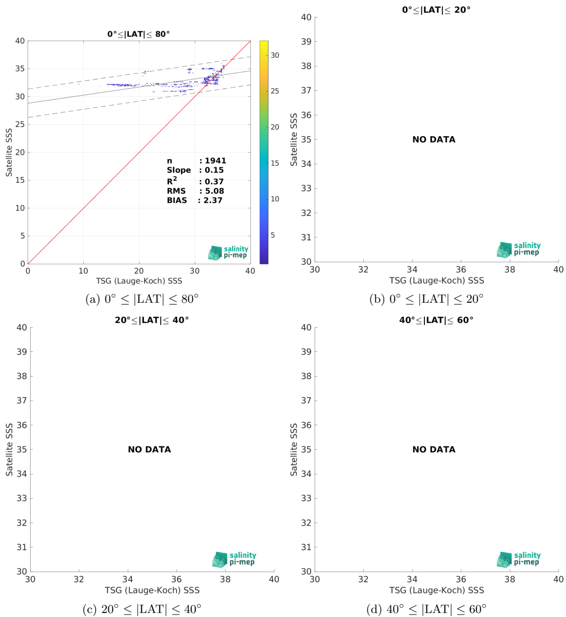
Figure 10: Contour maps of the concentration of SMOS SSS L4 OI v346 - Weekly (CMEMS-CATDS-LOPS) SSS (y-axis) versus TSG (Lauge-Koch) SSS (x-axis) at match-up pairs for different latitude bands. For each plot, the red line shows x=y . The black thin and dashed lines indicate a linear fit through the data cloud and the \pm 95\% confidence levels, respectively. The number match-up pairs n , the slope and R^2 coefficient of the linear fit, the root mean square (RMS) and the mean bias between satellite and in situ data are indicated for each latitude band in each plots.
