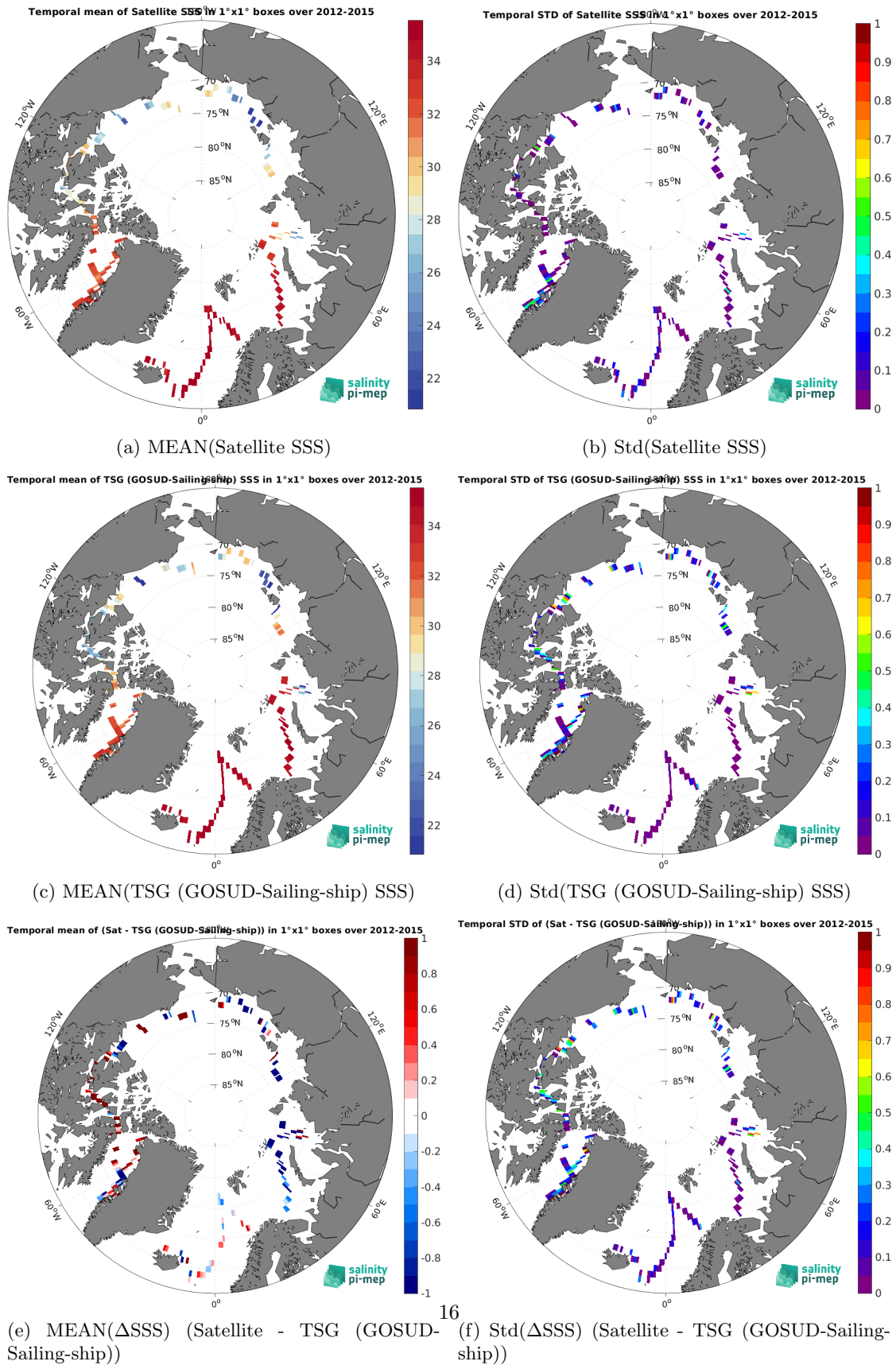
Figure 7: Temporal mean (left) and Std (right) of SSS from SMOS SSS L4 OI v346 - Weekly (CMEMS-CATDS-LOPS) (top), TSG (GOSUD-Sailing-ship) (middle), and of \Delta SSS (Satellite - TSG (GOSUD-Sailing-ship)). Only match-up pairs are used to generate these maps.
