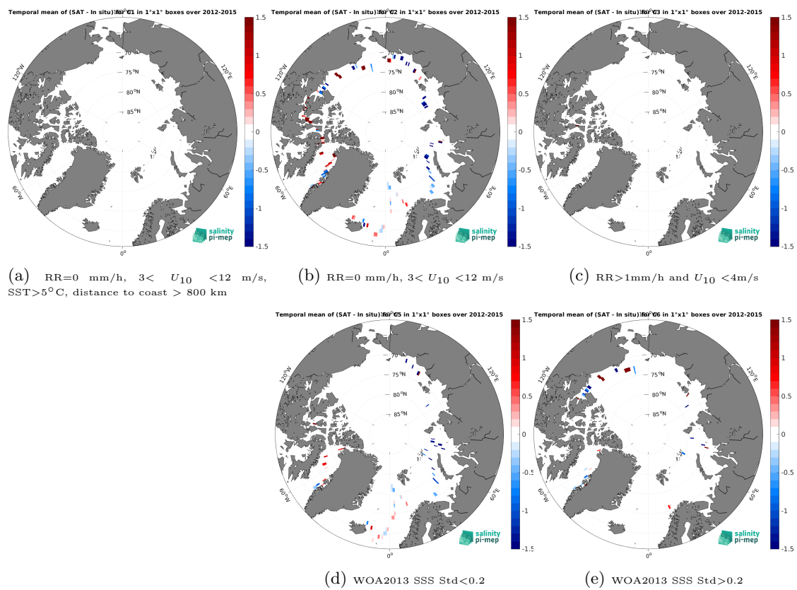
Figure 14: Temporal mean gridded over spatial boxes of size 1^\circ \times 1^\circ of \Delta\text{SSS} (SMOS SSS L4 OI v346 - Weekly (CMEMS-CATDS-LOPS) - TSG (GOSUD-Sailing-ship)) for 5 different sub-datasets corresponding to:RR=0 mm/h, 3 < U_{10} < 12 m/s, SST>5°C, distance to coast > 800 km (a), RR=0 mm/h, 3 < U_{10} < 12 m/s (b), RR>1mm/h and U_{10} < 4 m/s (c), WOA2013 SSS Std<0.2 (d), WOA2013 SSS Std>0.2 (e).
