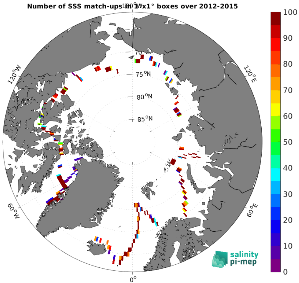
Figure 5: Number of SSS match-ups between TSG (GOSUD-Sailing-ship) SSS and the SMOS SSS L4 OI v346 - Weekly (CMEMS-CATDS-LOPS) SSS product for the Arctic Ocean Pi-MEP region over 1^{\circ} \times 1^{\circ} boxes and for the full satellite product period.
