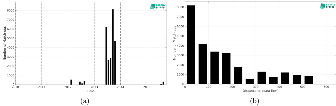
Figure 2: Number of match-ups between TSG (GOSUD-Sailing-ship) and SMOS SSS L4 OI v346 - Weekly (CMEMS-CATDS-LOPS) SSS as a function of time (a) and as function of the distance to coast (b) over the Arctic Ocean Pi-MEP region and for the full satellite product period.
