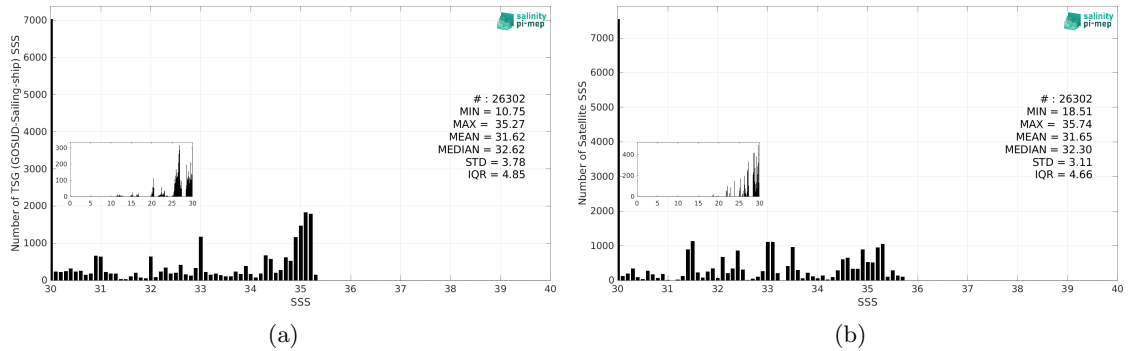
Figure 3: Histograms of SSS from TSG (GOSUD-Sailing-ship) (a) and SMOS SSS L4 OI v346 - Weekly (CMEMS-CATDS-LOPS) (b) considering all match-up pairs per bins of 0.1 over the Arctic Ocean Pi-MEP region and for the full satellite product period.
