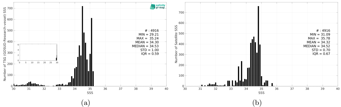
Figure 3: Histograms of SSS from TSG (GOSUD-Research-vessel) (a) and SMOS SSS L4 OI v346 - Weekly (CMEMS-CATDS-LOPS) (b) considering all match-up pairs per bins of 0.1 over the Arctic Ocean Pi-MEP region and for the full satellite product period.
