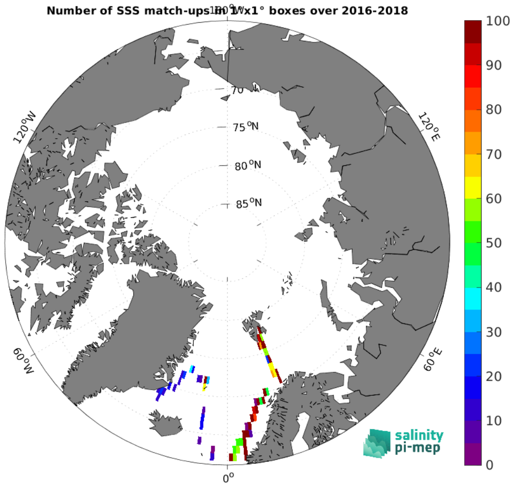
Figure 5: Number of SSS match-ups between TSG (GOSUD-Research-vessel) SSS and the SMOS SSS L4 OI v346 - Weekly (CMEMS-CATDS-LOPS) SSS product for the Arctic Ocean Pi-MEP region over 1^\circ \times 1^\circ boxes and for the full satellite product period.
