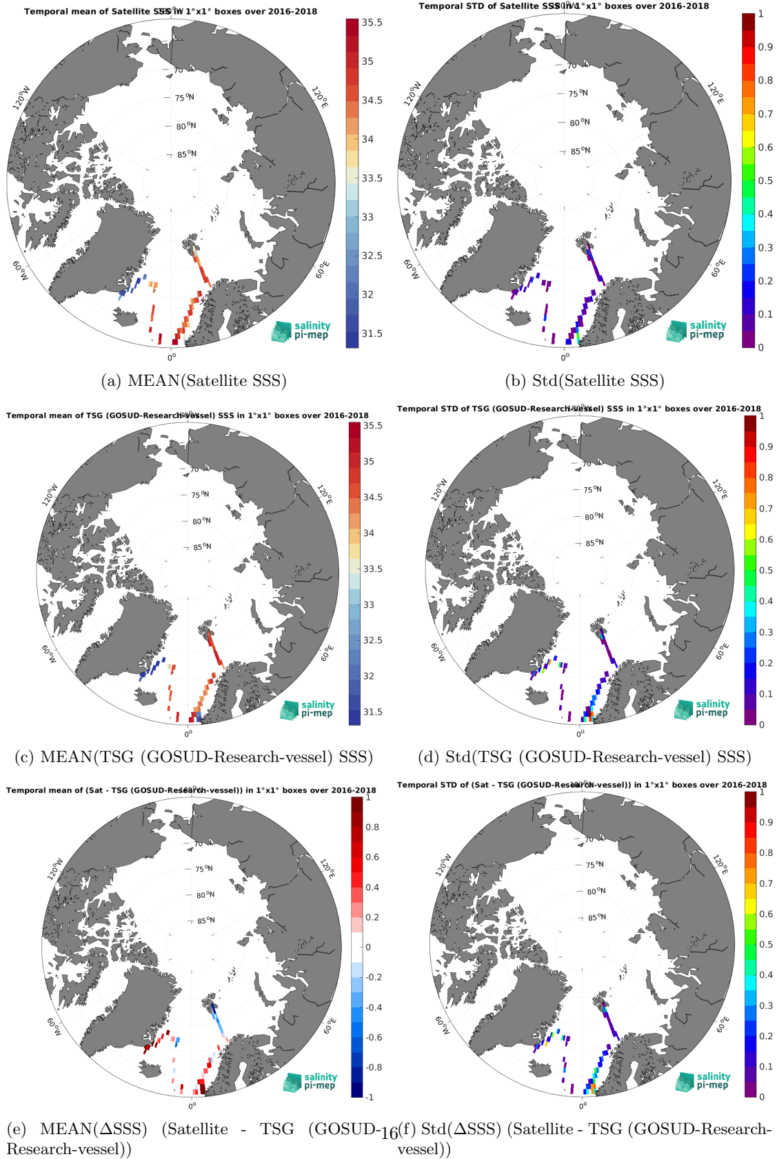
Figure 7: Temporal mean (left) and Std (right) of SSS from SMOS SSS L4 OI v346 - Weekly (CMEMS-CATDS-LOPS) (top), TSG (GOSUD-Research-vessel) (middle), and of \Delta SSS (Satellite - TSG (GOSUD-Research-vessel)). Only match-up pairs are used to generate these maps.
