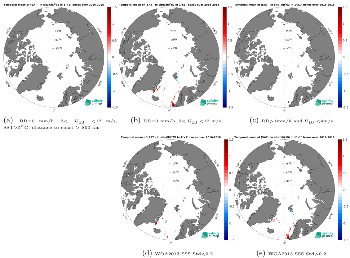
Figure 14: Temporal mean gridded over spatial boxes of size 1^\circ \times 1^\circ of \Delta\text{SSS} (SMOS SSS L4 OI v346 - Weekly (CMEMS-CATDS-LOPS) - TSG (GOSUD-Research-vessel)) for 5 different subdatasets corresponding to:RR=0 mm/h, 3 < U_{10} < 12 m/s, SST > 5°C, distance to coast > 800 km (a), RR=0 mm/h, 3 < U_{10} < 12 m/s (b), RR > 1mm/h and U_{10} < 4 m/s (c), WOA2013 SSS Std < 0.2 (d), WOA2013 SSS Std > 0.2 (e).
