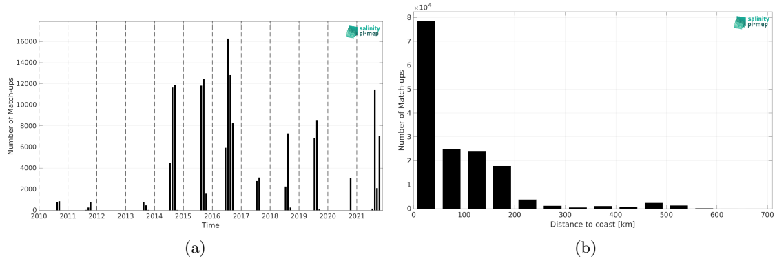
Figure 2: Number of match-ups between TSG (Amundsen) and SMOS SSS L4 OI v346 - Weekly (CMEMS-CATDS-LOPS) SSS as a function of time (a) and as function of the distance to coast (b) over the Arctic Ocean Pi-MEP region and for the full satellite product period.
