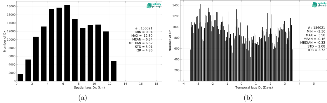
Figure 6: Histograms of the spatial (a) and temporal (b) lags between the location/time of the TSG (Amundsen) measurement and the date of the corresponding SMOS SSS L4 OI v346 - Weekly (CMEMS-CATDS-LOPS) SSS pixel.
