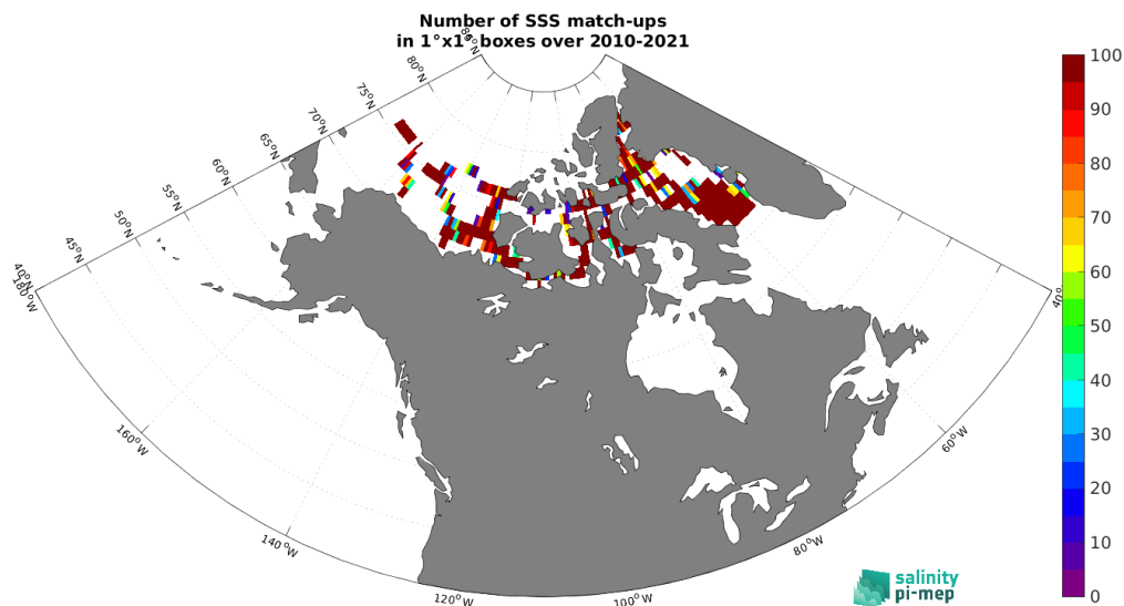
Figure 5: Number of SSS match-ups between TSG (Amundsen) SSS and the SMOS SSS L4 OI v346 - Weekly (CMEMS-CATDS-LOPS) SSS product for the Arctic Ocean Pi-MEP region over 1^\circ \times 1^\circ boxes and for the full satellite product period.
