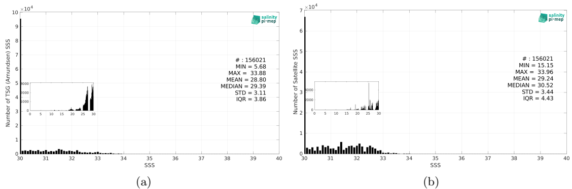
Figure 3: Histograms of SSS from TSG (Amundsen) (a) and SMOS SSS L4 OI v346 - Weekly (CMEMS-CATDS-LOPS) (b) considering all match-up pairs per bins of 0.1 over the Arctic Ocean Pi-MEP region and for the full satellite product period.
