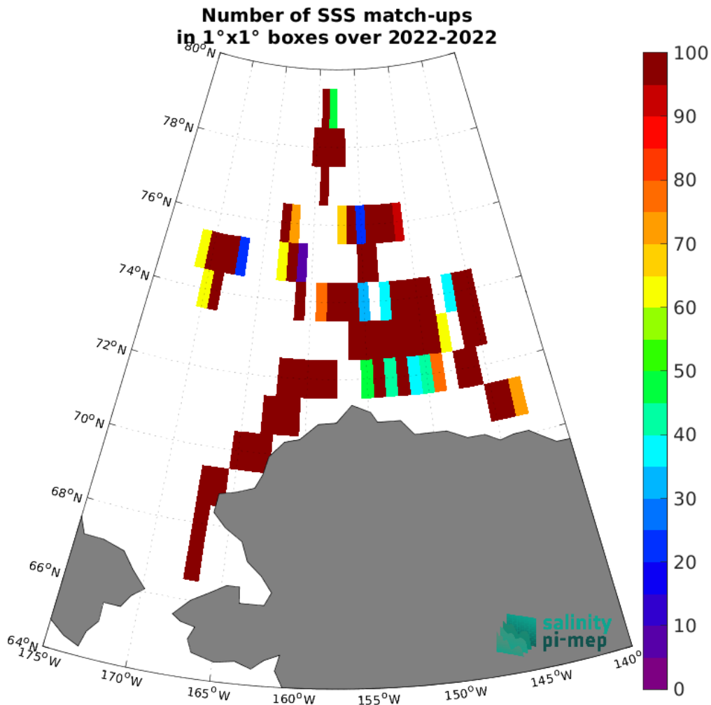
Figure 5: Number of SSS match-ups between SASSIE SSS and the SMOS SSS L4 OI v346 - Weekly (CMEMS-CATDS-LOPS) SSS product for the Arctic Ocean Pi-MEP region over 1^\circ \times 1^\circ boxes and for the full satellite product period.
