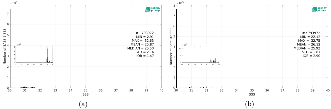
Figure 3: Histograms of SSS from SASSIE (a) and SMOS SSS L4 OI v346 - Weekly (CMEMS-CATDS-LOPS) (b) considering all match-up pairs per bins of 0.1 over the Arctic Ocean Pi-MEP region and for the full satellite product period.
