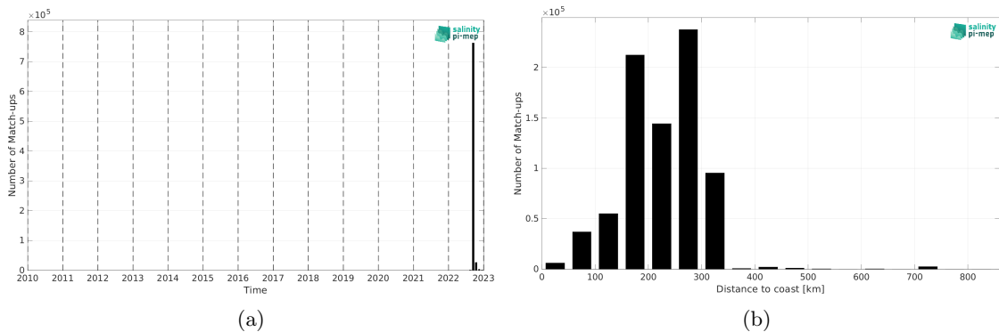
Figure 2: Number of match-ups between SASSIE and SMOS SSS L4 OI v346 - Weekly (CMEMS-CATDS-LOPS) SSS as a function of time (a) and as function of the distance to coast (b) over the Arctic Ocean Pi-MEP region and for the full satellite product period.
