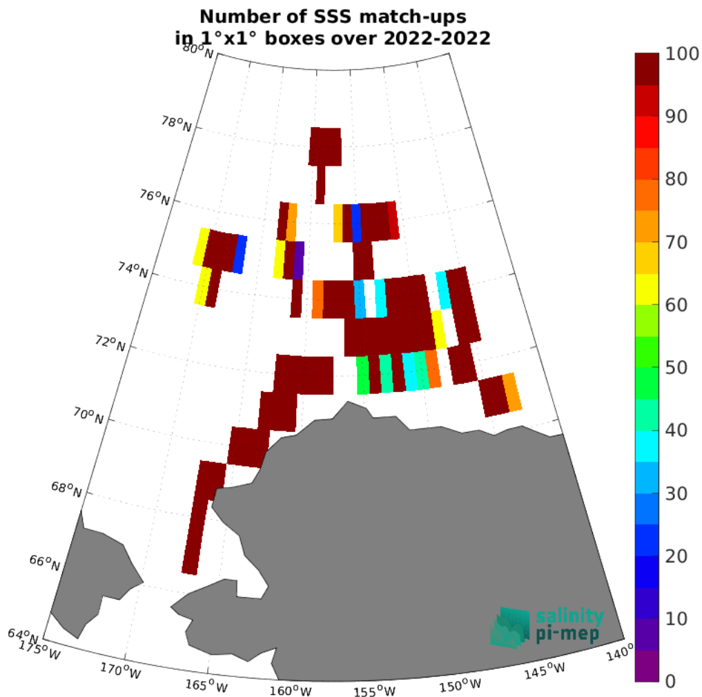
Figure 5: Number of SSS match-ups between SASSIE SSS and the SMOS SSS L4 OI v346 - Weekly (CMEMS-CATDS-LOPS) SSS product for the Arctic Ocean Pi-MEP region over 1°×1° boxes and for the full satellite product period.
