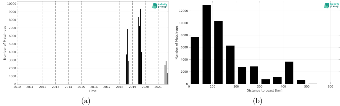
Figure 2: Number of match-ups between Saildrone and SMOS SSS L4 OI v346 - Weekly (CMEMS-CATDS-LOPS) SSS as a function of time (a) and as function of the distance to coast (b) over the Arctic Ocean Pi-MEP region and for the full satellite product period.
