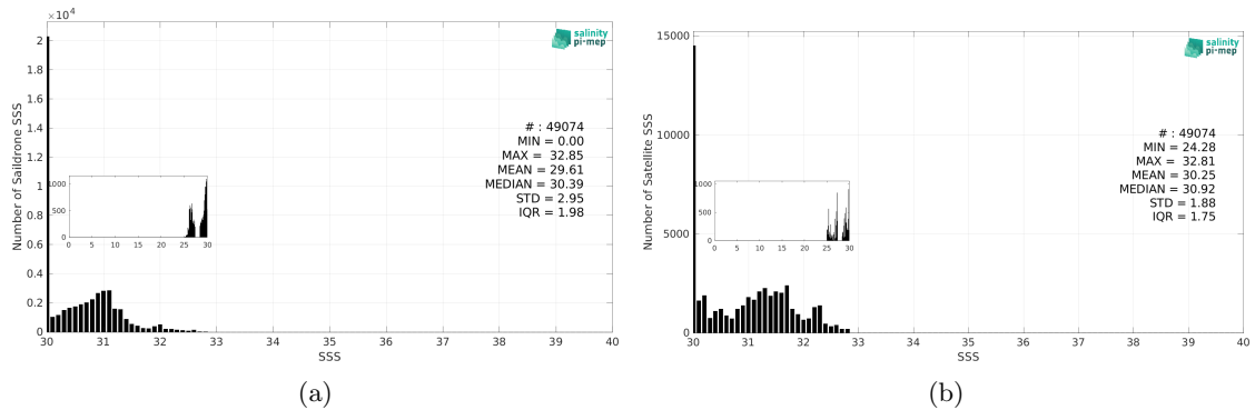
Figure 3: Histograms of SSS from Saildrone (a) and SMOS SSS L4 OI v346 - Weekly (CMEMS-CATDS-LOPS) (b) considering all match-up pairs per bins of 0.1 over the Arctic Ocean Pi-MEP region and for the full satellite product period.
