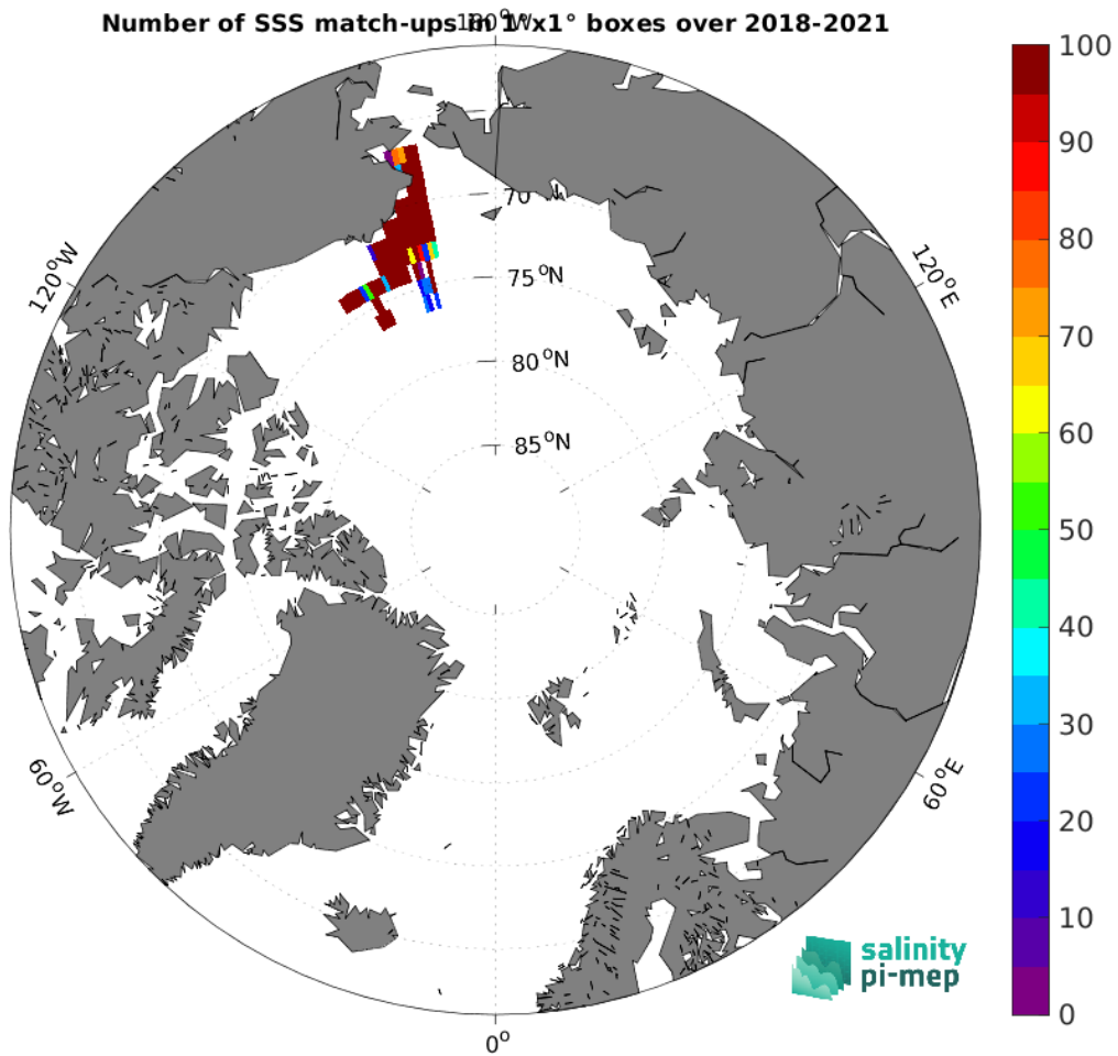
Figure 5: Number of SSS match-ups between Saildrone SSS and the SMOS SSS L4 OI v346 - Weekly (CMEMS-CATDS-LOPS) SSS product for the Arctic Ocean Pi-MEP region over 1^\circ \times 1^\circ boxes and for the full satellite product period.
