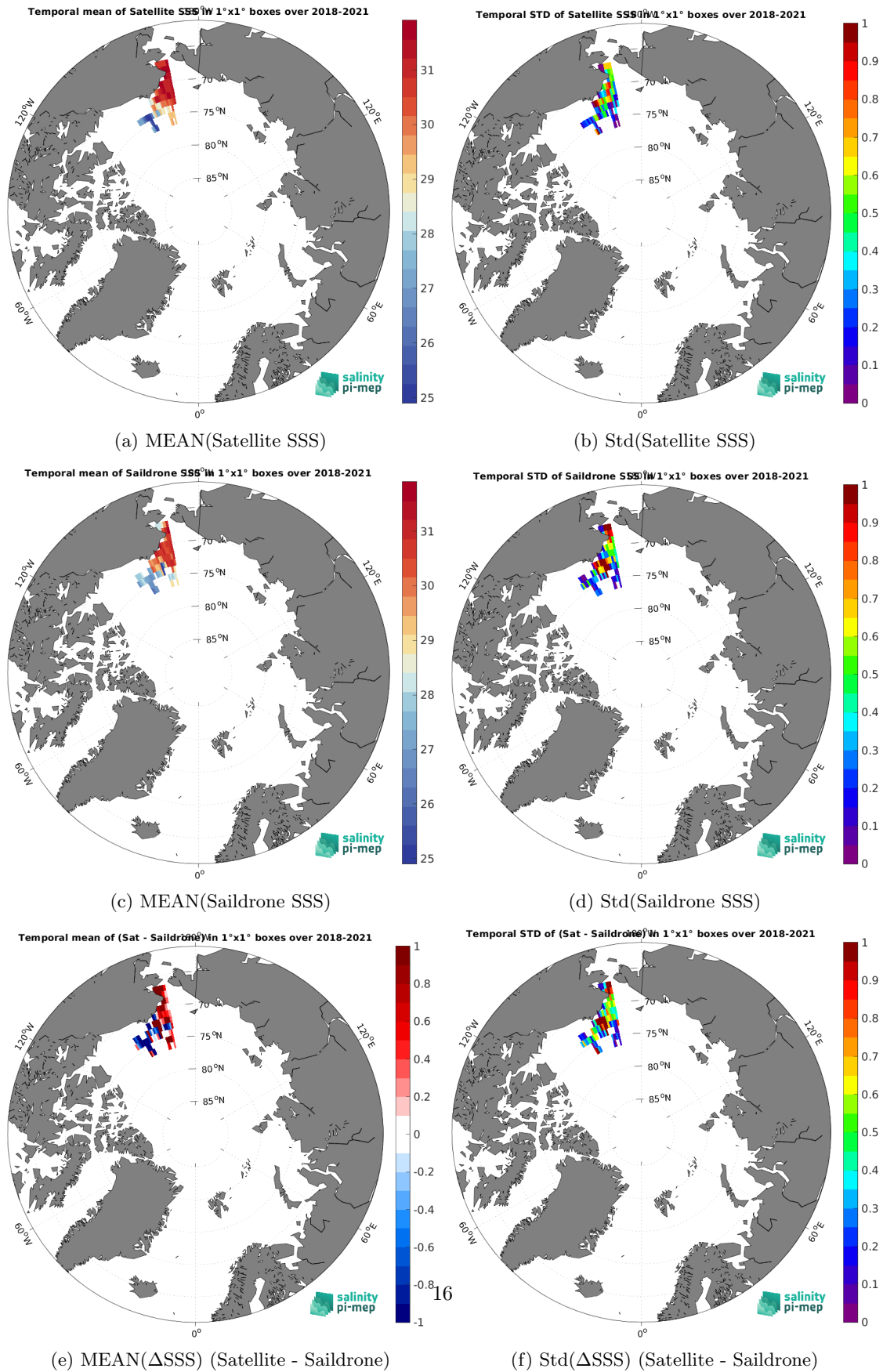
Figure 7: Temporal mean (left) and Std (right) of SSS from SMOS SSS L4 OI v346 - Weekly (CMEMS-CATDS-LOPS) (top), Saildrone (middle), and of \Delta SSS (Satellite - Saildrone). Only match-up pairs are used to generate these maps.
