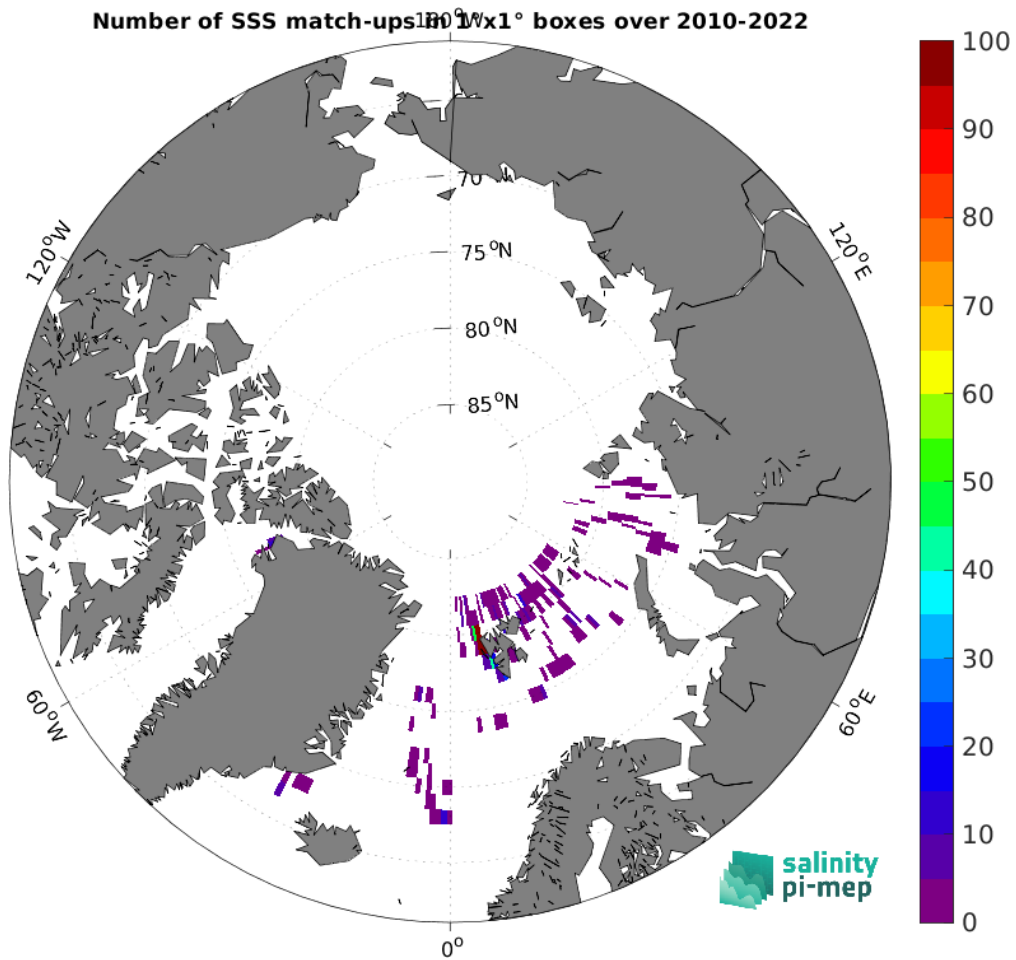
Figure 5: Number of SSS match-ups between Marine mammals SSS and the SMOS SSS L4 OI v346 - Weekly (CMEMS-CATDS-LOPS) SSS product for the Arctic Ocean Pi-MEP region over 1^\circ \times 1^\circ boxes and for the full satellite product period.
