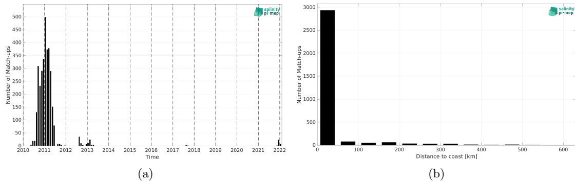
Figure 2: Number of match-ups between Marine mammals and SMOS SSS L4 OI v346 - Weekly (CMEMS-CATDS-LOPS) SSS as a function of time (a) and as function of the distance to coast (b) over the Arctic Ocean Pi-MEP region and for the full satellite product period.
