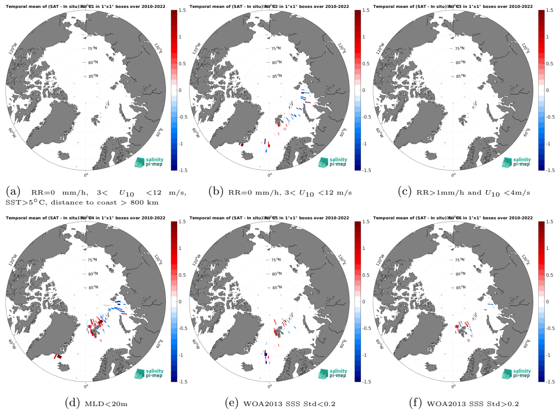
Figure 14: Temporal mean gridded over spatial boxes of size 1^\circ \times 1^\circ of \Delta\text{SSS} (SMOS SSS L4 OI v346 - Weekly (CMEMS-CATDS-LOPS) - Marine mammals) for 6 different subdatasets corresponding to: RR=0 mm/h, 3 < U_{10} < 12 m/s, SST > 5°C, distance to coast > 800 km (a), RR=0 mm/h, 3 < U_{10} < 12 m/s (b), RR > 1mm/h and U_{10} < 4 m/s (c), MLD < 20m (d), WOA2013 SSS Std < 0.2 (e), WOA2013 SSS Std > 0.2 (f).
