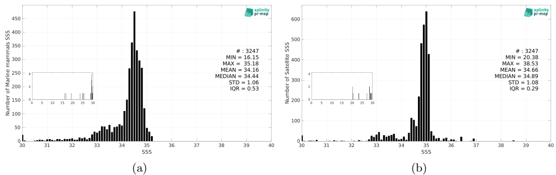
Figure 3: Histograms of SSS from Marine mammals (a) and SMOS SSS L4 OI v346 - Weekly (CMEMS-CATDS-LOPS) (b) considering all match-up pairs per bins of 0.1 over the Arctic Ocean Pi-MEP region and for the full satellite product period.
