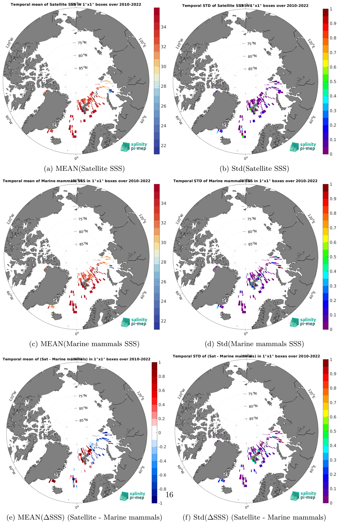
Figure 7: Temporal mean (left) and Std (right) of SSS from SMOS SSS L4 OI v346 - Weekly (CMEMS-CATDS-LOPS) (top), Marine mammals (middle), and of \Delta SSS (Satellite - Marine mammals). Only match-up pairs are used to generate these maps.
