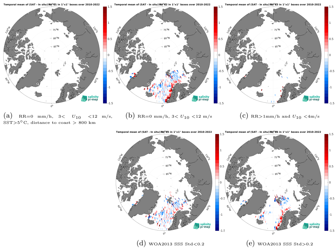
Figure 14: Temporal mean gridded over spatial boxes of size 1^\circ \times 1^\circ of \Delta SSS (SMOS SSS L4 OI v346 - Weekly (CMEMS-CATDS-LOPS) - ICES) for 5 different subdatasets corresponding to: RR=0 mm/h, 3 < U_{10} < 12 m/s, SST > 5^\circ\text{C} , distance to coast > 800 km (a), RR=0 mm/h, 3 < U_{10} < 12 m/s (b), RR > 1 mm/h and U_{10} < 4 m/s (c), WOA2013 SSS Std < 0.2 (d), WOA2013 SSS Std > 0.2 (e).
