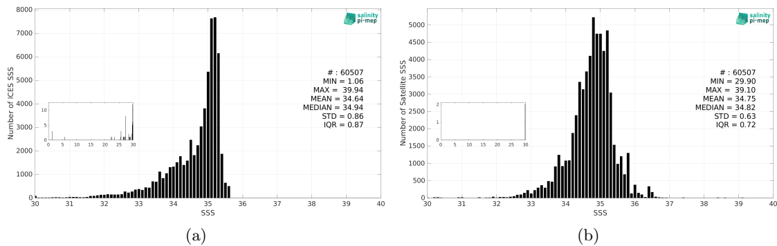
Figure 3: Histograms of SSS from ICES (a) and SMOS SSS L4 OI v346 - Weekly (CMEMS-CATDS-LOPS) (b) considering all match-up pairs per bins of 0.1 over the Arctic Ocean Pi-MEP region and for the full satellite product period.
