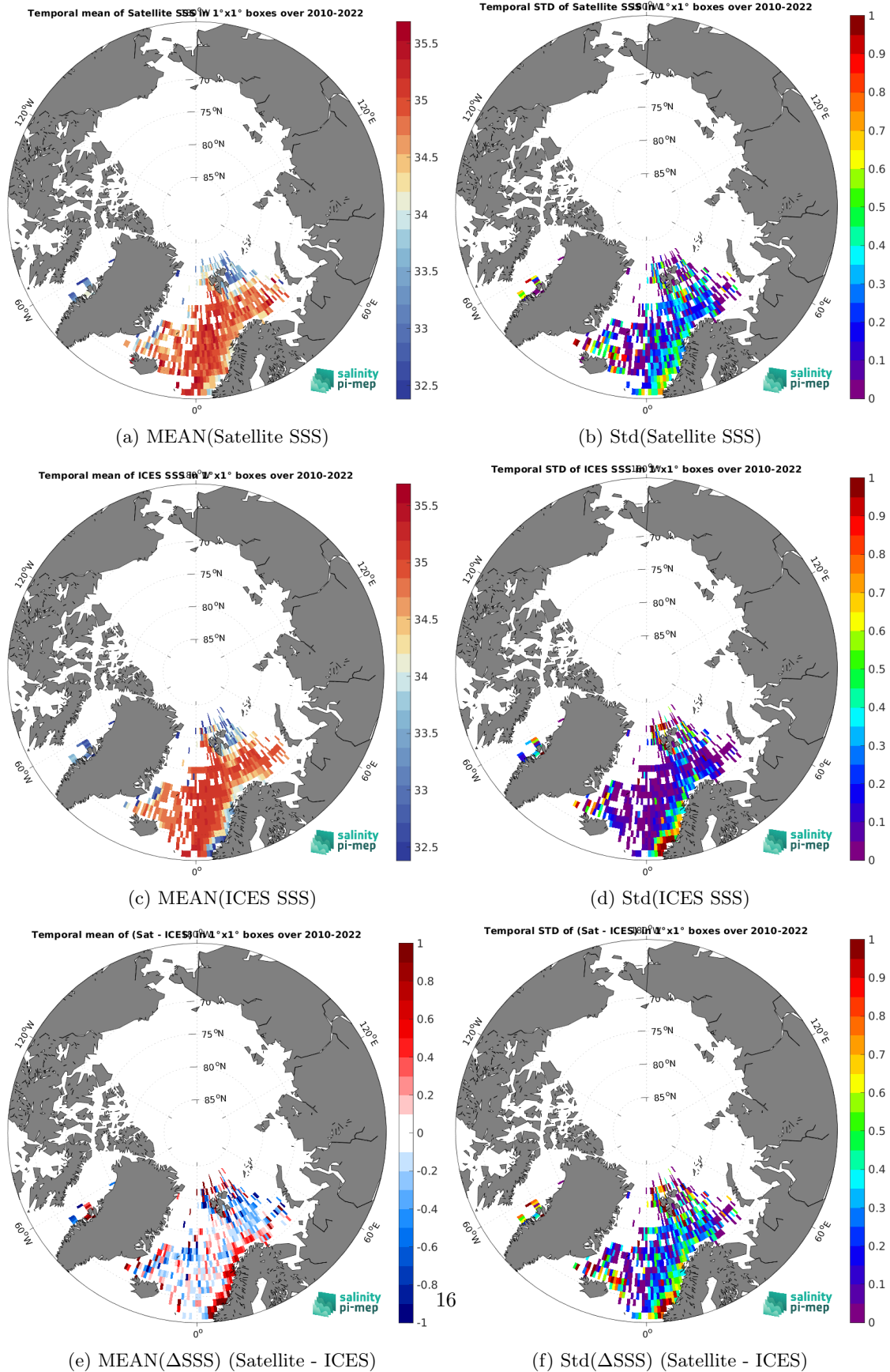
Figure 7: Temporal mean (left) and Std (right) of SSS from SMOS SSS L4 OI v346 - Weekly (CMEMS-CATDS-LOPS) (top), ICES (middle), and of \Delta SSS (Satellite - ICES). Only match-up pairs are used to generate these maps.
