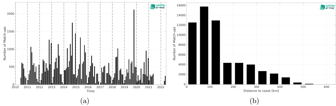
Figure 2: Number of match-ups between ICES and SMOS SSS L4 OI v346 - Weekly (CMEMS-CATDS-LOPS) SSS as a function of time (a) and as function of the distance to coast (b) over the Arctic Ocean Pi-MEP region and for the full satellite product period.
