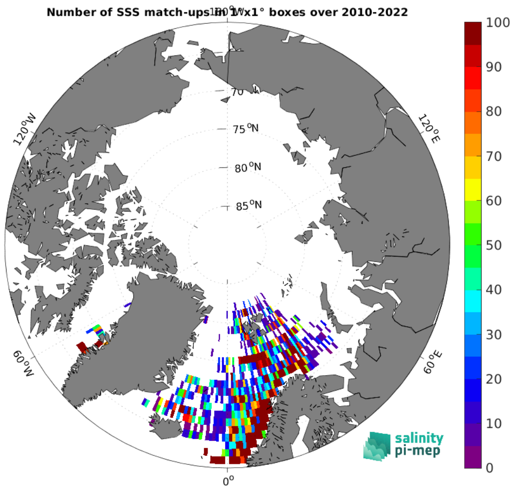
Figure 5: Number of SSS match-ups between ICES SSS and the SMOS SSS L4 OI v346 - Weekly (CMEMS-CATDS-LOPS) SSS product for the Arctic Ocean Pi-MEP region over 1^\circ \times 1^\circ boxes and for the full satellite product period.
