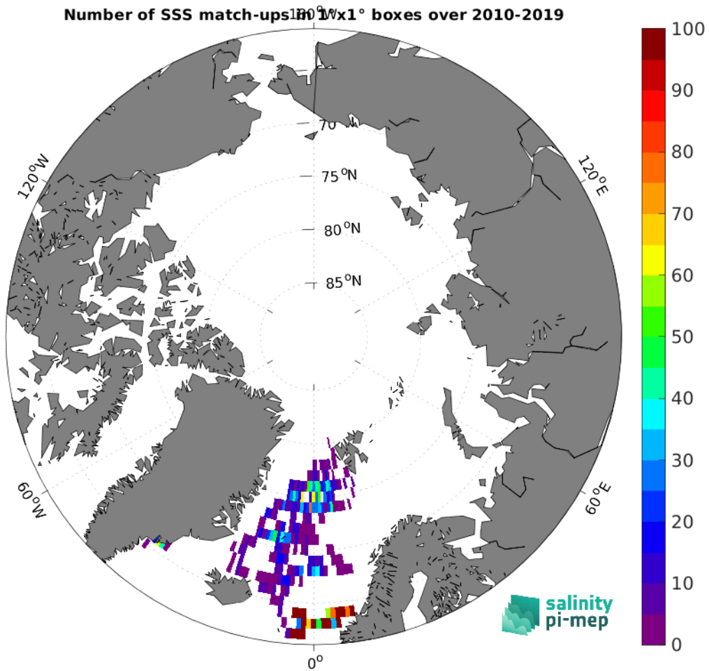
Figure 4: Number of SSS match-ups between Surface drifters SSS and the SMOS SSS L4 OI v346 - Weekly (CMEMS-CATDS-LOPS) SSS product for the Arctic Ocean Pi-MEP region over 1^\circ \times 1^\circ boxes and for the full satellite product period.
