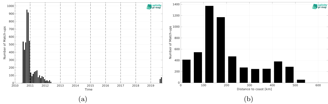
Figure 2: Number of match-ups between Surface drifters and SMOS SSS L4 OI v346 - Weekly (CMEMS-CATDS-LOPS) SSS as a function of time (a) and as function of the distance to coast (b) over the Arctic Ocean Pi-MEP region and for the full satellite product period.
