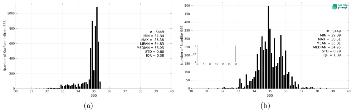
Figure 3: Histograms of SSS from Surface drifters (a) and SMOS SSS L4 OI v346 - Weekly (CMEMS-CATDS-LOPS) (b) considering all match-up pairs per bins of 0.1 over the Arctic Ocean Pi-MEP region and for the full satellite product period.
