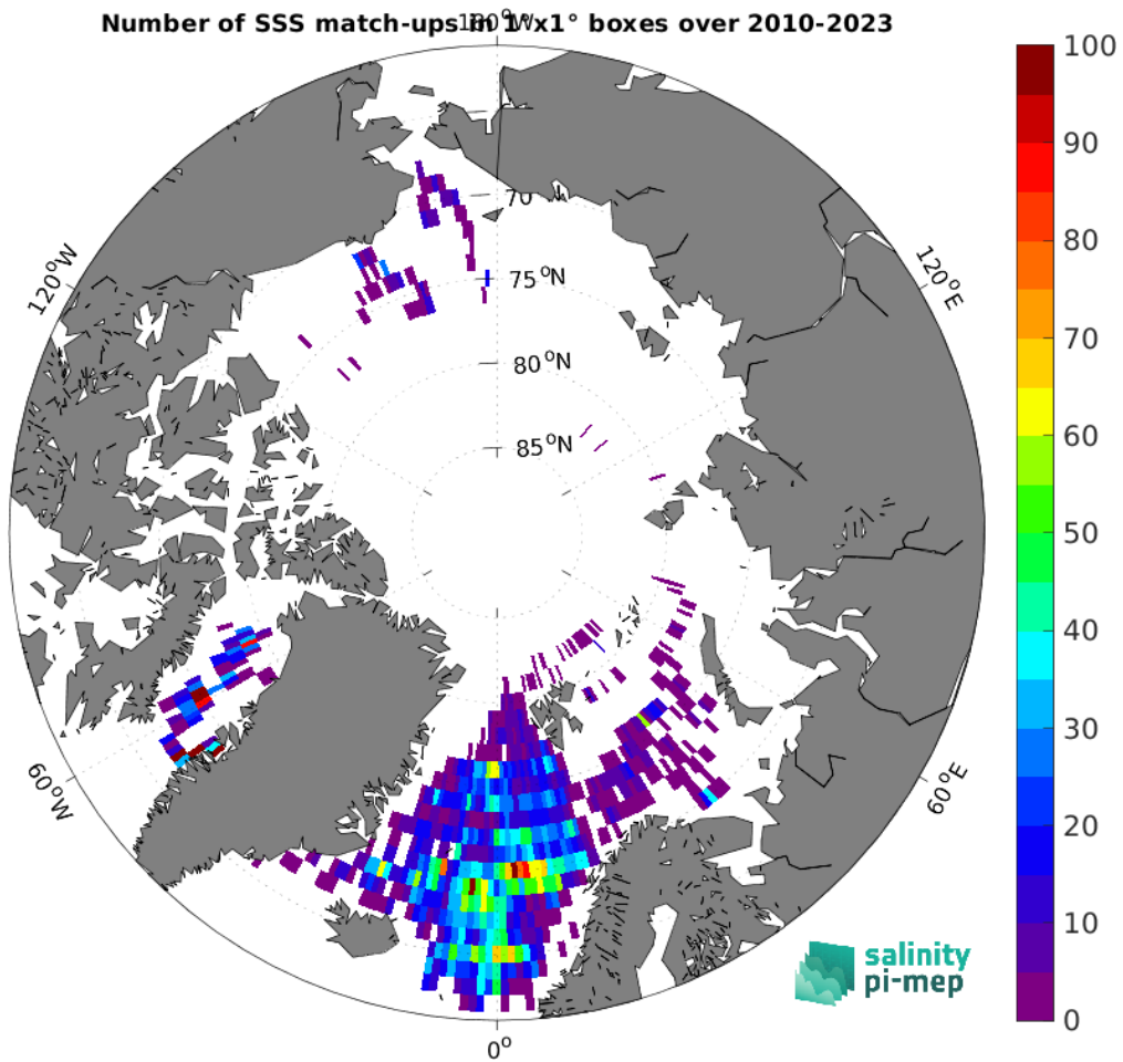
Figure 5: Number of SSS match-ups between Argo SSS and the SMOS SSS L4 OI v346 - Weekly (CMEMS-CATDS-LOPS) SSS product for the Arctic Ocean Pi-MEP region over 1^\circ \times 1^\circ boxes and for the full satellite product period.
