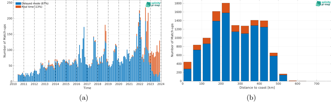
Figure 2: Number of match-ups between Argo and SMOS SSS L4 OI v346 - Weekly (CMEMS-CATDS-LOPS) SSS as a function of time (a) and as function of the distance to coast (b) over the Arctic Ocean Pi-MEP region and for the full satellite product period.
