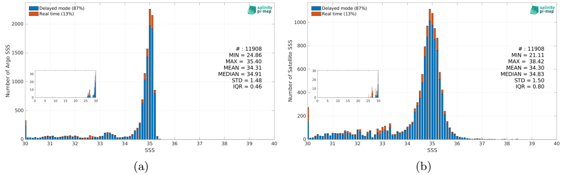
Figure 3: Histograms of SSS from Argo (a) and SMOS SSS L4 OI v346 - Weekly (CMEMS-CATDS-LOPS) (b) considering all match-up pairs per bins of 0.1 over the Arctic Ocean Pi-MEP region and for the full satellite product period.
