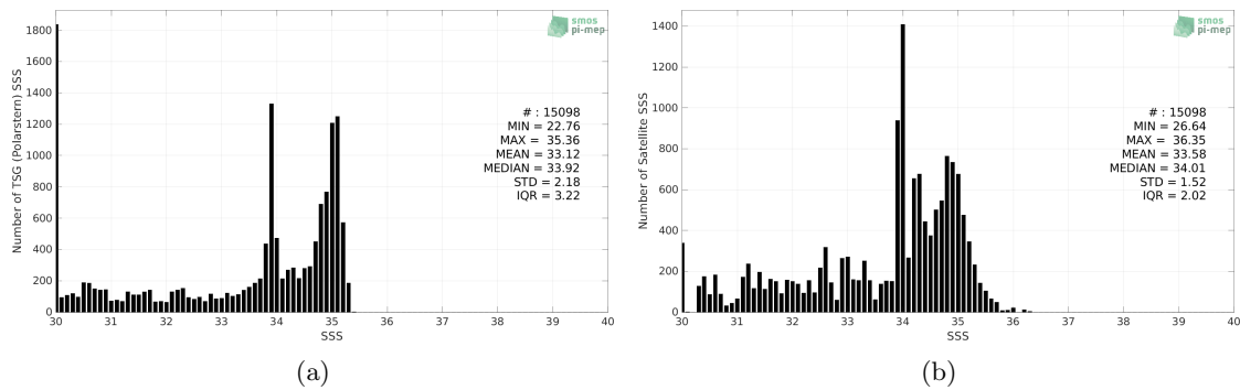
Figure 2: Histograms of SSS from TSG (Polarstern) (a) and SMOS SSS L4 OI v342 - Weekly (CMEMS-CATDS-LOPS) (b) considering all match-up pairs per bins of 0.1 over the Arctic Ocean Pi-MEP region and for the full satellite product period.
