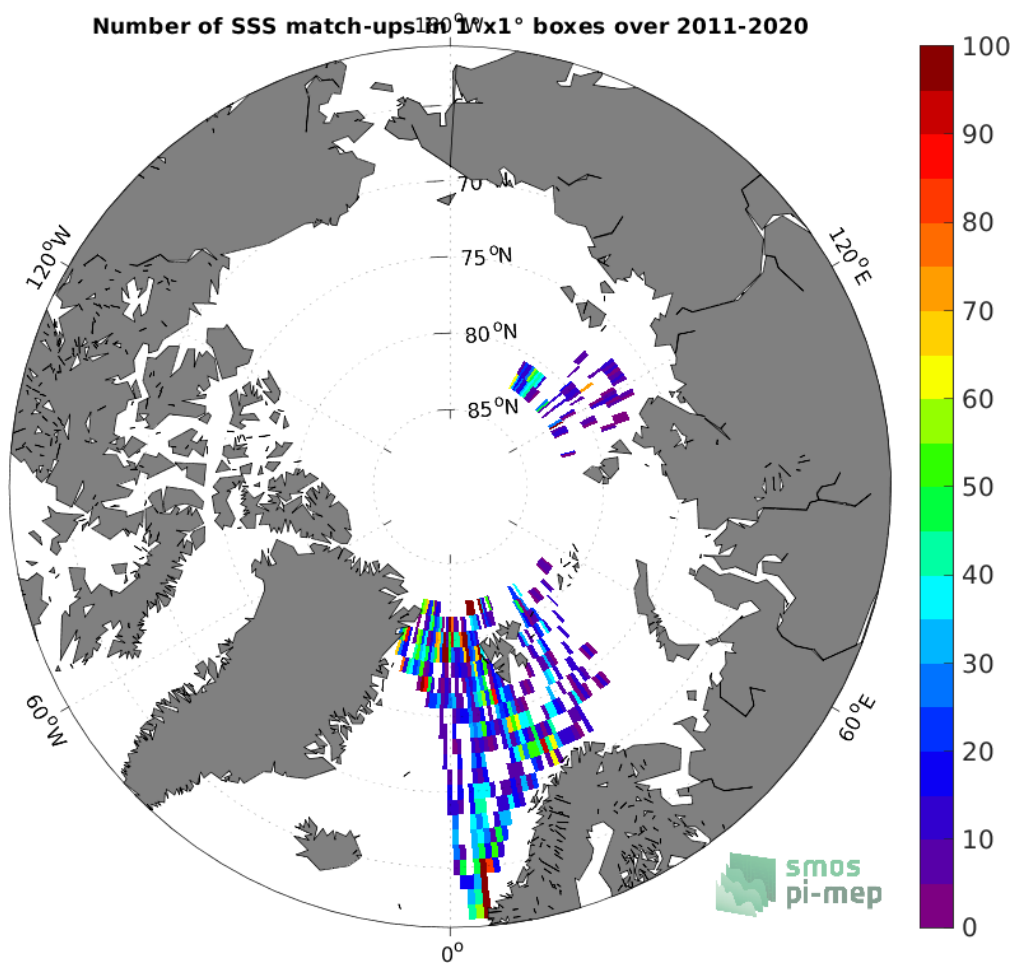
Figure 4: Number of SSS match-ups between TSG (Polarstern) SSS and the SMOS SSS L4 OI v342 - Weekly (CMEMS-CATDS-LOPS) SSS product for the Arctic Ocean Pi-MEP region over 1^\circ \times 1^\circ boxes and for the full satellite product period.
