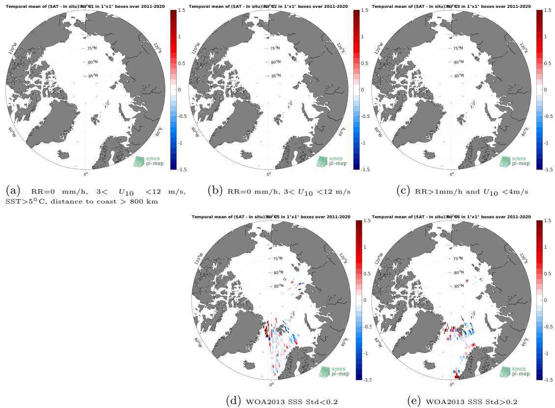
Figure 12: Temporal mean gridded over spatial boxes of size 1^{\circ}\times 1^{\circ} of \Delta\text{SSS} (SMOS SSS L4 OI v342 - Weekly (CMEMS-CATDS-LOPS) - TSG (Polarstern)) for 5 different subdatasets corresponding to:RR=0 mm/h, 3 < U_{10} < 12 m/s, SST > 5^{\circ}\text{C} , distance to coast > 800 km (a), RR=0 mm/h, 3 < U_{10} < 12 m/s (b), RR > 1 mm/h and U_{10} < 4 m/s (c), WOA2013 SSS Std < 0.2 (d), WOA2013 SSS Std > 0.2 (e).
