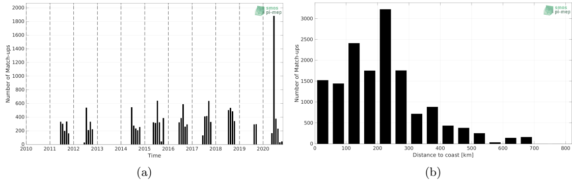
Figure 1: Number of match-ups between TSG (Polarstern) and SMOS SSS L4 OI v342 - Weekly (CMEMS-CATDS-LOPS) SSS as a function of time (a) and as function of the distance to coast (b) over the Arctic Ocean Pi-MEP region and for the full satellite product period.
