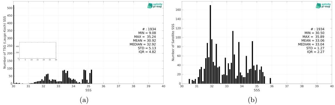
Figure 2: Histograms of SSS from TSG (Lauge-Koch) (a) and SMOS SSS L4 OI v342 - Weekly (CMEMS-CATDS-LOPS) (b) considering all match-up pairs per bins of 0.1 over the Arctic Ocean Pi-MEP region and for the full satellite product period.
