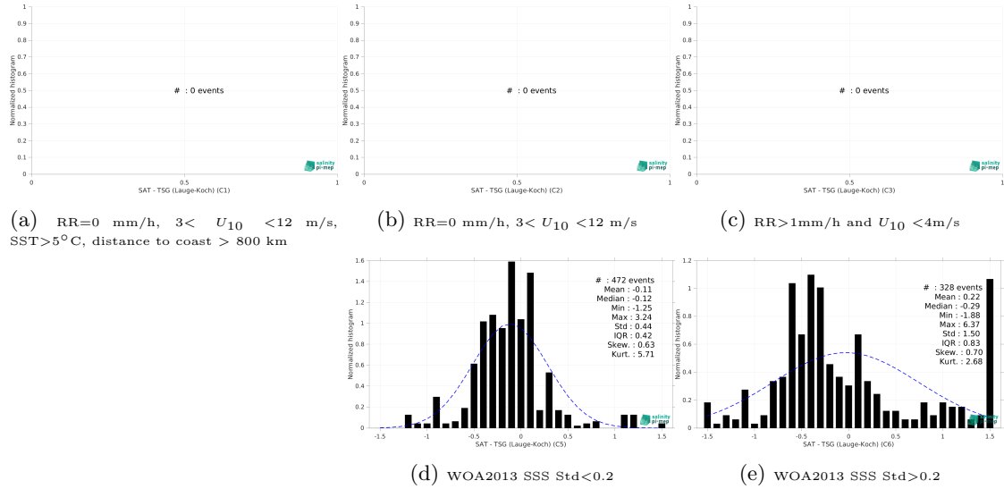
Figure 13: Normalized histogram of \Delta SSS (SMOS SSS L4 OI v342 - Weekly (CMEMS-CATDS-LOPS) - TSG (Lauge-Koch)) for 5 different subdatasets corresponding to: RR=0 mm/h, 3 < U_{10} < 12 m/s, SST>5°C, distance to coast > 800 km (a), RR=0 mm/h, 3 < U_{10} < 12 m/s (b), RR>1mm/h and U_{10} < 4 m/s (c), WOA2013 SSS Std<0.2 (d), WOA2013 SSS Std>0.2 (e).
