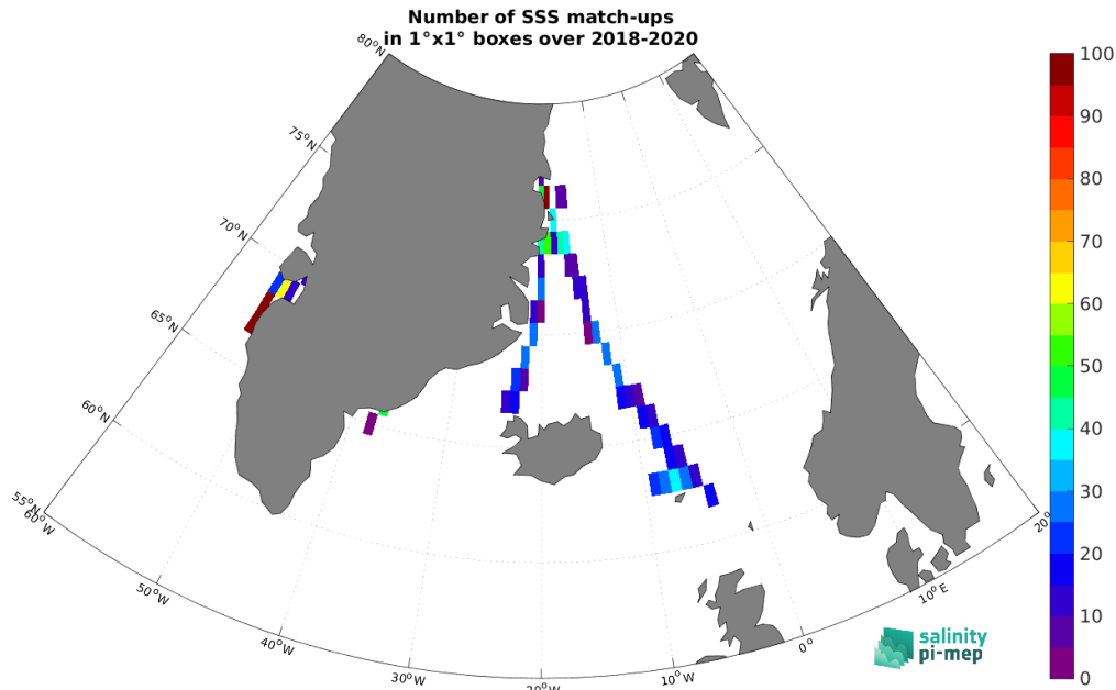
Figure 4: Number of SSS match-ups between TSG (Lauge-Koch) SSS and the SMOS SSS L4 OI v342 - Weekly (CMEMS-CATDS-LOPS) SSS product for the Arctic Ocean Pi-MEP region over 1^\circ \times 1^\circ boxes and for the full satellite product period.
