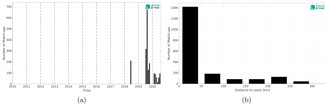
Figure 1: Number of match-ups between TSG (Lauge-Koch) and SMOS SSS L4 OI v342 - Weekly (CMEMS-CATDS-LOPS) SSS as a function of time (a) and as function of the distance to coast (b) over the Arctic Ocean Pi-MEP region and for the full satellite product period.
