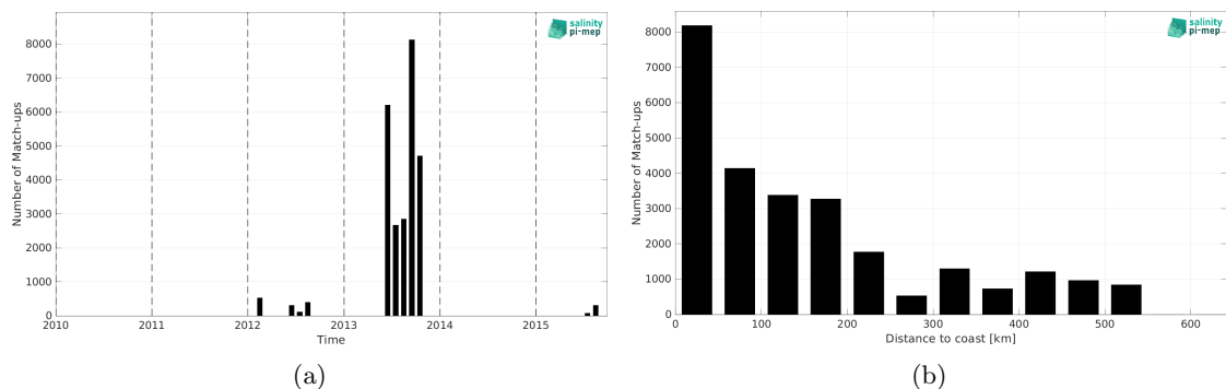
Figure 1: Number of match-ups between TSG (GOSUD-Sailing-ship) and SMOS SSS L4 OI v342 - Weekly (CMEMS-CATDS-LOPS) SSS as a function of time (a) and as function of the distance to coast (b) over the Arctic Ocean Pi-MEP region and for the full satellite product period.
