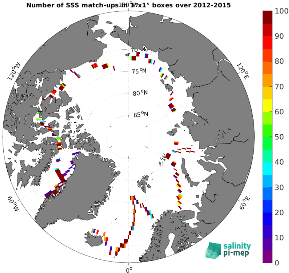
Figure 4: Number of SSS match-ups between TSG (GOSUD-Sailing-ship) SSS and the SMOS SSS L4 OI v342 - Weekly (CMEMS-CATDS-LOPS) SSS product for the Arctic Ocean Pi-MEP region over 1^\circ \times 1^\circ boxes and for the full satellite product period.
