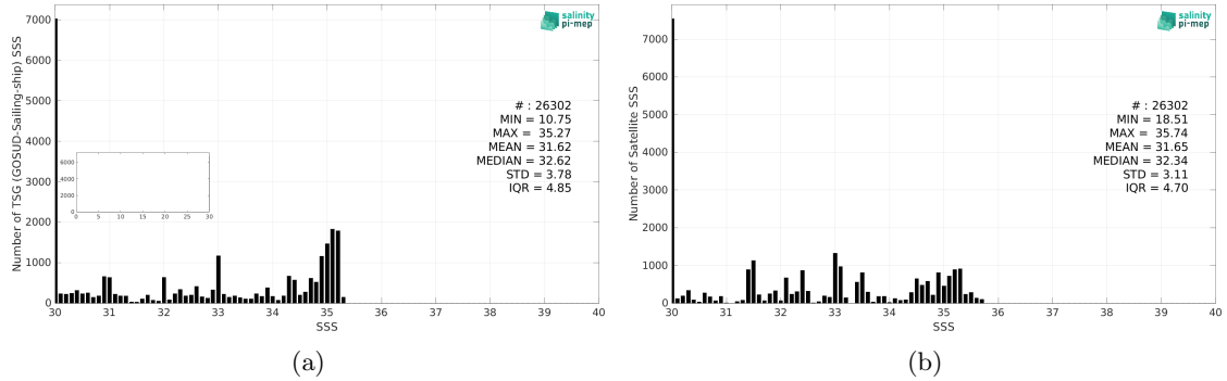
Figure 2: Histograms of SSS from TSG (GOSUD-Sailing-ship) (a) and SMOS SSS L4 OI v342 - Weekly (CMEMS-CATDS-LOPS) (b) considering all match-up pairs per bins of 0.1 over the Arctic Ocean Pi-MEP region and for the full satellite product period.
