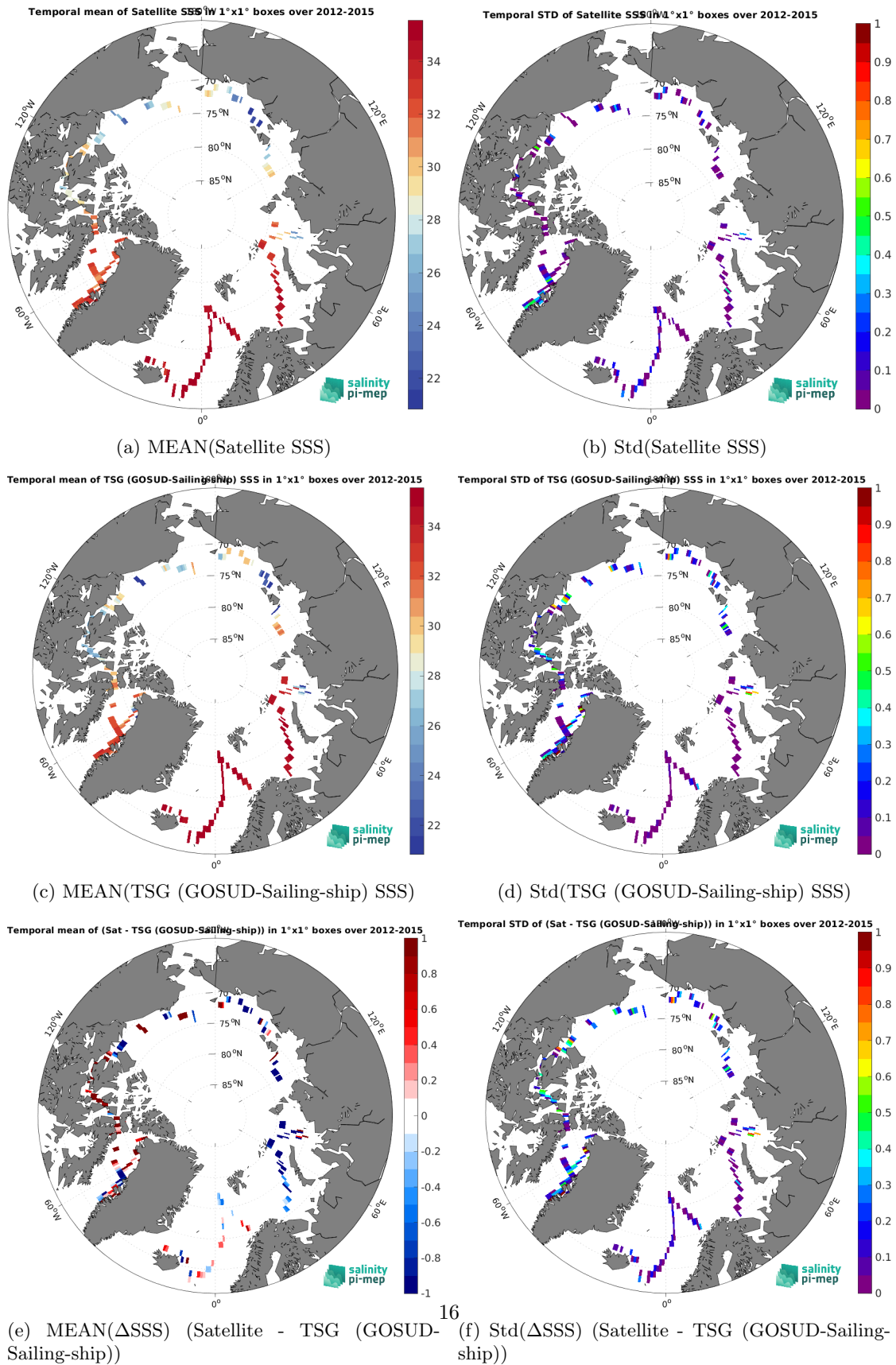
Figure 6: Temporal mean (left) and Std (right) of SSS from SMOS SSS L4 OI v342 - Weekly (CMEMS-CATDS-LOPS) (top), TSG (GOSUD-Sailing-ship) (middle), and of \Delta SSS (Satellite - TSG (GOSUD-Sailing-ship)). Only match-up pairs are used to generate these maps.
