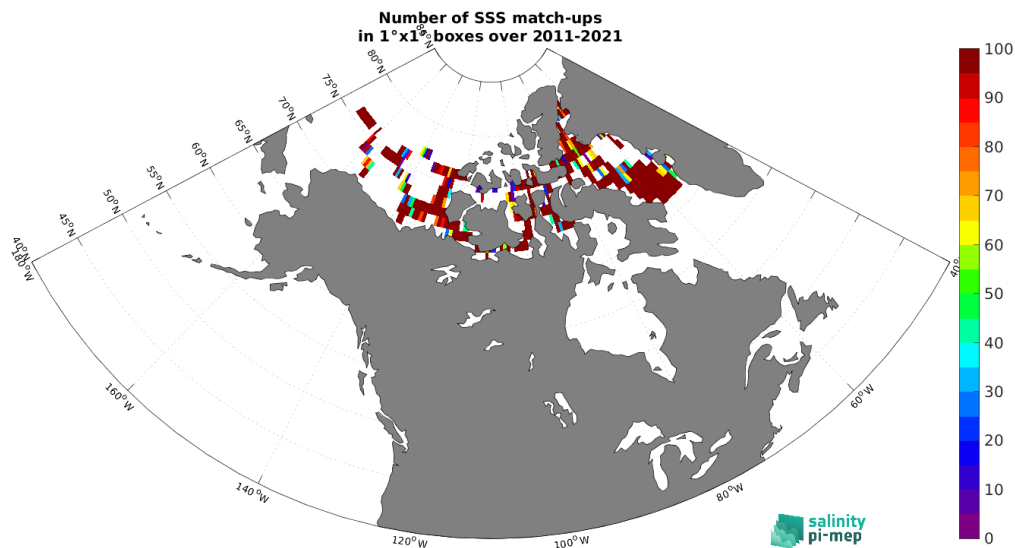
Figure 4: Number of SSS match-ups between TSG (Amundsen) SSS and the SMOS SSS L4 OI v342 - Weekly (CMEMS-CATDS-LOPS) SSS product for the Arctic Ocean Pi-MEP region over 1^\circ \times 1^\circ boxes and for the full satellite product period.
