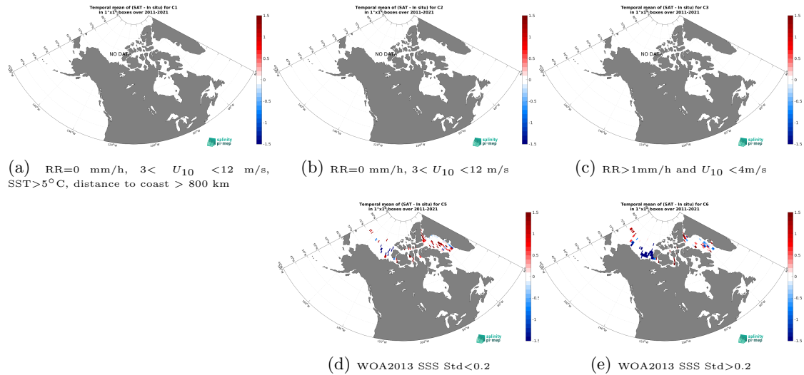
Figure 12: Temporal mean gridded over spatial boxes of size 1^{\circ}\times 1^{\circ} of \Delta\text{SSS} (SMOS SSS L4 OI v342 - Weekly (CMEMS-CATDS-LOPS) - TSG (Amundsen)) for 5 different subdatasets corresponding to:RR=0 mm/h, 3 < U_{10} < 12 m/s, SST >5^{\circ}\text{C} , distance to coast > 800 km (a), RR=0 mm/h, 3 < U_{10} < 12 m/s (b), RR >1 mm/h and U_{10} < 4 m/s (c), WOA2013 SSS Std <0.2 (d), WOA2013 SSS Std >0.2 (e).
