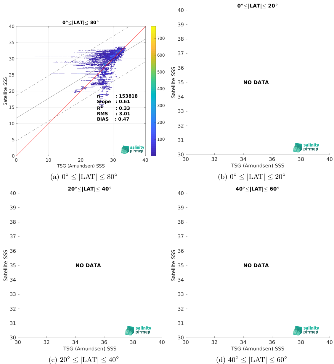
Figure 9: Contour maps of the concentration of SMOS SSS L4 OI v342 - Weekly (CMEMS-CATDS-LOPS) SSS (y-axis) versus TSG (Amundsen) SSS (x-axis) at match-up pairs for different latitude bands. For each plot, the red line shows x=y . The black thin and dashed lines indicate a linear fit through the data cloud and the \pm 95\% confidence levels, respectively. The number match-up pairs n , the slope and R^2 coefficient of the linear fit, the root mean square (RMS) and the mean bias between satellite and in situ data are indicated for each latitude band in each plots.
