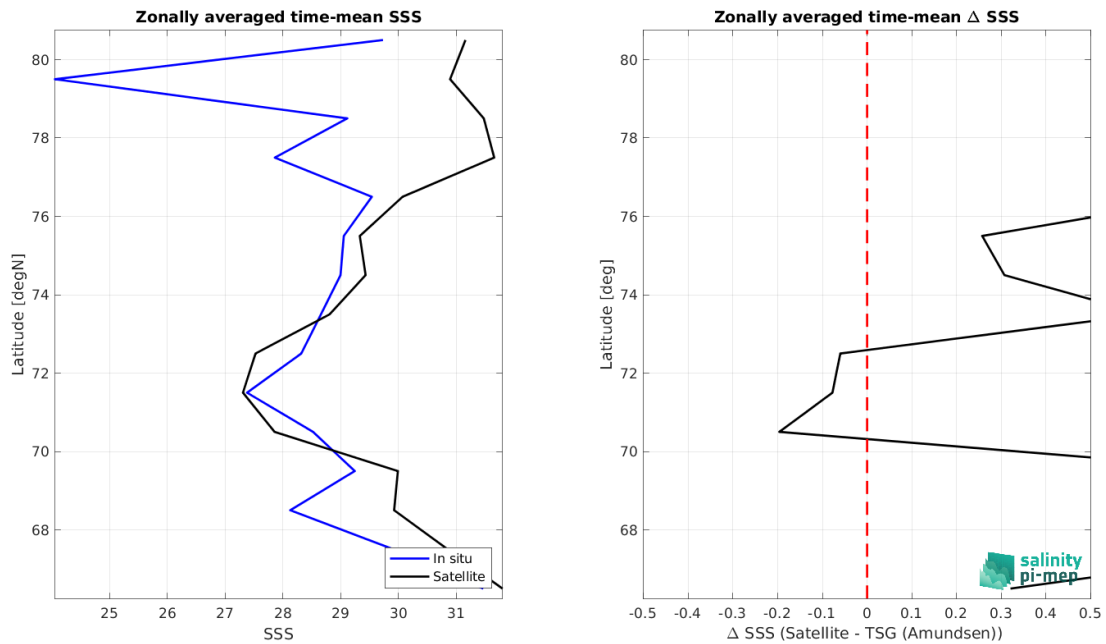
Figure 8: Left panel: Zonal mean SSS from SMOS SSS L4 OI v342 - Weekly (CMEMS-CATDS-LOPS) satellite product (black) and from TSG (Amundsen) (blue). Right panel: Zonal mean of \Delta SSS (Satellite - TSG (Amundsen)) for all the collected Pi-MEP match-up pairs estimated over the full satellite product period.
