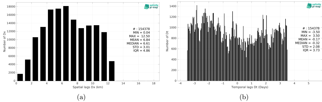
Figure 5: Histograms of the spatial (a) and temporal (b) lags between the location/time of the TSG (Amundsen) measurement and the date of the corresponding SMOS SSS L4 OI v342 - Weekly (CMEMS-CATDS-LOPS) SSS pixel.
