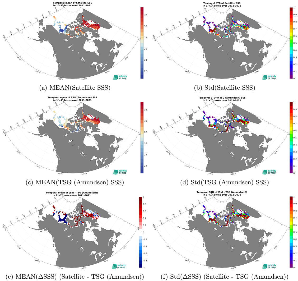
Figure 6: Temporal mean (left) and Std (right) of SSS from SMOS SSS L4 OI v342 - Weekly (CMEMS-CATDS-LOPS) (top), TSG (Amundsen) (middle), and of \Delta SSS (Satellite - TSG (Amundsen)). Only match-up pairs are used to generate these maps.
