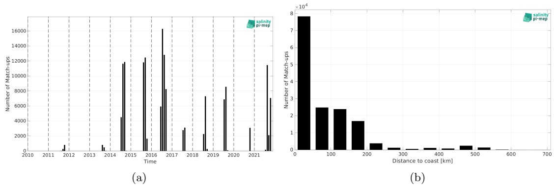
Figure 1: Number of match-ups between TSG (Amundsen) and SMOS SSS L4 OI v342 - Weekly (CMEMS-CATDS-LOPS) SSS as a function of time (a) and as function of the distance to coast (b) over the Arctic Ocean Pi-MEP region and for the full satellite product period.
