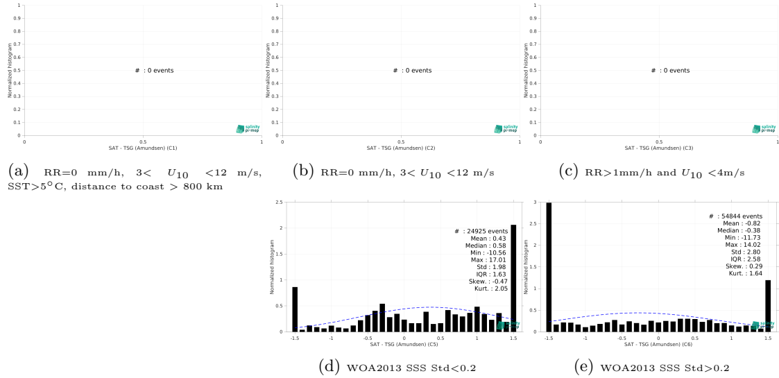
Figure 13: Normalized histogram of \Delta SSS (SMOS SSS L4 OI v342 - Weekly (CMEMS-CATDS-LOPS) - TSG (Amundsen)) for 5 different subdatasets corresponding to: RR=0 mm/h, 3 < U_{10} < 12 m/s, SST > 5°C, distance to coast > 800 km (a), RR=0 mm/h, 3 < U_{10} < 12 m/s (b), RR > 1mm/h and U_{10} < 4 m/s (c), WOA2013 SSS Std < 0.2 (d), WOA2013 SSS Std > 0.2 (e).
