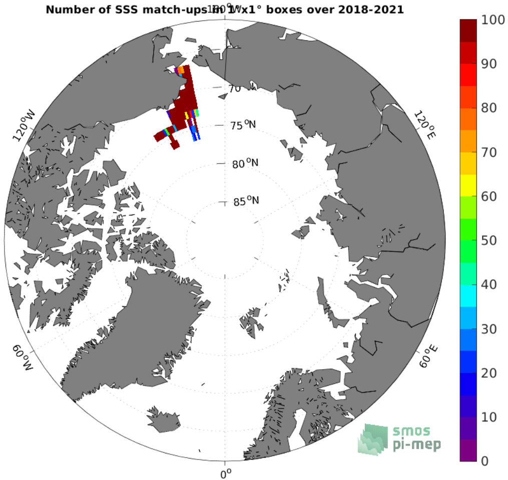
Figure 4: Number of SSS match-ups between Saildrone SSS and the SMOS SSS L4 OI v342 - Weekly (CMEMS-CATDS-LOPS) SSS product for the Arctic Ocean Pi-MEP region over 1^{\circ} \times 1^{\circ} boxes and for the full satellite product period.
