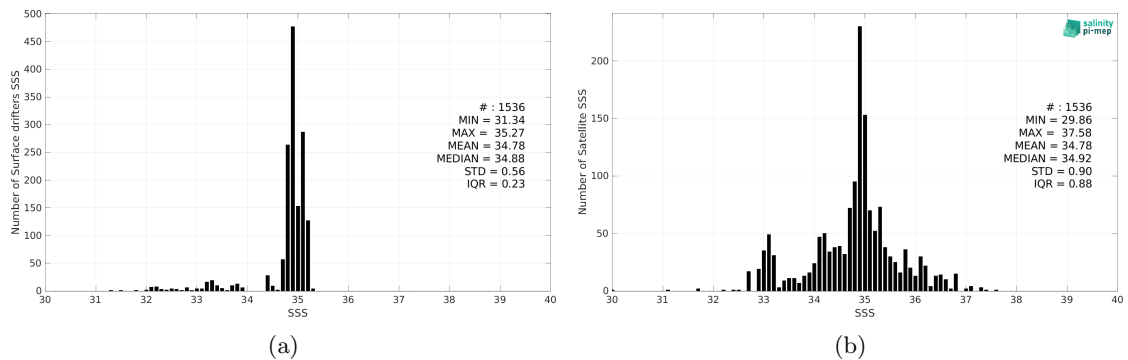
Figure 2: Histograms of SSS from Surface drifters (a) and SMOS SSS L4 OI v342 - Weekly (CMEMS-CATDS-LOPS) (b) considering all match-up pairs per bins of 0.1 over the Arctic Ocean Pi-MEP region and for the full satellite product period.
