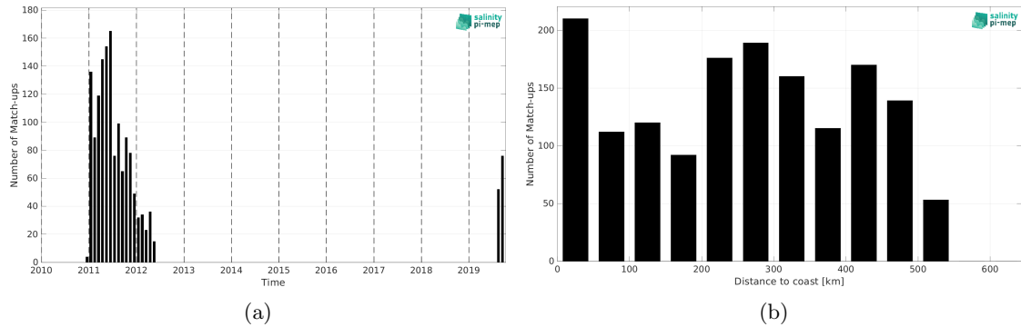
Figure 1: Number of match-ups between Surface drifters and SMOS SSS L4 OI v342 - Weekly (CMEMS-CATDS-LOPS) SSS as a function of time (a) and as function of the distance to coast (b) over the Arctic Ocean Pi-MEP region and for the full satellite product period.
