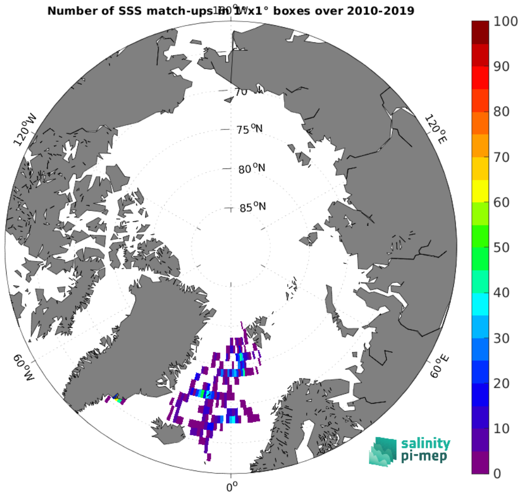
Figure 3: Number of SSS match-ups between Surface drifters SSS and the SMOS SSS L4 OI v342 - Weekly (CMEMS-CATDS-LOPS) SSS product for the Arctic Ocean Pi-MEP region over 1^\circ \times 1^\circ boxes and for the full satellite product period.
