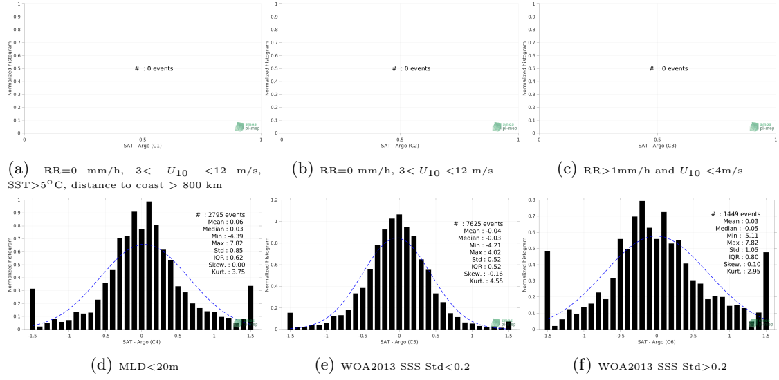
Figure 13: Normalized histogram of \Delta\text{SSS} (SMOS SSS L4 OI v342 - Weekly (CMEMS-CATDS-LOPS) - Argo) for 6 different subdatasets corresponding to: RR=0 mm/h, 3 < U_{10} < 12 m/s, SST > 5^{\circ}\text{C} , distance to coast > 800 km (a), RR=0 mm/h, 3 < U_{10} < 12 m/s (b), RR > 1\text{mm/h} and U_{10} < 4\text{m/s} (c), MLD < 20\text{m} (d), WOA2013 SSS Std < 0.2 (e), WOA2013 SSS Std > 0.2 (f).
