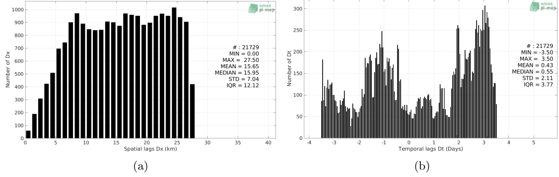
Figure 5: Histograms of the spatial (a) and temporal (b) lags between the location/time of the TSG (LEGOS-DM) measurement and the date of the corresponding SMOS L4 v2 Weekly (CATDS-CECOS-IFREMER) SSS pixel.
