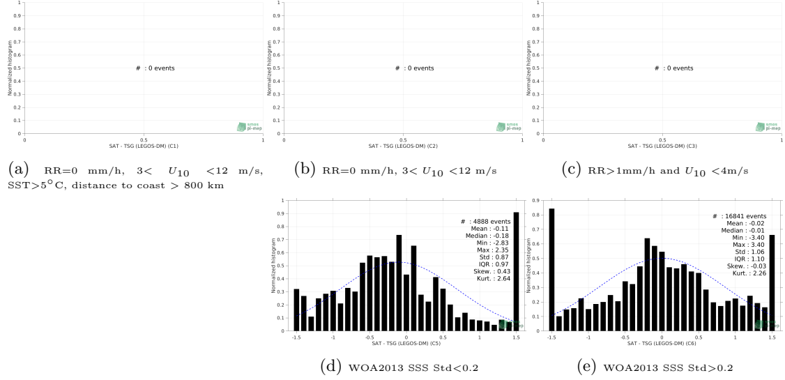
Figure 13: Normalized histogram of \Delta SSS (SMOS L4 v2 Weekly (CATDS-CECOS-IFREMER) - TSG (LEGOS-DM)) for 5 different subdatasets corresponding to: RR=0 mm/h, 3 < U_{10} < 12 m/s, SST>5°C, distance to coast > 800 km (a), RR=0 mm/h, 3 < U_{10} < 12 m/s (b), RR>1mm/h and U_{10} < 4 m/s (c), WOA2013 SSS Std<0.2 (d), WOA2013 SSS Std>0.2 (e).
