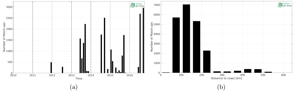
Figure 1: Number of match-ups between TSG (LEGOS-DM) and SMOS L4 v2 Weekly (CATDS-CECOS-IFREMER) SSS as a function of time (a) and as function of the distance to coast (b) over the Arctic Ocean Pi-MEP region and for the full satellite product period.
