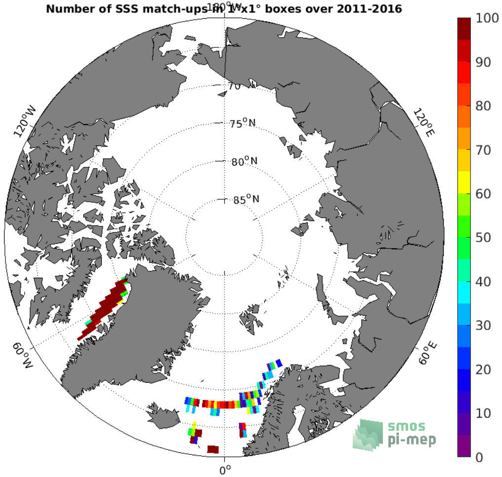
Figure 4: Number of SSS match-ups between TSG (LEGOS-DM) SSS and the SMOS L4 v2 Weekly (CATDS-CECOS-IFREMER) SSS product for the Arctic Ocean Pi-MEP region over 1^\circ \times 1^\circ boxes and for the full satellite product period.
