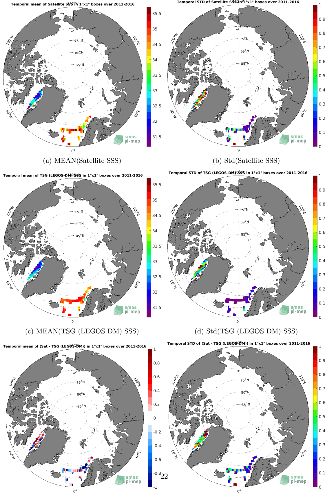
Figure 6: Temporal mean (left) and Std (right) of SSS from SMOS L4 v2 Weekly (CATDS-CECOS-IFREMER) (top), TSG (LEGOS-DM) (middle), and of \Delta SSS (Satellite - TSG (LEGOS-DM)). Only match-up pairs are used to generate these maps.
