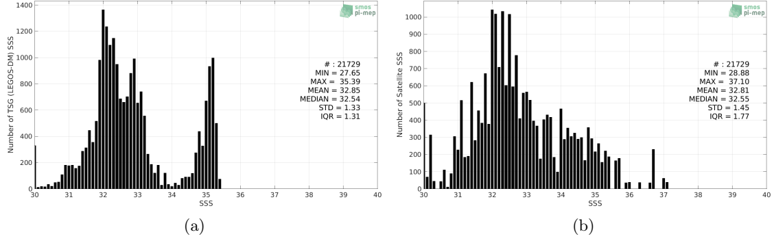
Figure 2: Histograms of SSS from TSG (LEGOS-DM) (a) and SMOS L4 v2 Weekly (CATDS-CECOS-IFREMER) (b) considering all match-up pairs per bins of 0.1 over the Arctic Ocean Pi-MEP region and for the full satellite product period.
