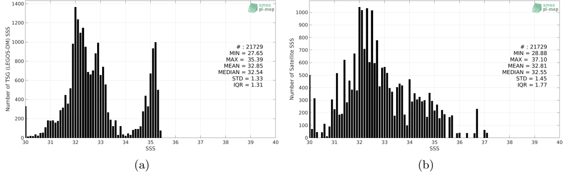
Figure 2: Histograms of SSS from TSG (LEGOS-DM) (a) and SMOS L4 v2 Weekly (CATDS-CECOS-IFREMER) (b) considering all match-up pairs per bins of 0.1 over the Arctic Ocean Pi-MEP region and for the full satellite product period.
