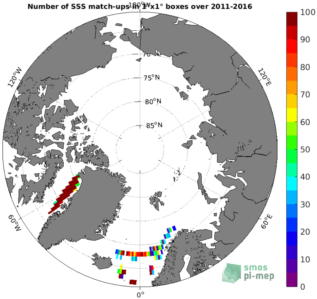
Figure 4: Number of SSS match-ups between TSG (LEGOS-DM) SSS and the SMOS L4 v2 Weekly (CATDS-CECOS-IFREMER) SSS product for the Arctic Ocean Pi-MEP region over 1°x1° boxes and for the full satellite product period.
