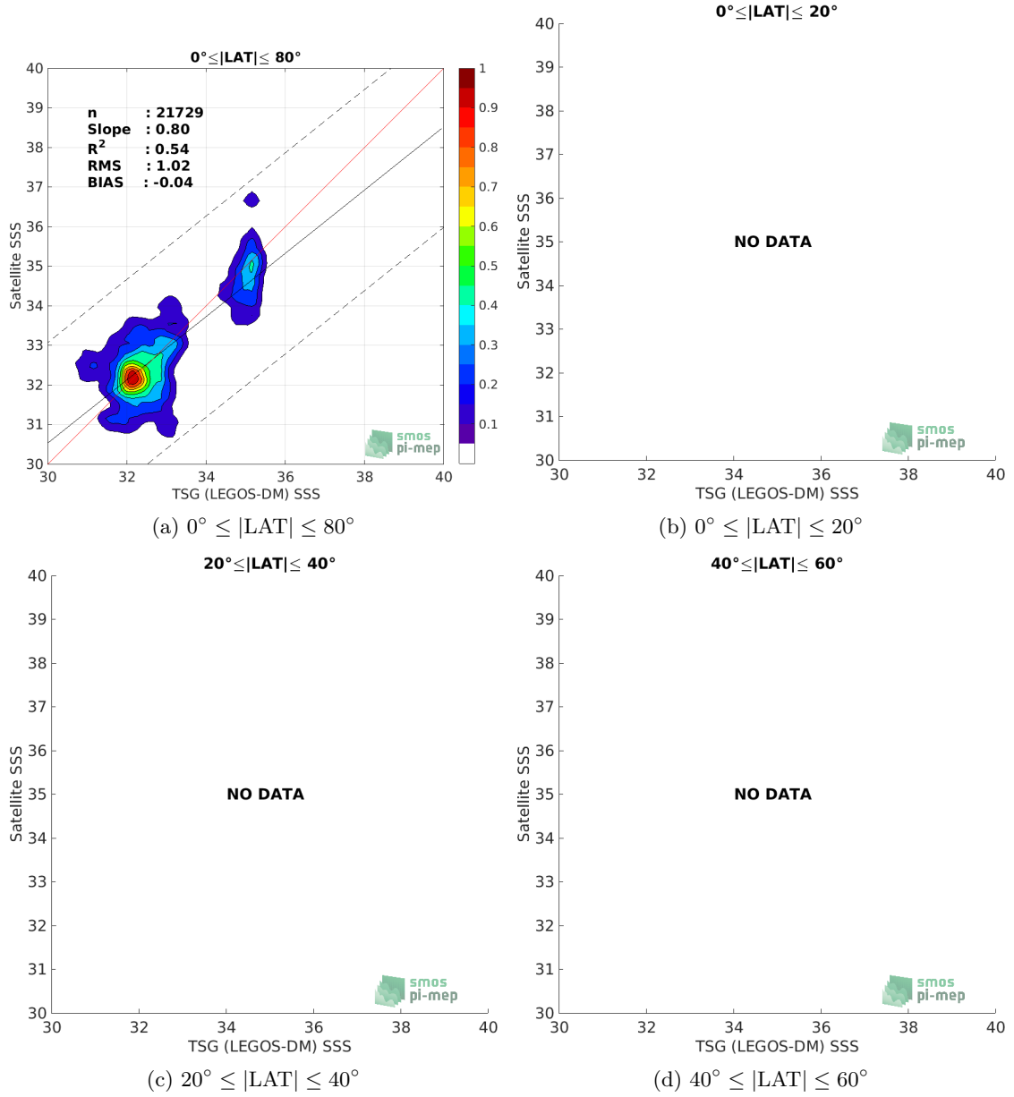
Figure 9: Contour maps of the concentration of SMOS L4 v2 Weekly (CATDS-CECOS-IFREMER) SSS (y-axis) versus TSG (LEGOS-DM) SSS (x-axis) at match-up pairs for different latitude bands. For each plot, the red line shows x=y . The black thin and dashed lines indicate a linear fit through the data cloud and the \pm 95\% confidence levels, respectively. The number match-up pairs n , the slope and R^2 coefficient of the linear fit, the root mean square (RMS) and the mean bias between satellite and in situ data are indicated for each latitude band in each plots.
