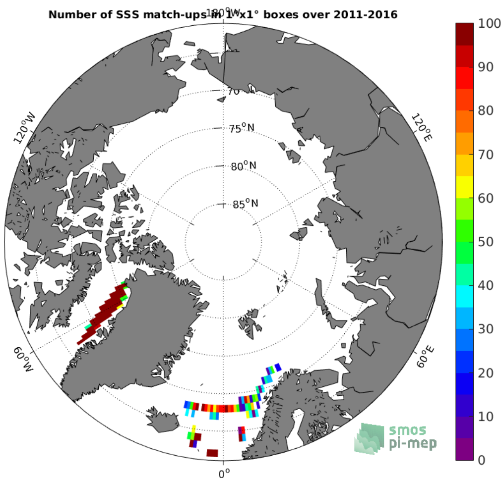
Figure 4: Number of SSS match-ups between TSG-LEGOS-DM SSS and the SMOS-L4-CATDS-CECOS-IFREMER-V2-WEEKLY-0.5DEG SSS product for the Arctic Ocean Pi-MEP region over 1^\circ \times 1^\circ boxes and for the full satellite product period.
