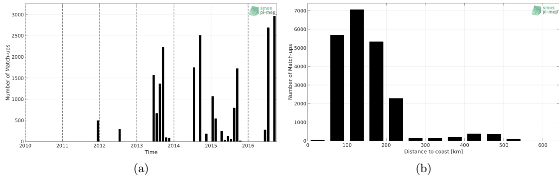
Figure 1: Number of match-ups between TSG-LEGOS-DM and SMOS-L4-CATDS-CECOS-IFREMER-V2-WEEKLY-0.5DEG SSS as a function of time (a) and as function of the distance to coast (b) over the Arctic Ocean Pi-MEP region and for the full satellite product period.
