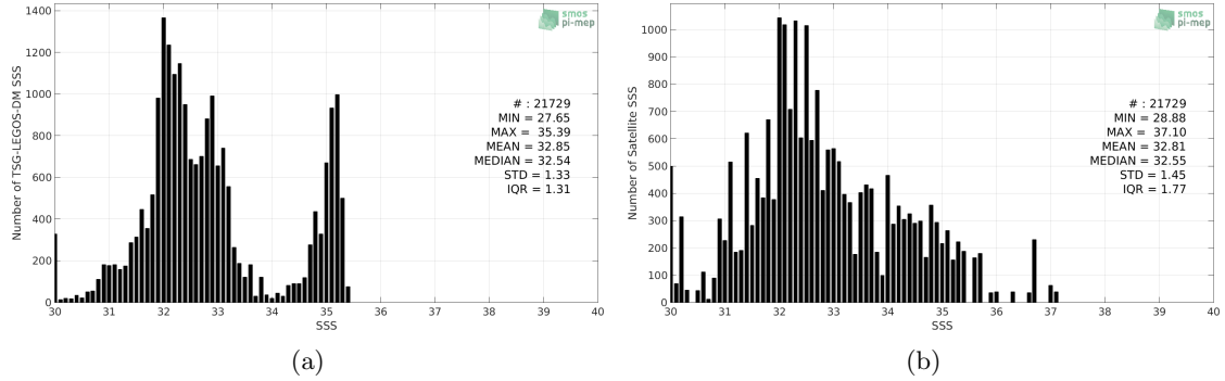
Figure 2: Histograms of SSS from TSG-LEGOS-DM (a) and SMOS-L4-CATDS-CECOS-IFREMER-V2-WEEKLY-0.5DEG (b) considering all match-up pairs per bins of 0.1 over the Arctic Ocean Pi-MEP region and for the full satellite product period.
