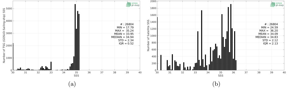
Figure 2: Histograms of SSS from TSG (GOSUD-Sailing-ship) (a) and SMOS L4 v2 Weekly (CATDS-CECOS-IFREMER) (b) considering all match-up pairs per bins of 0.1 over the Arctic Ocean Pi-MEP region and for the full satellite product period.
