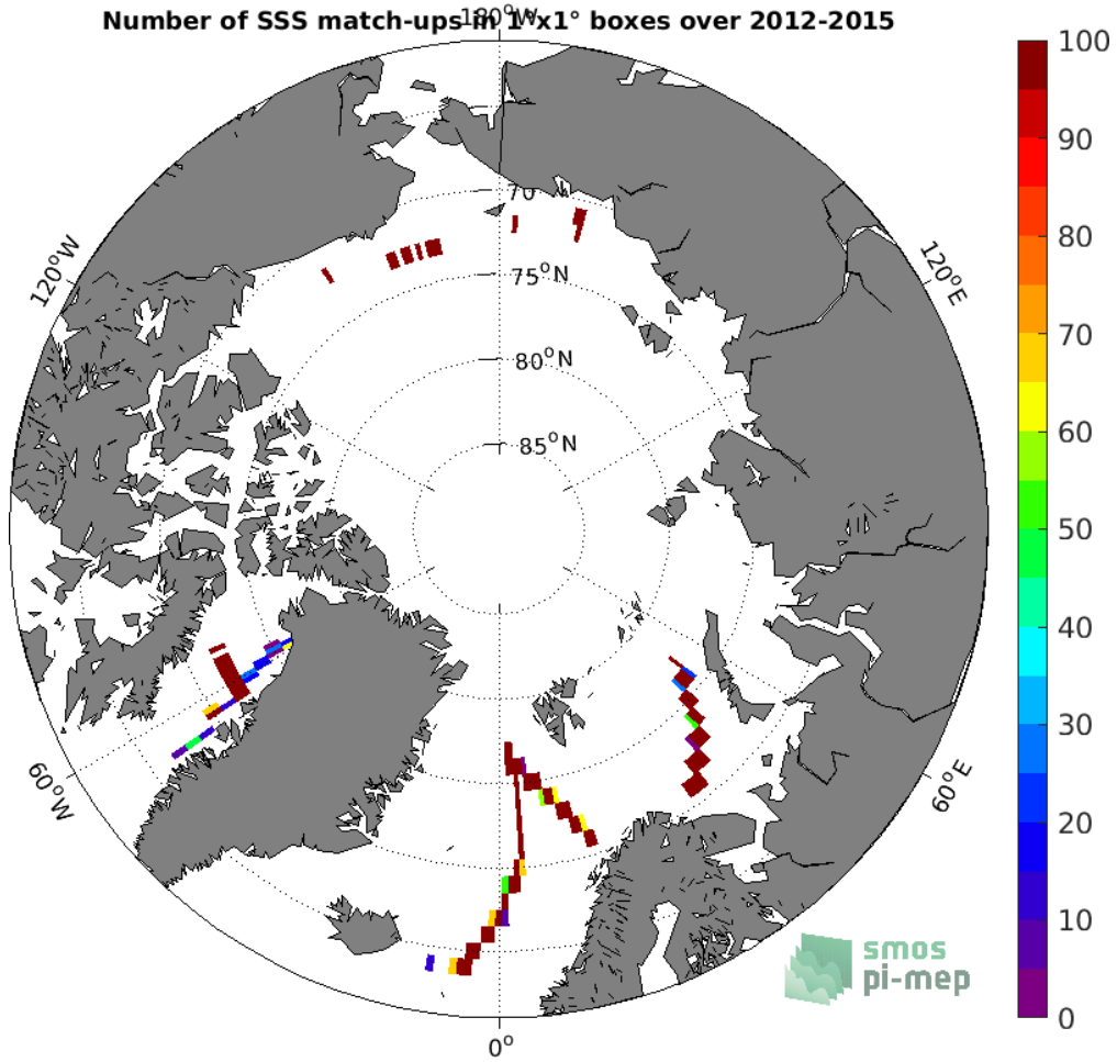
Figure 4: Number of SSS match-ups between TSG (GOSUD-Sailing-ship) SSS and the SMOS L4 v2 Weekly (CATDS-CECOS-IFREMER) SSS product for the Arctic Ocean Pi-MEP region over 1^\circ \times 1^\circ boxes and for the full satellite product period.
