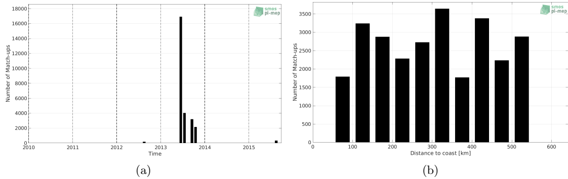
Figure 1: Number of match-ups between TSG (GOSUD-Sailing-ship) and SMOS L4 v2 Weekly (CATDS-CECOS-IFREMER) SSS as a function of time (a) and as function of the distance to coast (b) over the Arctic Ocean Pi-MEP region and for the full satellite product period.
