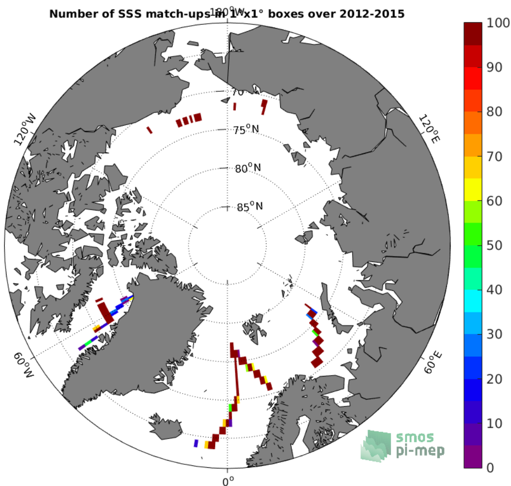
Figure 4: Number of SSS match-ups between TSG-GOSUD-Sailing-ship SSS and the SMOS-L4-CATDS-CECOS-IFREMER-V2-WEEKLY-0.5DEG SSS product for the Arctic Ocean Pi-MEP region over 1°x1° boxes and for the full satellite product period.
