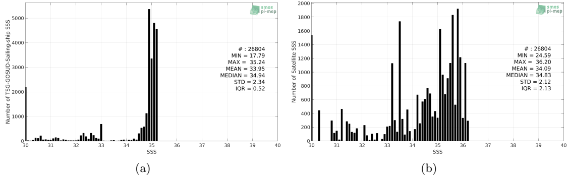
Figure 2: Histograms of SSS from TSG-GOSUD-Sailing-ship (a) and SMOS-L4-CATDS-CECOS-IFREMER-V2-WEEKLY-0.5DEG (b) considering all match-up pairs per bins of 0.1 over the Arctic Ocean Pi-MEP region and for the full satellite product period.
