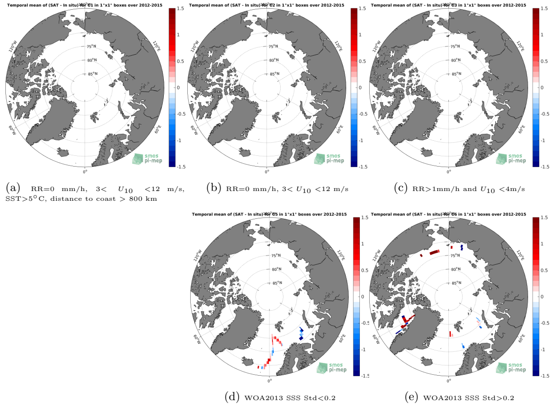
Figure 12: Temporal mean gridded over spatial boxes of size 1°x1° of \Delta SSS (SMOS-L4-CATDS-CECOS-IFREMER-V2-WEEKLY-0.5DEG - TSG-GOSUD-Sailing-ship) for 5 different subdatasets corresponding to: RR=0 mm/h, 3 < U_{10} < 12 m/s, SST > 5^\circ\text{C} , distance to coast > 800 km (a), RR=0 mm/h, 3 < U_{10} < 12 m/s (b), RR > 1 mm/h and U_{10} < 4 m/s (c), WOA2013 SSS Std < 0.2 (d), WOA2013 SSS Std > 0.2 (e).
