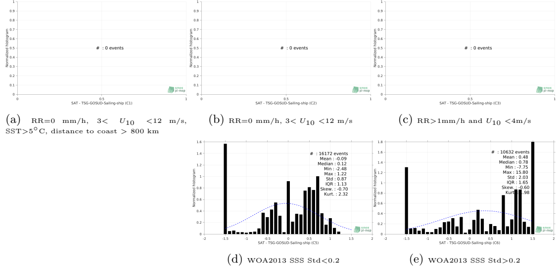
Figure 13: Normalized histogram of \Delta\text{SSS} (SMOS-L4-CATDS-CECOS-IFREMER-V2-WEEKLY-0.5DEG - TSG-GOSUD-Sailing-ship) for 5 different subdatasets corresponding to: RR=0 mm/h, 3 < U_{10} < 12 m/s, SST > 5^\circ\text{C} , distance to coast > 800 km (a), RR=0 mm/h, 3 < U_{10} < 12 m/s (b), RR > 1\text{mm/h} and U_{10} < 4\text{m/s} (c), WOA2013 SSS Std<0.2 (d), WOA2013 SSS Std>0.2 (e).
