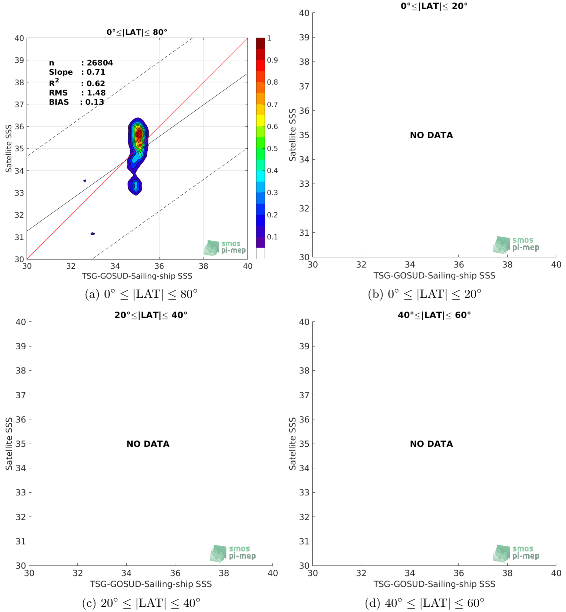
Figure 9: Contour maps of the concentration of SMOS-L4-CATDS-CECOS-IFREMER-V2-WEEKLY-0.5DEG SSS (y-axis) versus TSG-GOSUD-Sailing-ship SSS (x-axis) at match-up pairs for different latitude bands. For each plot, the red line shows x=y . The black thin and dashed lines indicate a linear fit through the data cloud and the \pm 95\% confidence levels, respectively. The number match-up pairs n , the slope and R^2 coefficient of the linear fit, the root mean square (RMS) and the mean bias between satellite and in situ data are indicated for each latitude band in each plots.
