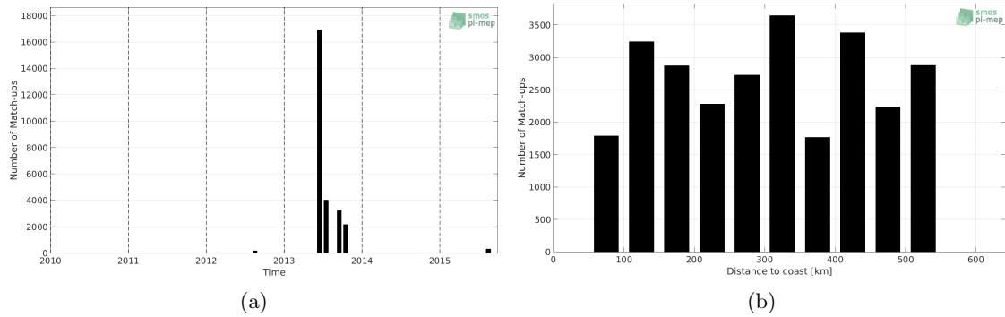
Figure 1: Number of match-ups between TSG-GOSUD-Sailing-ship and SMOS-L4-CATDS-CECOS-IFREMER-V2-WEEKLY-0.5DEG SSS as a function of time (a) and as function of the distance to coast (b) over the Arctic Ocean Pi-MEP region and for the full satellite product period.
