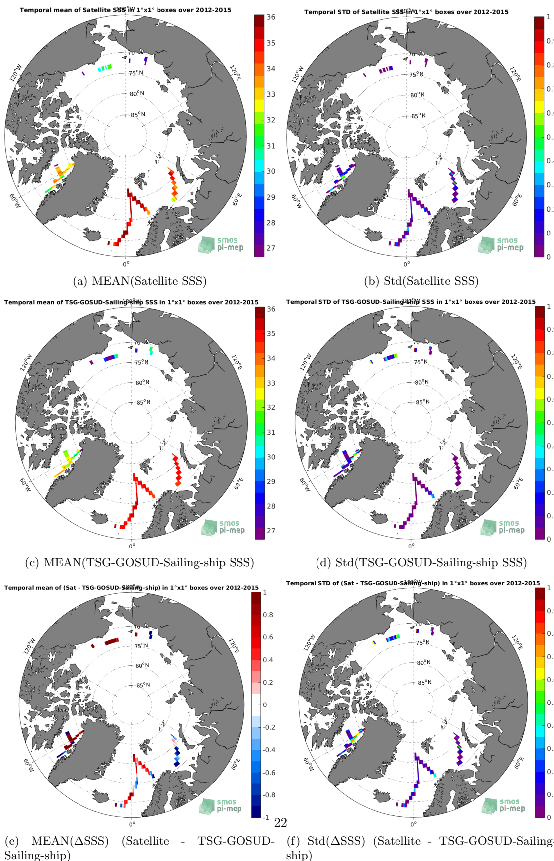
Figure 6: Temporal mean (left) and Std (right) of SSS from SMOS-L4-CATDS-CECOS-IFREMER-V2-WEEKLY-0.5DEG (top), TSG-GOSUD-Sailing-ship (middle), and of ΔSSS (Satellite - TSG-GOSUD-Sailing-ship). Only match-up pairs are used to generate these maps.
