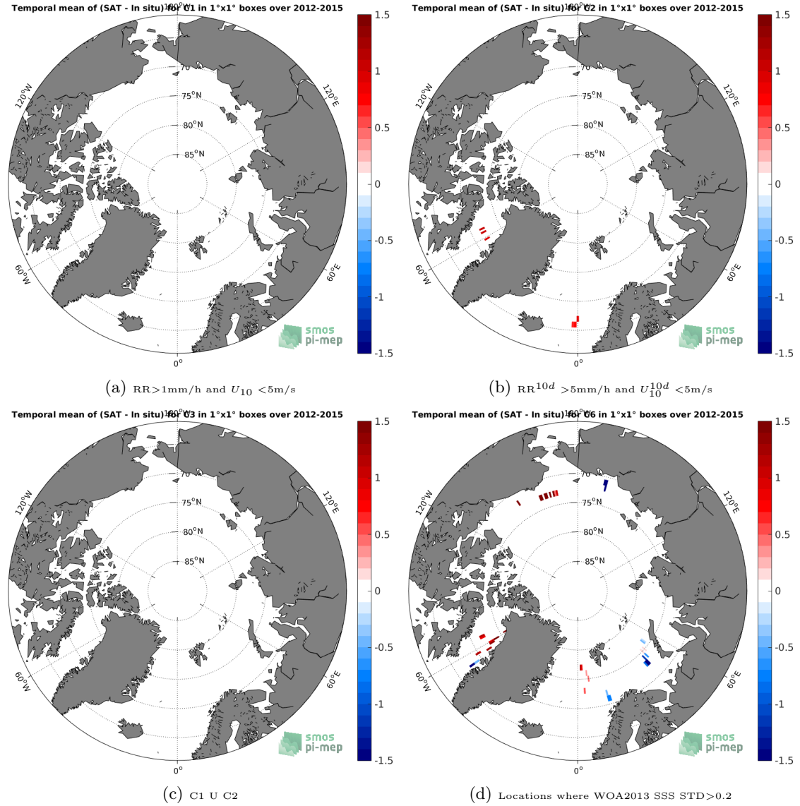
Figure 12: Temporal mean gridded over spatial boxes of size 1^\circ \times 1^\circ of \Delta SSS (SMOS-L4-CATDS-CECOS-IFREMER-V2-WEEKLY-0.5DEG - TSG-GOSUD-Sailing-ship) for 4 different subdatasets corresponding to: RR > 1\text{mm/h} and U_{10} < 5\text{m/s} (a), RR^{10d} > 5\text{mm/h} and U_{10}^{10d} < 5\text{m/s} (b), C1 U C2 (c), Locations where WOA2013 SSS STD > 0.2 (d).
