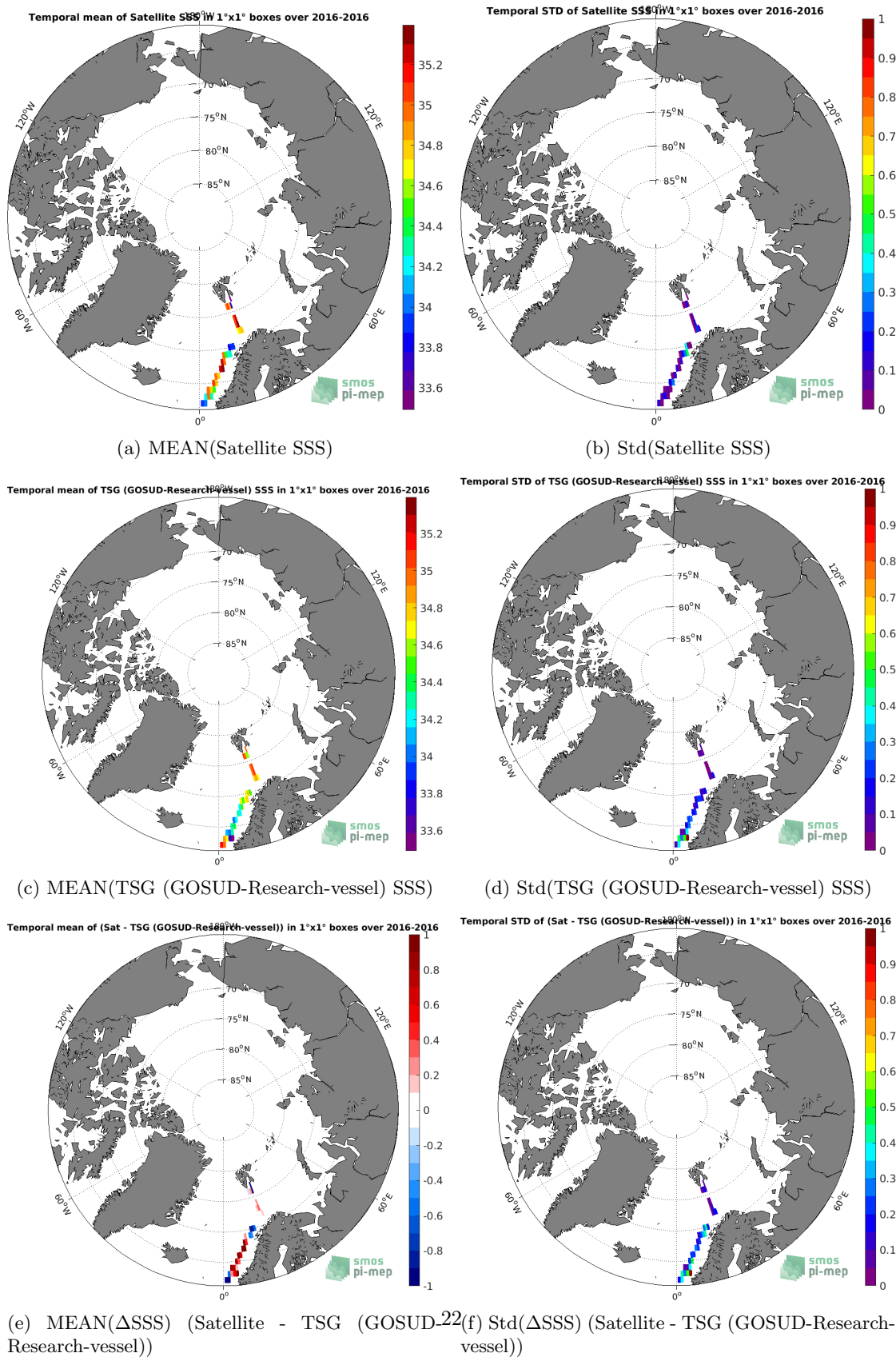
Figure 6: Temporal mean (left) and Std (right) of SSS from SMOS L4 v2 Weekly (CATDS-CECOS-IFREMER) (top), TSG (GOSUD-Research-vessel) (middle), and of \Delta SSS (Satellite - TSG (GOSUD-Research-vessel)). Only match-up pairs are used to generate these maps.
