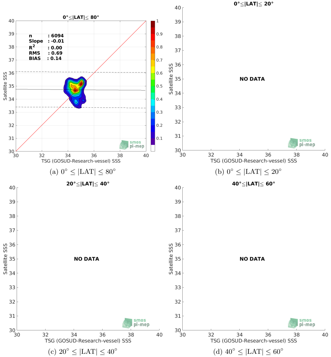
Figure 9: Contour maps of the concentration of SMOS L4 v2 Weekly (CATDS-CECOS-IFREMER) SSS (y-axis) versus TSG (GOSUD-Research-vessel) SSS (x-axis) at match-up pairs for different latitude bands. For each plot, the red line shows x=y . The black thin and dashed lines indicate a linear fit through the data cloud and the \pm 95\% confidence levels, respectively. The number match-up pairs n , the slope and R^2 coefficient of the linear fit, the root mean square (RMS) and the mean bias between satellite and in situ data are indicated for each latitude band in each plots.
