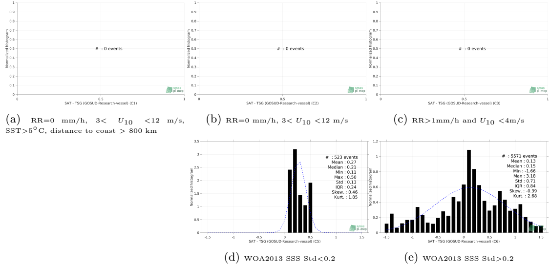
Figure 13: Normalized histogram of \Delta\text{SSS} (SMOS L4 v2 Weekly (CATDS-CECOS-IFREMER) - TSG (GOSUD-Research-vessel)) for 5 different subdatasets corresponding to: RR=0 mm/h, 3 < U_{10} < 12 m/s, SST > 5^\circ\text{C} , distance to coast > 800 km (a), RR=0 mm/h, 3 < U_{10} < 12 m/s (b), RR > 1\text{mm/h} and U_{10} < 4\text{m/s} (c), WOA2013 SSS Std<0.2 (d), WOA2013 SSS Std>0.2 (e).
