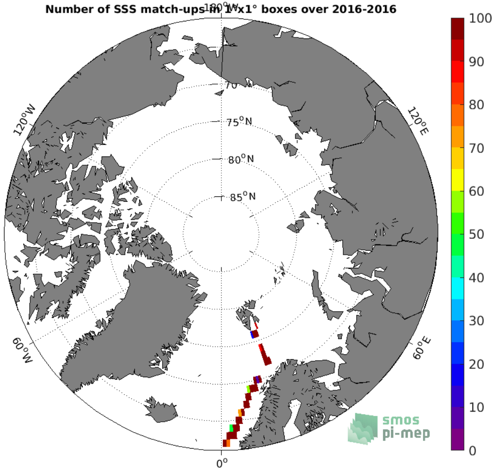
Figure 4: Number of SSS match-ups between TSG (GOSUD-Research-vessel) SSS and the SMOS L4 v2 Weekly (CATDS-CECOS-IFREMER) SSS product for the Arctic Ocean Pi-MEP region over 1°x1° boxes and for the full satellite product period.
