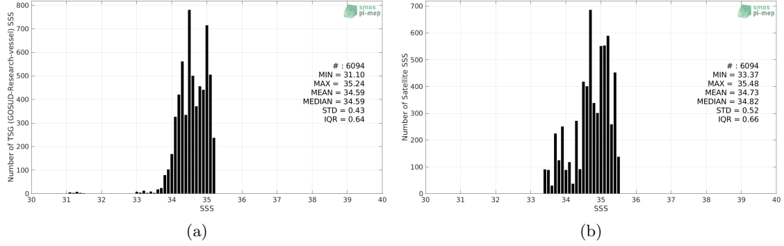
Figure 2: Histograms of SSS from TSG (GOSUD-Research-vessel) (a) and SMOS L4 v2 Weekly (CATDS-CECOS-IFREMER) (b) considering all match-up pairs per bins of 0.1 over the Arctic Ocean Pi-MEP region and for the full satellite product period.
