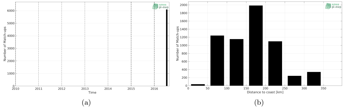
Figure 1: Number of match-ups between TSG (GOSUD-Research-vessel) and SMOS L4 v2 Weekly (CATDS-CECOS-IFREMER) SSS as a function of time (a) and as function of the distance to coast (b) over the Arctic Ocean Pi-MEP region and for the full satellite product period.
