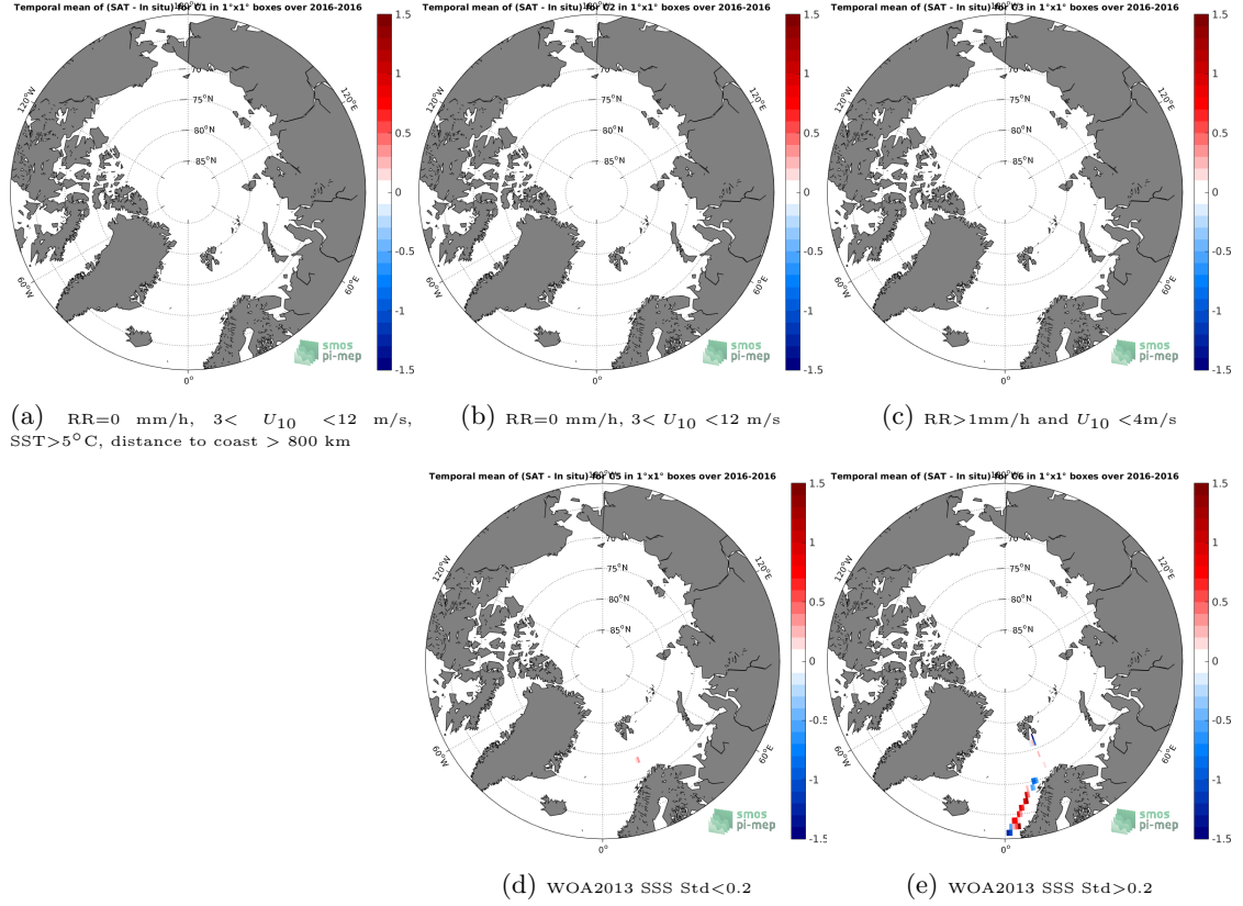
Figure 12: Temporal mean gridded over spatial boxes of size 1°x1° of \Delta SSS (SMOS-L4-CATDS-CECOS-IFREMER-V2-WEEKLY-0.5DEG - TSG-GOSUD-Research-vessel) for 5 different sub-datasets corresponding to: RR=0 mm/h, 3 < U_{10} < 12 m/s, SST > 5^\circ\text{C} , distance to coast > 800 km (a), RR=0 mm/h, 3 < U_{10} < 12 m/s (b), RR > 1 mm/h and U_{10} < 4 m/s (c), WOA2013 SSS Std < 0.2 (d), WOA2013 SSS Std > 0.2 (e).
