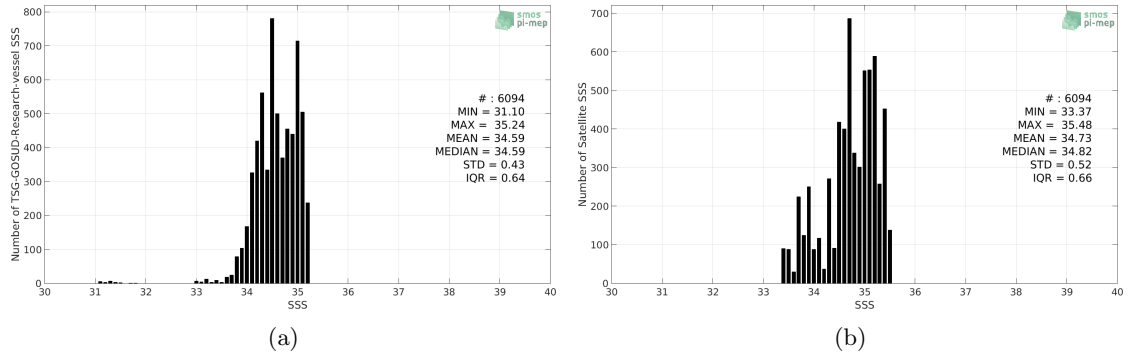
Figure 2: Histograms of SSS from TSG-GOSUD-Research-vessel (a) and SMOS-L4-CATDS-CECOS-IFREMER-V2-WEEKLY-0.5DEG (b) considering all match-up pairs per bins of 0.1 over the Arctic Ocean Pi-MEP region and for the full satellite product period.
