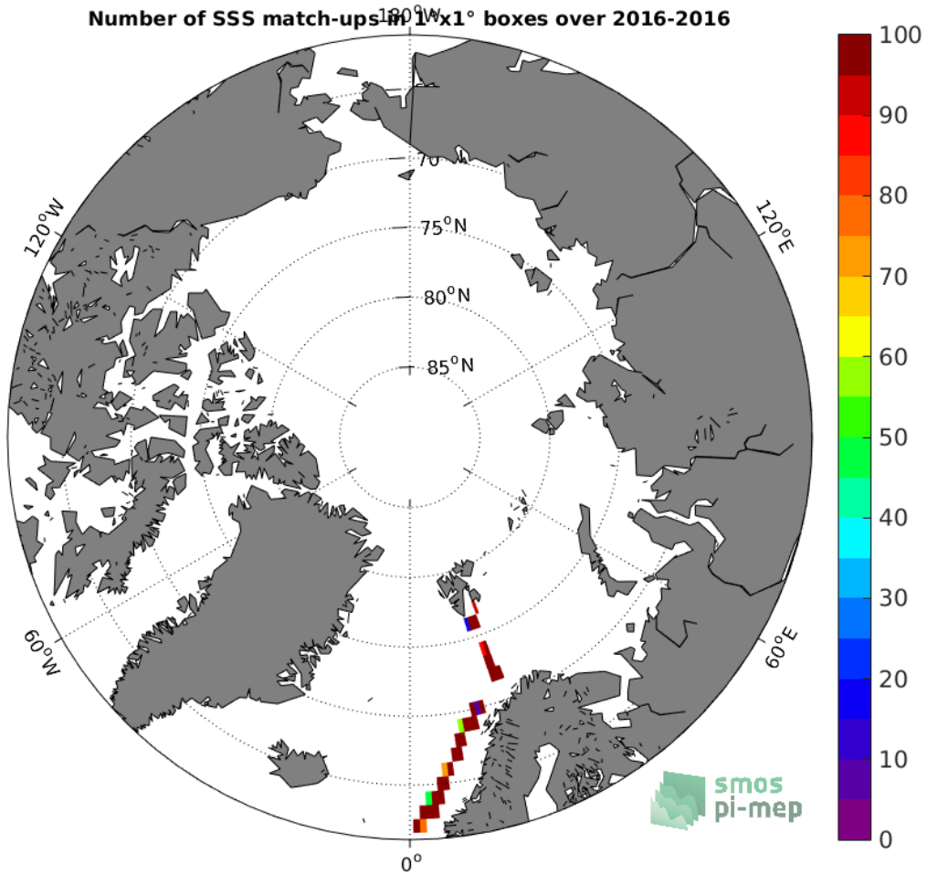
Figure 4: Number of SSS match-ups between TSG-GOSUD-Research-vessel SSS and the SMOS-L4-CATDS-CECOS-IFREMER-V2-WEEKLY-0.5DEG SSS product for the Arctic Ocean Pi-MEP region over 1^\circ \times 1^\circ boxes and for the full satellite product period.
