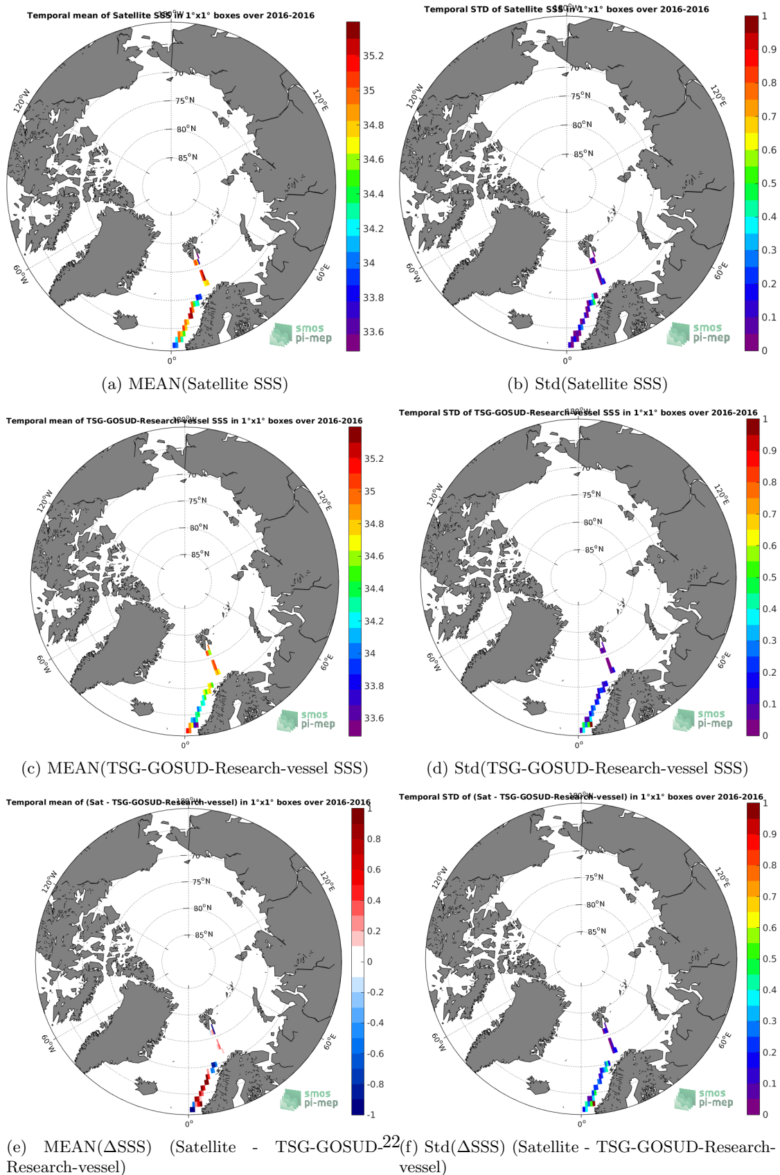
Figure 6: Temporal mean (left) and Std (right) of SSS from SMOS-L4-CATDS-CECOS-IFREMER-V2-WEEKLY-0.5DEG (top), TSG-GOSUD-Research-vessel (middle), and of \Delta SSS (Satellite - TSG-GOSUD-Research-vessel). Only match-up pairs are used to generate these maps.
