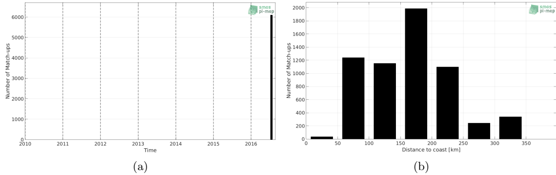
Figure 1: Number of match-ups between TSG-GOSUD-Research-vessel and SMOS-L4-CATDS-CECOS-IFREMER-V2-WEEKLY-0.5DEG SSS as a function of time (a) and as function of the distance to coast (b) over the Arctic Ocean Pi-MEP region and for the full satellite product period.
