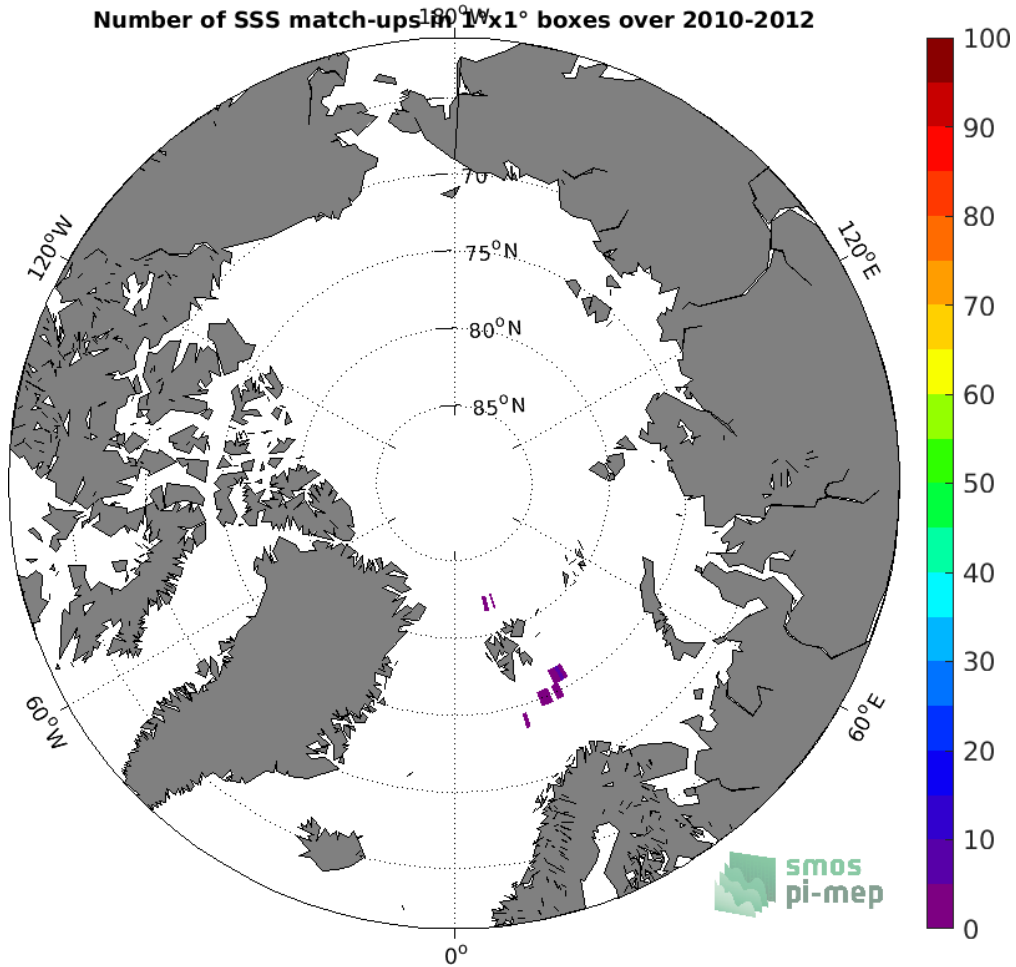
Figure 4: Number of SSS match-ups between Sea mammals SSS and the SMOS L4 v2 Weekly (CATDS-CECOS-IFREMER) SSS product for the Arctic Ocean Pi-MEP region over 1^\circ \times 1^\circ boxes and for the full satellite product period.
