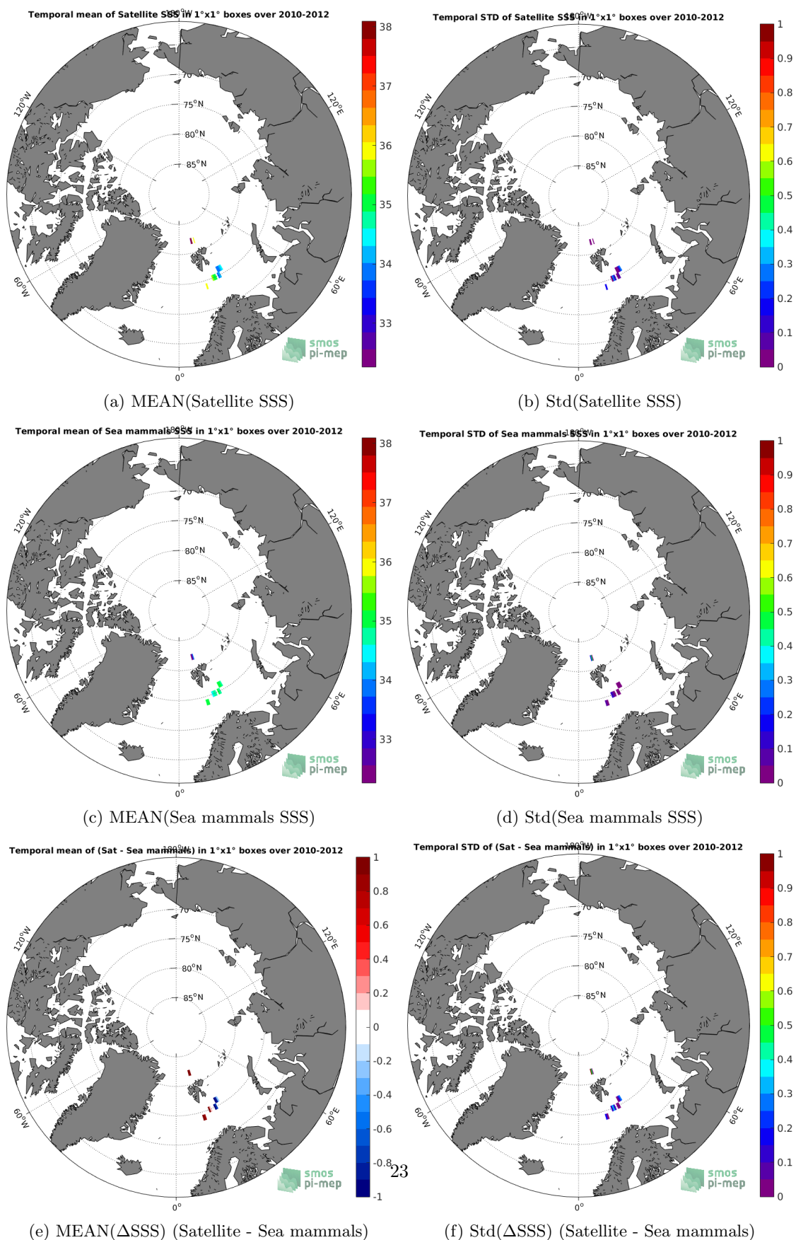
Figure 6: Temporal mean (left) and Std (right) of SSS from SMOS-L4-CATDS-CECOS-IFREMER-V2-WEEKLY-0.5DEG (top), Sea mammals (middle), and of \Delta SSS (Satellite - Sea mammals). Only match-up pairs are used to generate these maps.
