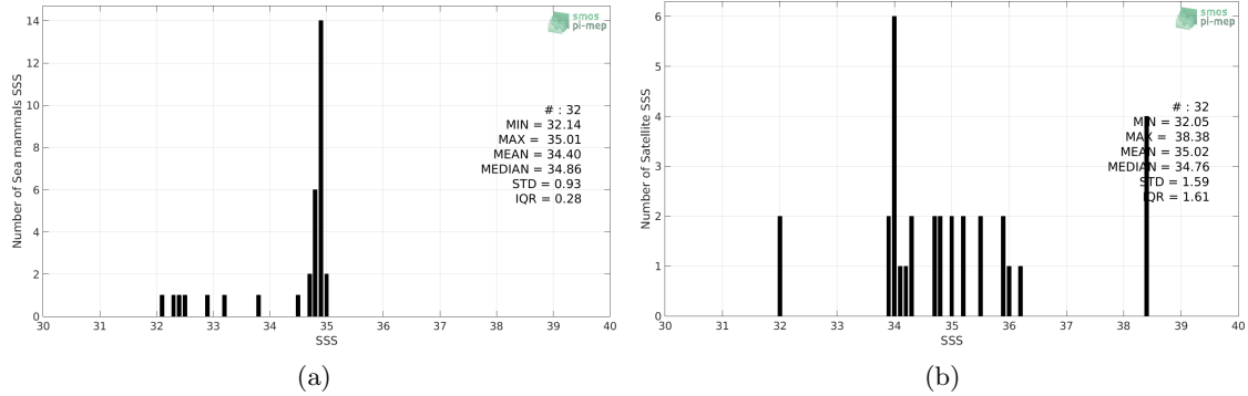
Figure 2: Histograms of SSS from Sea mammals (a) and SMOS-L4-CATDS-CECOS-IFREMER-V2-WEEKLY-0.5DEG (b) considering all match-up pairs per bins of 0.1 over the Arctic Ocean Pi-MEP region and for the full satellite product period.
