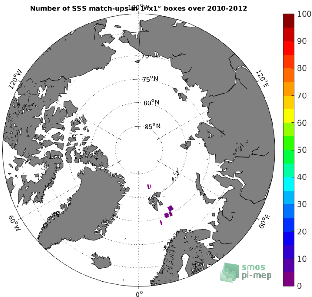
Figure 4: Number of SSS match-ups between Sea mammals SSS and the SMOS-L4-CATDS-CECOS-IFREMER-V2-WEEKLY-0.5DEG SSS product for the Arctic Ocean Pi-MEP region over 1^\circ \times 1^\circ boxes and for the full satellite product period.
