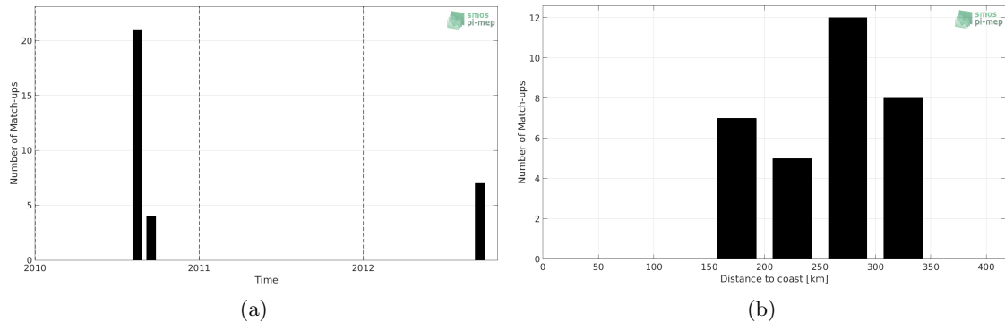
Figure 1: Number of match-ups between Sea mammals and SMOS-L4-CATDS-CECOS-IFREMER-V2-WEEKLY-0.5DEG SSS as a function of time (a) and as function of the distance to coast (b) over the Arctic Ocean Pi-MEP region and for the full satellite product period.
