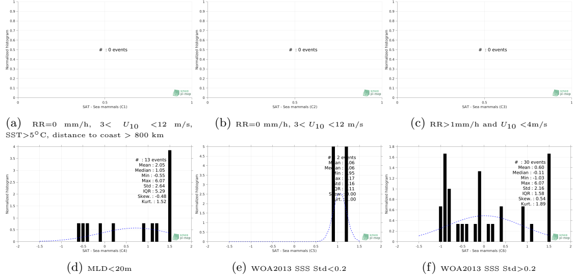
Figure 13: Normalized histogram of \Delta\text{SSS} (SMOS-L4-CATDS-CECOS-IFREMER-V2-WEEKLY-0.5DEG - Sea mammals) for 6 different subdatasets corresponding to: RR=0 mm/h, 3 < U_{10} < 12 m/s, SST > 5^\circ\text{C} , distance to coast > 800 km (a), RR=0 mm/h, 3 < U_{10} < 12 m/s (b), RR > 1 mm/h and U_{10} < 4 m/s (c), MLD < 20 m (d), WOA2013 SSS Std < 0.2 (e), WOA2013 SSS Std > 0.2 (f).
