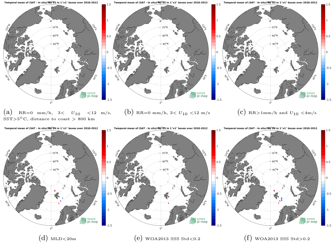
Figure 12: Temporal mean gridded over spatial boxes of size 1^{\circ}\times 1^{\circ} of \Delta\text{SSS} (SMOS-L4-CATDS-CECOS-IFREMER-V2-WEEKLY-0.5DEG - Sea mammals) for 6 different subdatasets corresponding to:RR=0 mm/h, 3 < U_{10} < 12 m/s, SST >5^{\circ}\text{C} , distance to coast > 800 km (a), RR=0 mm/h, 3 < U_{10} < 12 m/s (b), RR >1 mm/h and U_{10} < 4 m/s (c),MLD <20 m (d),WOA2013 SSS Std <0.2 (e),WOA2013 SSS Std >0.2 (f).
