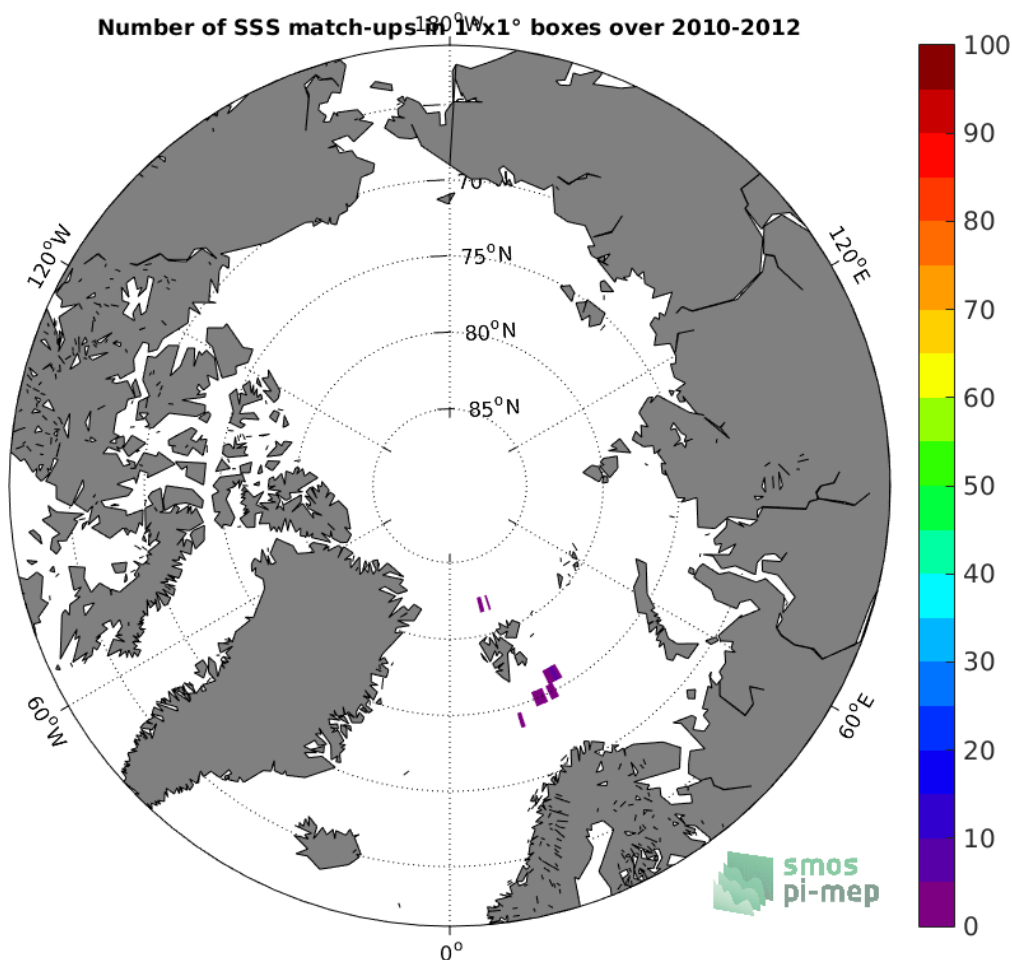
Figure 4: Number of SSS match-ups between Sea mammals SSS and the SMOS-L4-CATDS-CECOS-IFREMER-V2-WEEKLY-0.5DEG SSS product for the Arctic Ocean Pi-MEP region over 1°x1° boxes and for the full satellite product period.
