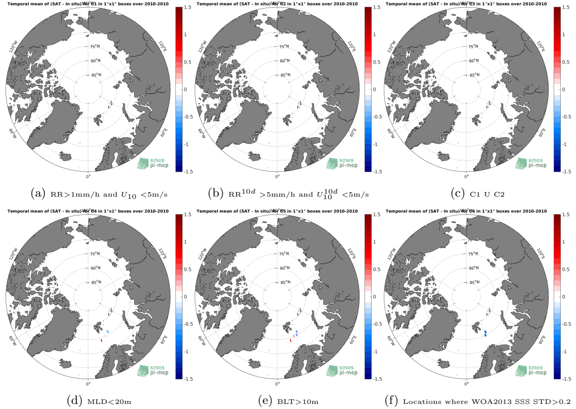
Figure 12: Temporal mean gridded over spatial boxes of size 1^\circ \times 1^\circ of \Delta\text{SSS} (SMOS-L4-CATDS-CECOS-IFREMER-V2-WEEKLY-0.5DEG - Sea mammals) for 6 different subdatasets corresponding to: \text{RR} > 1\text{mm/h} and U_{10} < 5\text{m/s} (a), \text{RR}^{10d} > 5\text{mm/h} and U_{10}^{10d} < 5\text{m/s} (b), C1 U C2 (c), \text{MLD} < 20\text{m} (d), \text{BLT} > 10\text{m} (e), Locations where WOA2013 SSS STD > 0.2 (f).
