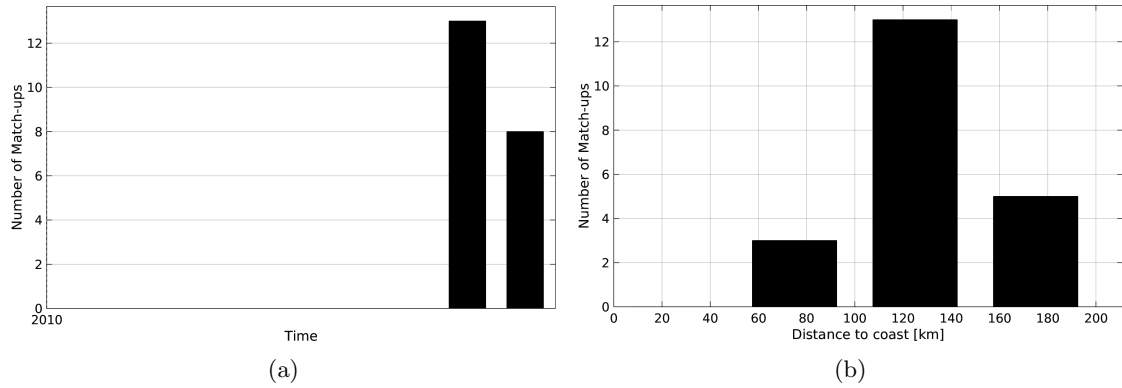
Figure 1: Number of match-ups between Sea mammals and SMOS-L4-CATDS-CECOS-IFREMER-V2-WEEKLY-0.5DEG SSS as a function of time (a) and as function of the distance to coast (b) over the Arctic Ocean Pi-MEP region and for the full satellite product period.
