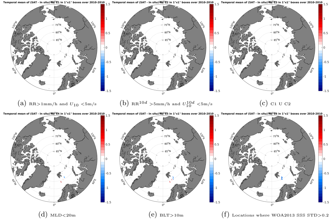
Figure 12: Temporal mean gridded over spatial boxes of size 1^\circ \times 1^\circ of \Delta SSS (SMOS-L4-CATDS-CECOS-IFREMER-V2-WEEKLY-0.5DEG - Sea mammals) for 6 different subdatasets corresponding to: RR > 1\text{mm/h} and U_{10} < 5\text{m/s} (a), RR^{10d} > 5\text{mm/h} and U_{10}^{10d} < 5\text{m/s} (b), C1 U C2 (c), MLD < 20\text{m} (d), BLT > 10\text{m} (e), Locations where WOA2013 SSS STD > 0.2 (f).
