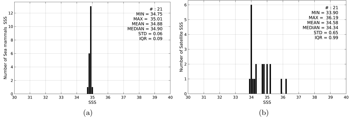
Figure 2: Histograms of SSS from Sea mammals (a) and SMOS-L4-CATDS-CECOS-IFREMER-V2-WEEKLY-0.5DEG (b) considering all match-up pairs per bins of 0.1 over the Arctic Ocean Pi-MEP region and for the full satellite product period.
