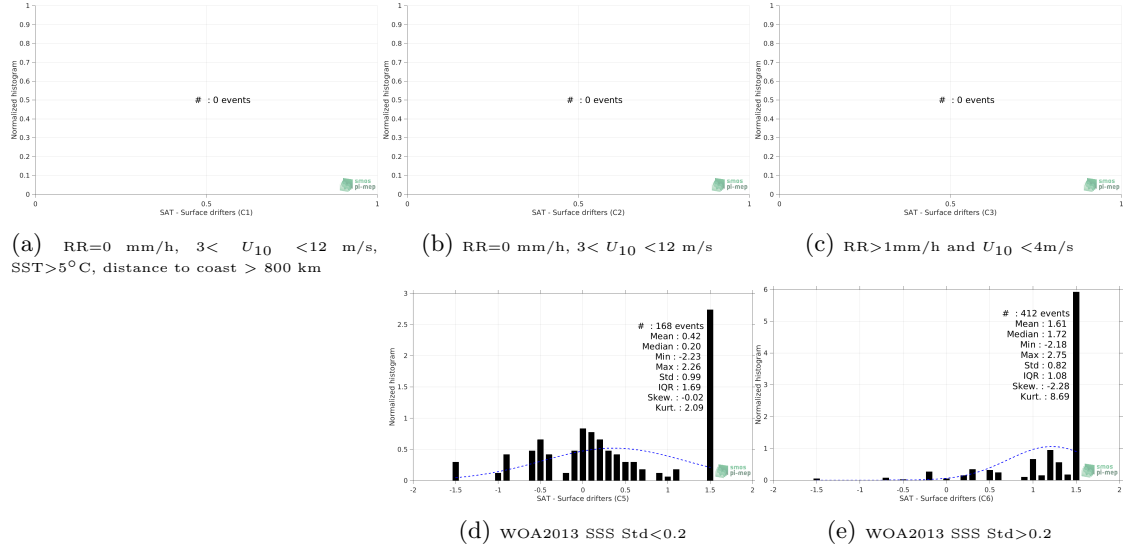
Figure 12: Normalized histogram of \Delta\text{SSS} (SMOS L4 v2 Weekly (CATDS-CECOS-IFREMER) - Surface drifters) for 5 different subdatasets corresponding to: RR=0 mm/h, 3 < U_{10} < 12 m/s, SST > 5^\circ\text{C} , distance to coast > 800 km (a), RR=0 mm/h, 3 < U_{10} < 12 m/s (b), RR > 1\text{mm/h} and U_{10} < 4\text{m/s} (c), WOA2013 SSS Std < 0.2 (d), WOA2013 SSS Std > 0.2 (e).
