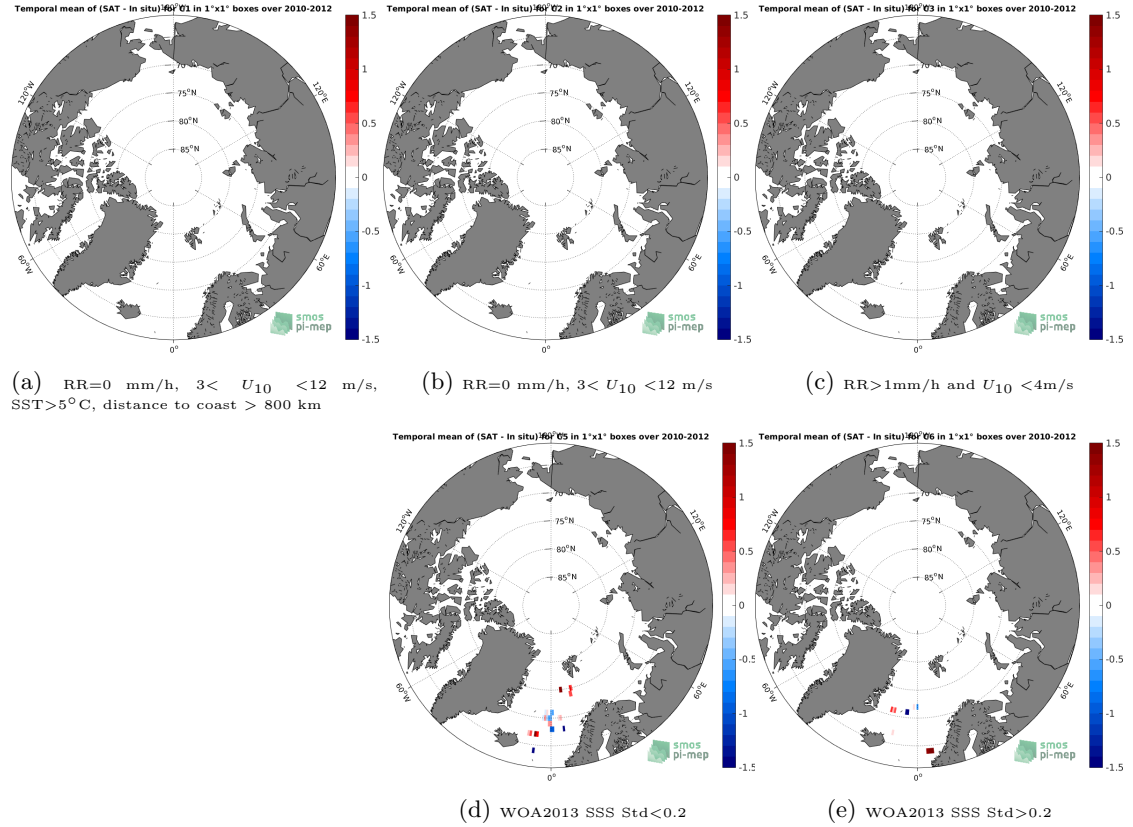
Figure 11: Temporal mean gridded over spatial boxes of size 1^{\circ}\times 1^{\circ} of \Delta\text{SSS} (SMOS-L4-CATDS-CECOS-IFREMER-V2-WEEKLY-0.5DEG - Surface drifters) for 5 different subdatasets corresponding to: RR=0 mm/h, 3 < U_{10} < 12 m/s, SST > 5^{\circ}\text{C} , distance to coast > 800 km (a), RR=0 mm/h, 3 < U_{10} < 12 m/s (b), RR > 1 mm/h and U_{10} < 4 m/s (c), WOA2013 SSS Std < 0.2 (d), WOA2013 SSS Std > 0.2 (e).
