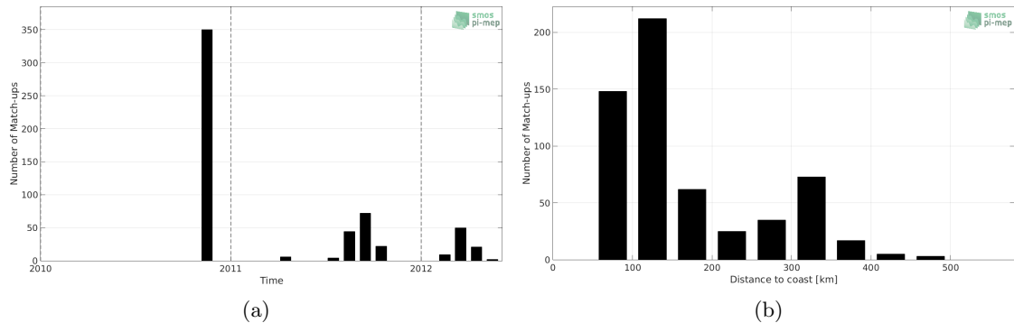
Figure 1: Number of match-ups between Surface drifters and SMOS-L4-CATDS-CECOS-IFREMER-V2-WEEKLY-0.5DEG SSS as a function of time (a) and as function of the distance to coast (b) over the Arctic Ocean Pi-MEP region and for the full satellite product period.
