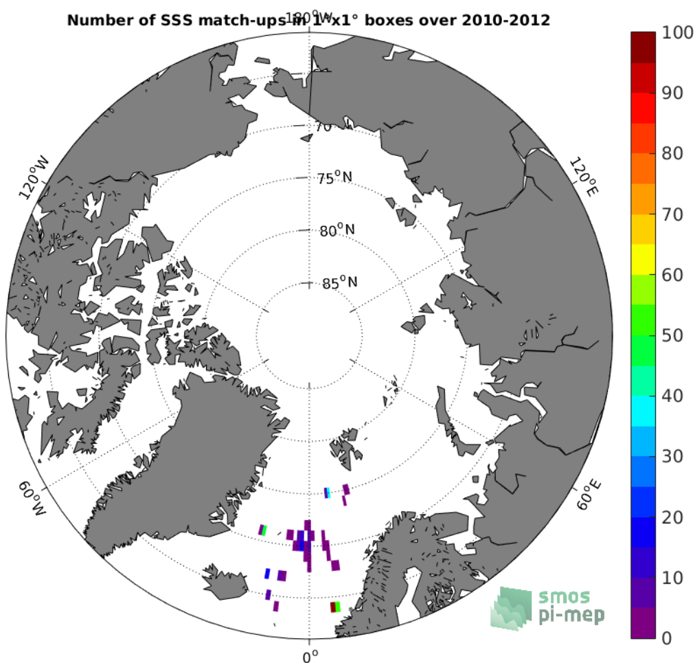
Figure 3: Number of SSS match-ups between Surface drifters SSS and the SMOS-L4-CATDS-CECOS-IFREMER-V2-WEEKLY-0.5DEG SSS product for the Arctic Ocean Pi-MEP region over 1^\circ \times 1^\circ boxes and for the full satellite product period.
