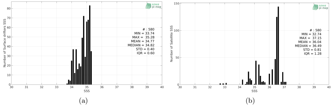
Figure 2: Histograms of SSS from Surface drifters (a) and SMOS-L4-CATDS-CECOS-IFREMER-V2-WEEKLY-0.5DEG (b) considering all match-up pairs per bins of 0.1 over the Arctic Ocean Pi-MEP region and for the full satellite product period.
