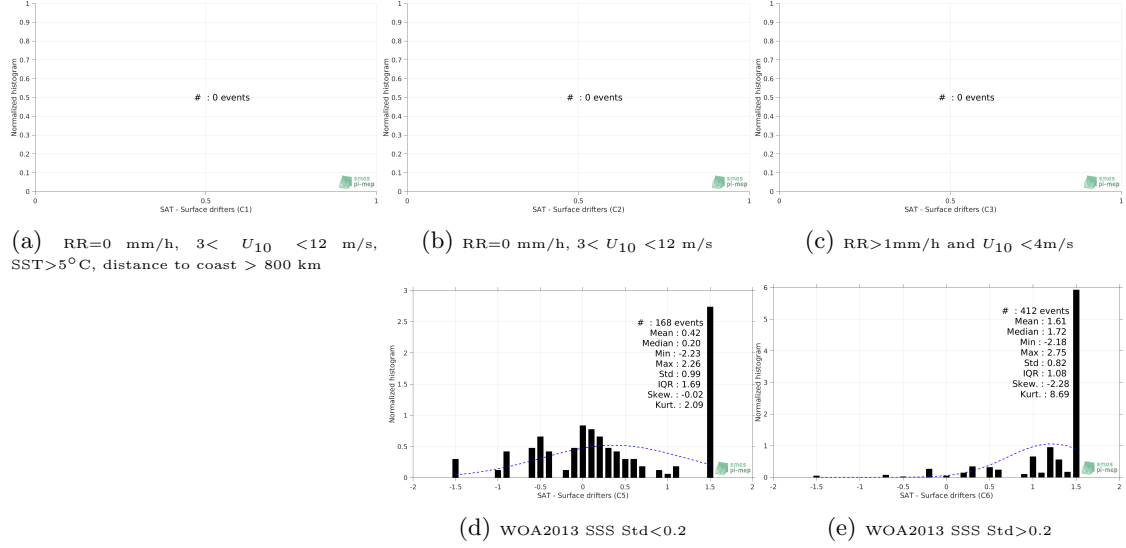
Figure 12: Normalized histogram of \Delta\text{SSS} (SMOS-L4-CATDS-CECOS-IFREMER-V2-WEEKLY-0.5DEG - Surface drifters) for 5 different subdatasets corresponding to: RR=0 mm/h, 3 < U_{10} < 12 m/s, SST > 5^\circ\text{C} , distance to coast > 800 km (a), RR=0 mm/h, 3 < U_{10} < 12 m/s (b), RR > 1\text{mm/h} and U_{10} < 4\text{m/s} (c), WOA2013 SSS Std < 0.2 (d), WOA2013 SSS Std > 0.2 (e).
