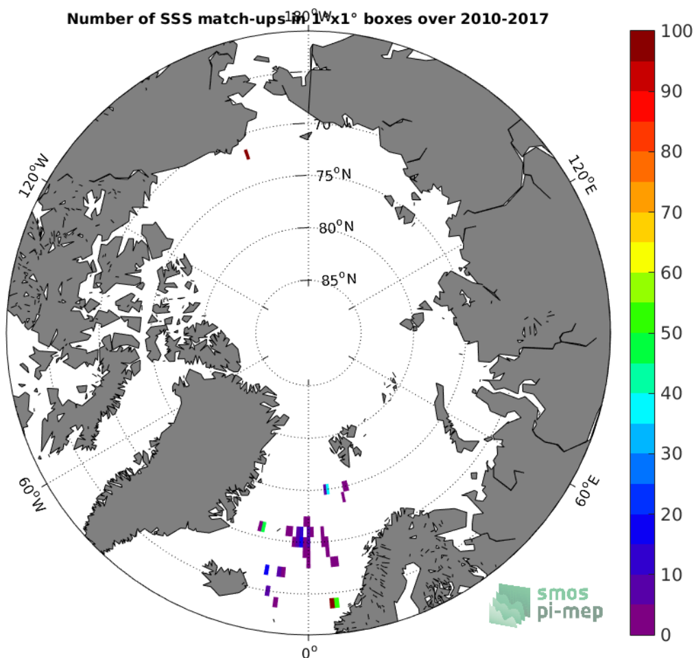
Figure 3: Number of SSS match-ups between Surface drifters SSS and the SMOS-L4-CATDS-CECOS-IFREMER-V2-WEEKLY-0.5DEG SSS product for the Arctic Ocean Pi-MEP region over 1°x1° boxes and for the full satellite product period.
