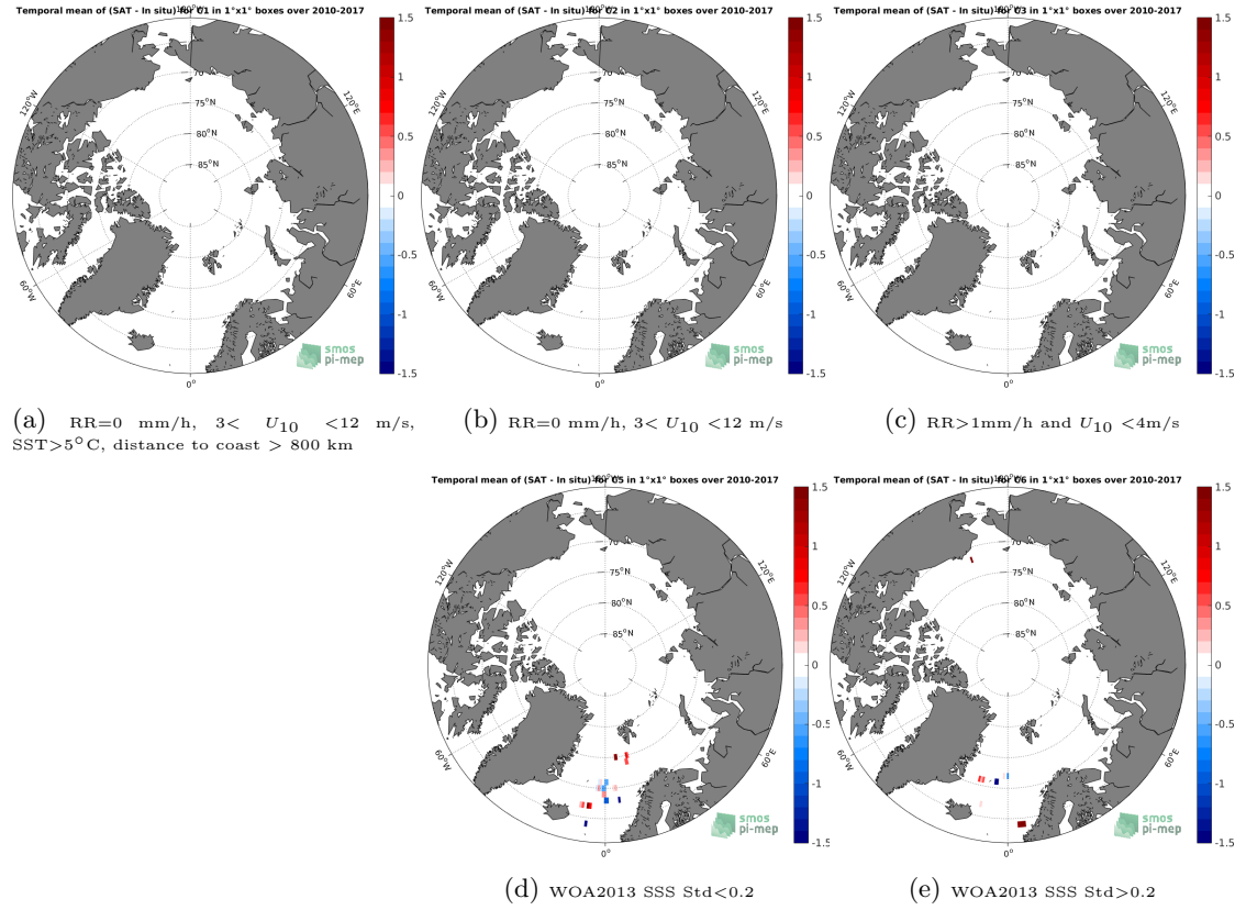
Figure 11: Temporal mean gridded over spatial boxes of size 1^\circ \times 1^\circ of \Delta SSS (SMOS-L4-CATDS-CECOS-IFREMER-V2-WEEKLY-0.5DEG - Surface drifters) for 5 different subdatasets corresponding to: RR=0 mm/h, 3 < U_{10} < 12 m/s, SST > 5^\circ C , distance to coast > 800 km (a), RR=0 mm/h, 3 < U_{10} < 12 m/s (b), RR > 1 mm/h and U_{10} < 4 m/s (c), WOA2013 SSS Std < 0.2 (d), WOA2013 SSS Std > 0.2 (e).
