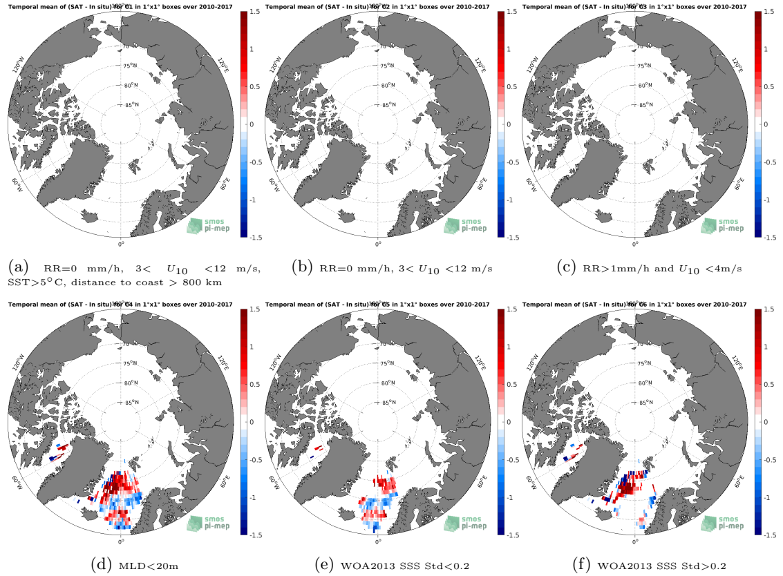
Figure 12: Temporal mean gridded over spatial boxes of size 1^{\circ}\times 1^{\circ} of \Delta\text{SSS} (SMOS L4 v2 Weekly (CATDS-CECOS-IFREMER) - Argo) for 6 different subdatasets corresponding to:RR=0 mm/h, 3 < U_{10} < 12 m/s, SST >5^{\circ}\text{C} , distance to coast > 800 km (a), RR=0 mm/h, 3 < U_{10} < 12 m/s (b), RR >1\text{mm/h} and U_{10} < 4\text{m/s} (c),MLD <20\text{m} (d),WOA2013 SSS Std <0.2 (e),WOA2013 SSS Std >0.2 (f).
