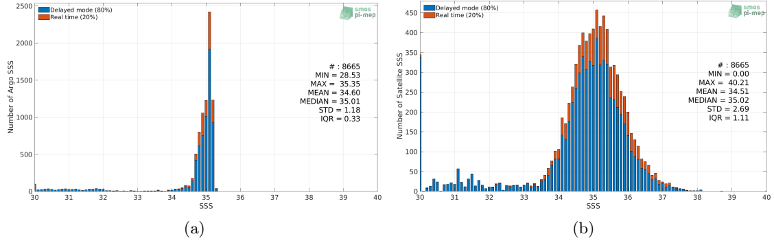
Figure 2: Histograms of SSS from Argo (a) and SMOS L4 v2 Weekly (CATDS-CECOS-IFREMER) (b) considering all match-up pairs per bins of 0.1 over the Arctic Ocean Pi-MEP region and for the full satellite product period.
