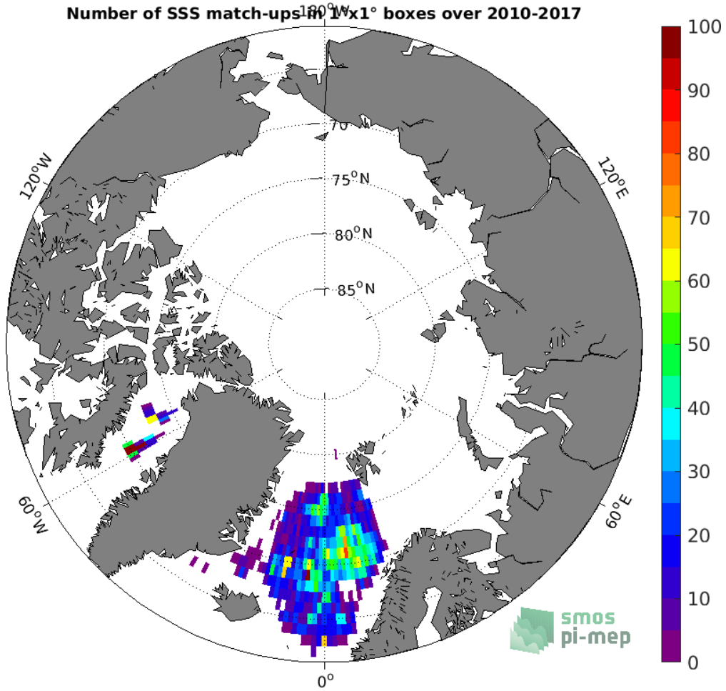
Figure 4: Number of SSS match-ups between Argo SSS and the SMOS L4 v2 Weekly (CATDS-CECOS-IFREMER) SSS product for the Arctic Ocean Pi-MEP region over 1^\circ \times 1^\circ boxes and for the full satellite product period.
