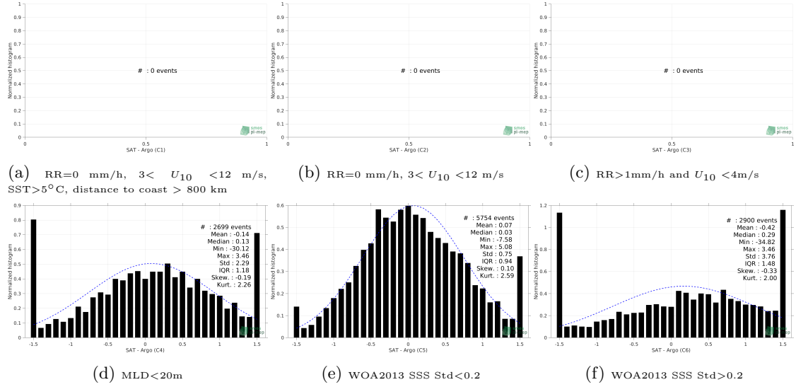
Figure 13: Normalized histogram of \Delta\text{SSS} (SMOS L4 v2 Weekly (CATDS-CECOS-IFREMER) - Argo) for 6 different subdatasets corresponding to: RR=0 mm/h, 3 < U_{10} < 12 m/s, SST > 5^\circ\text{C} , distance to coast > 800 km (a), RR=0 mm/h, 3 < U_{10} < 12 m/s (b), RR > 1\text{mm/h} and U_{10} < 4\text{m/s} (c), MLD < 20\text{m} (d), WOA2013 SSS Std < 0.2 (e), WOA2013 SSS Std > 0.2 (f).
