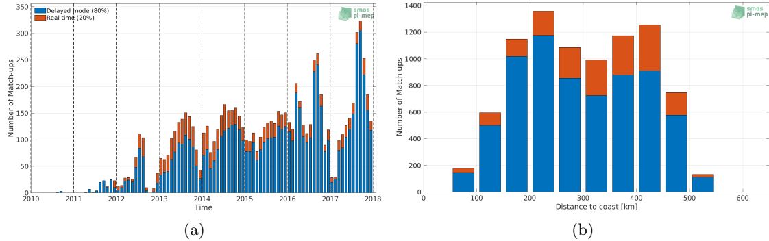
Figure 1: Number of match-ups between Argo and SMOS L4 v2 Weekly (CATDS-CECOS-IFREMER) SSS as a function of time (a) and as function of the distance to coast (b) over the Arctic Ocean Pi-MEP region and for the full satellite product period.
