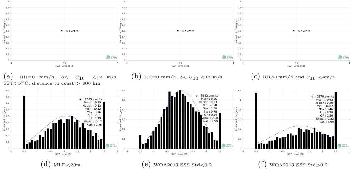
Figure 13: Normalized histogram of \Delta SSS (SMOS L4 v2 Weekly (CATDS-CECOS-IFREMER) - Argo) for 6 different subdatasets corresponding to: RR=0 mm/h, 3 < U_{10} < 12 m/s, SST > 5°C, distance to coast > 800 km (a), RR=0 mm/h, 3 < U_{10} < 12 m/s (b), RR > 1mm/h and U_{10} < 4 m/s (c), MLD < 20m (d), WOA2013 SSS Std < 0.2 (e), WOA2013 SSS Std > 0.2 (f).
