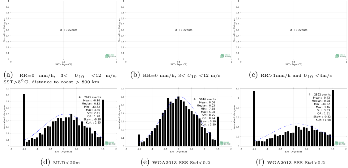
Figure 13: Normalized histogram of \Delta\text{SSS} (SMOS-L4-CATDS-CECOS-IFREMER-V2-WEEKLY-0.5DEG - Argo) for 6 different subdatasets corresponding to: RR=0 mm/h, 3 < U_{10} < 12 m/s, SST > 5^\circ\text{C} , distance to coast > 800 km (a), RR=0 mm/h, 3 < U_{10} < 12 m/s (b), RR > 1\text{mm/h} and U_{10} < 4\text{m/s} (c), MLD < 20\text{m} (d), WOA2013 SSS Std < 0.2 (e), WOA2013 SSS Std > 0.2 (f).
