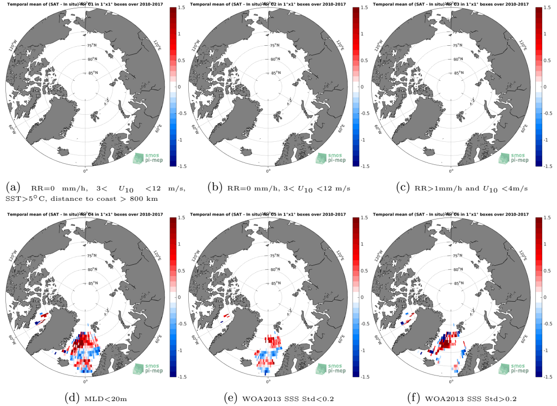
Figure 12: Temporal mean gridded over spatial boxes of size 1^{\circ}\times 1^{\circ} of \Delta\text{SSS} (SMOS-L4-CATDS-CECOS-IFREMER-V2-WEEKLY-0.5DEG - Argo) for 6 different subdatasets corresponding to:RR=0 mm/h, 3 < U_{10} < 12 m/s, SST >5^{\circ}\text{C} , distance to coast > 800 km (a), RR=0 mm/h, 3 < U_{10} < 12 m/s (b), RR >1 mm/h and U_{10} < 4 m/s (c),MLD <20 m (d),WOA2013 SSS Std <0.2 (e),WOA2013 SSS Std >0.2 (f).
