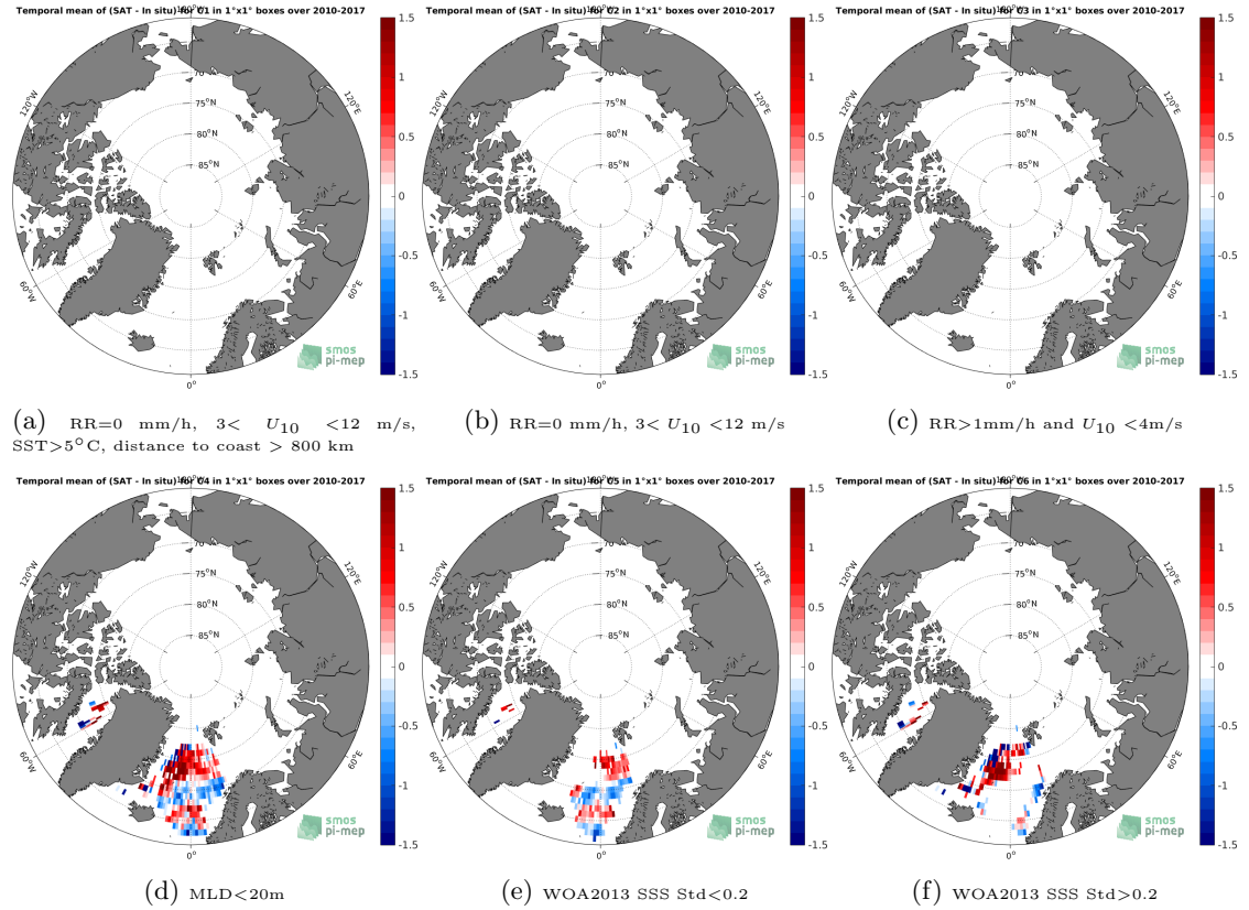
Figure 12: Temporal mean gridded over spatial boxes of size 1^\circ \times 1^\circ of \Delta SSS (SMOS-L4-CATDS-CECOS-IFREMER-V2-WEEKLY-0.5DEG - Argo) for 6 different subdatasets corresponding to: RR=0 mm/h, 3 < U_{10} < 12 m/s, SST > 5^\circ C , distance to coast > 800 km (a), RR=0 mm/h, 3 < U_{10} < 12 m/s (b), RR > 1 mm/h and U_{10} < 4 m/s (c), MLD < 20 m (d), WOA2013 SSS Std < 0.2 (e), WOA2013 SSS Std > 0.2 (f).
