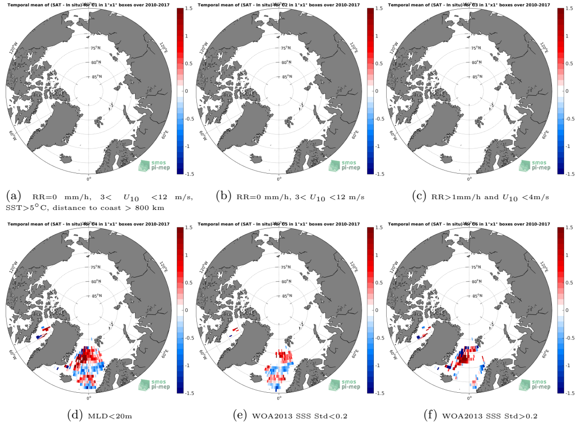
Figure 12: Temporal mean gridded over spatial boxes of size 1^\circ \times 1^\circ of \Delta SSS (SMOS-L4-CATDS-CECOS-IFREMER-V2-WEEKLY-0.5DEG - Argo) for 6 different subdatasets corresponding to:RR=0 mm/h, 3 < U_{10} < 12 m/s, SST >5^\circ\text{C} , distance to coast > 800 km (a), RR=0 mm/h, 3 < U_{10} < 12 m/s (b), RR >1 mm/h and U_{10} < 4 m/s (c),MLD <20 m (d),WOA2013 SSS Std <0.2 (e),WOA2013 SSS Std >0.2 (f).
