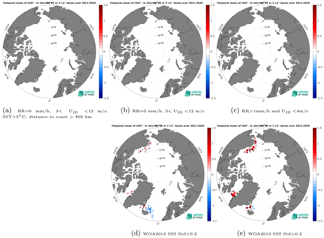
Figure 12: Temporal mean gridded over spatial boxes of size 1^{\circ}\times 1^{\circ} of \Delta\text{SSS} (SMOS SSS L4 v2 - Daily (BEC) - TSG (SAMOS)) for 5 different subdatasets corresponding to:RR=0 mm/h, 3 < U_{10} < 12 m/s, SST > 5^{\circ}\text{C} , distance to coast > 800 km (a), RR=0 mm/h, 3 < U_{10} < 12 m/s (b), RR > 1 mm/h and U_{10} < 4 m/s (c), WOA2013 SSS Std < 0.2 (d), WOA2013 SSS Std > 0.2 (e).
