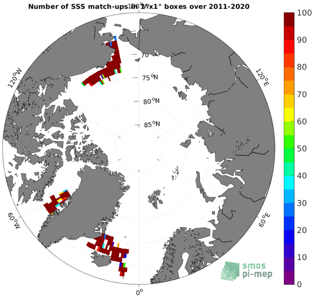
Figure 4: Number of SSS match-ups between TSG (SAMOS) SSS and the SMOS SSS L4 v2 - Daily (BEC) SSS product for the Arctic Ocean Pi-MEP region over 1^{\circ} \times 1^{\circ} boxes and for the full satellite product period.
