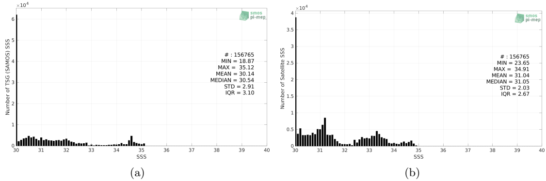
Figure 2: Histograms of SSS from TSG (SAMOS) (a) and SMOS SSS L4 v2 - Daily (BEC) (b) considering all match-up pairs per bins of 0.1 over the Arctic Ocean Pi-MEP region and for the full satellite product period.
