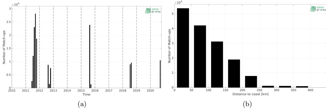
Figure 1: Number of match-ups between TSG (SAMOS) and SMOS SSS L4 v2 - Daily (BEC) SSS as a function of time (a) and as function of the distance to coast (b) over the Arctic Ocean Pi-MEP region and for the full satellite product period.
